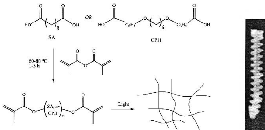
Figure 6 Synthesis of methacrylated anhydride oligomers for use in a photo-polymerizable polyanhydride system. (right) A degradable bone screw (length = 4 cm) produced in a mold from illuminating at the screw head only.
