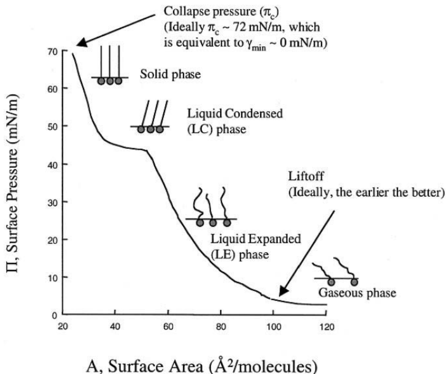
Figure 4 Surface pressure–area ( \Pi -A) isotherm of the compression of a hypothetical surfactant film that exhibits gaseous, liquid-expanded, liquid-condensed, and solid phases. As area decreases, the surface pressure increases until the film collapses. Typical lift-off and collapse pressure values of lung surfactant are depicted. (Adapted from Ref. 279, with permission.)
