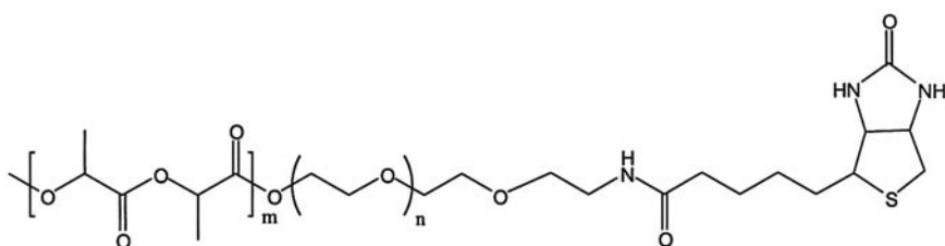
PLA-PEG-biotin
