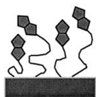
PLA-PEG-biotin
