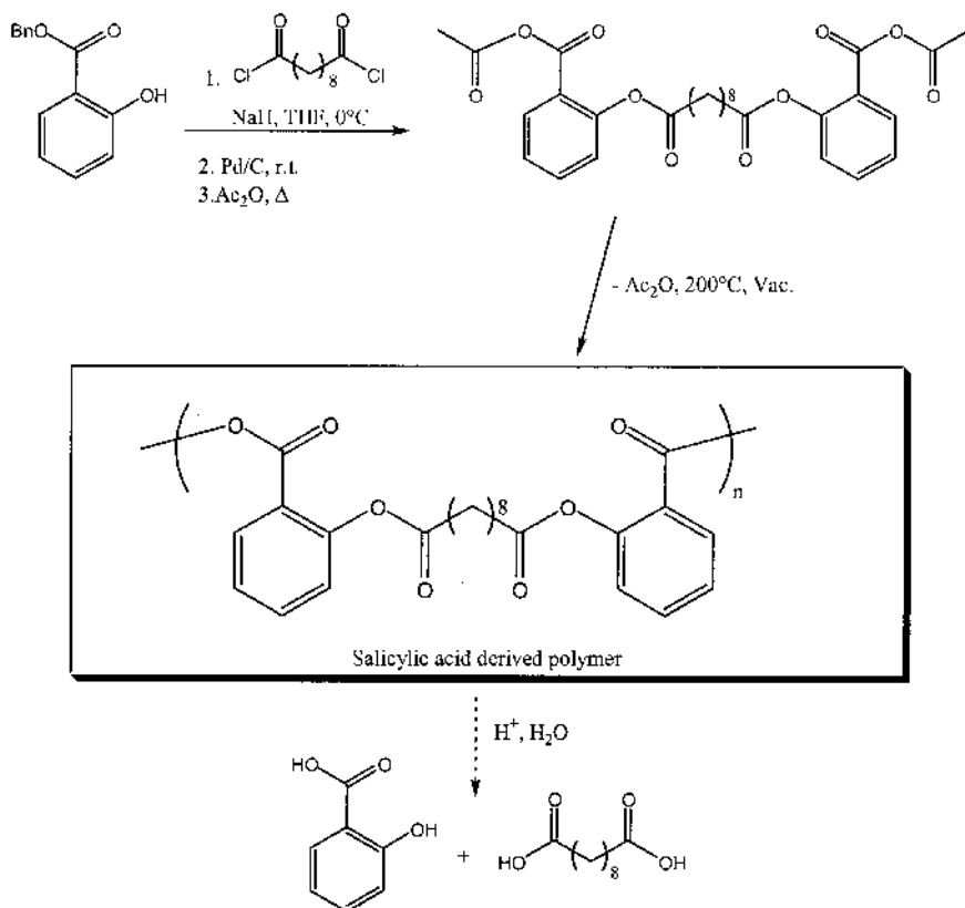
Figure 7 Synthesis of polyanhydride ester: PolyAspirin.
