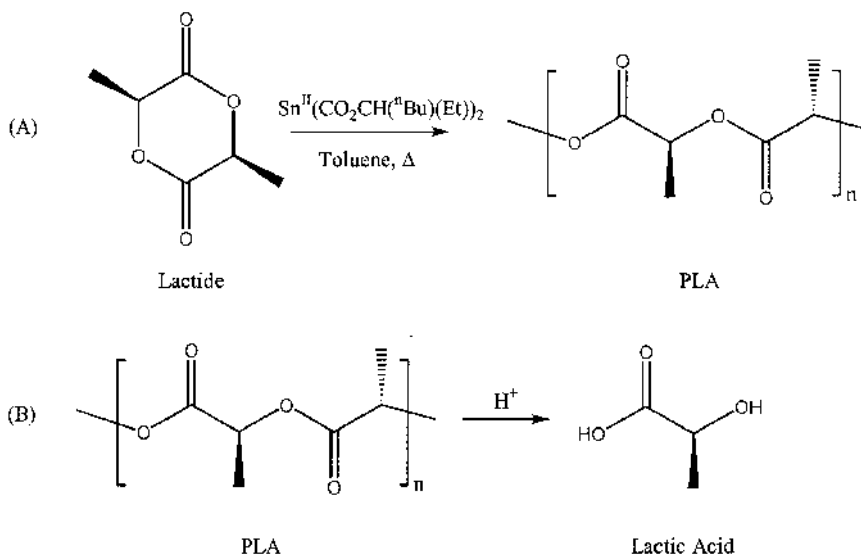
Figure 1 Synthesis and degradation of polylactic acid (PLA). (A) Polymer synthesis: ring-opening polymerization of lactide via stannous octoate to give PLA. (B) Polymer degradation: acid hydrolysis of PLA to give lactic acid.
