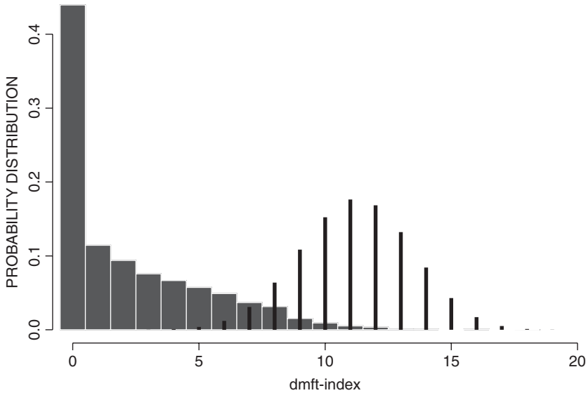
Figure 10.4 Comparison of Signal-Tandmobiel ® probability distribution of dmft-index (left histogram) to binomial distribution based 20 experiments with probability of success' = 0.55, i.e. \text{Bin}(20, 0.55) .
