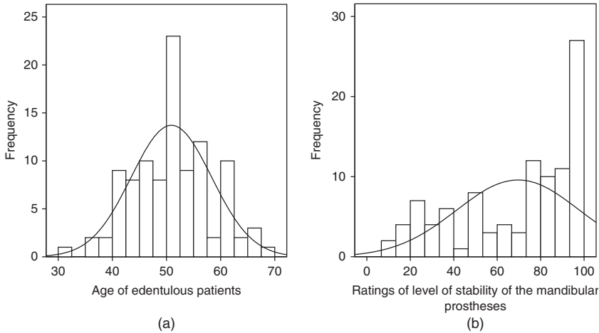
Figure 10.1 2-IO Study: shapes of distributions (displayed as histograms) and approximating normal curves. (a) symmetric and (b) negatively skewed.
