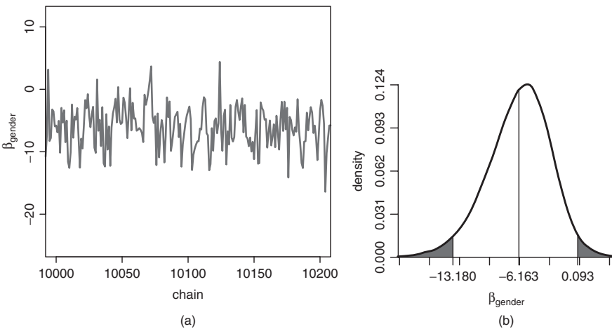
Figure 18.5 Smile for Life study: Trace plot (a) and graphical display of contour probability (b) for the regression coefficient associated to gender.
