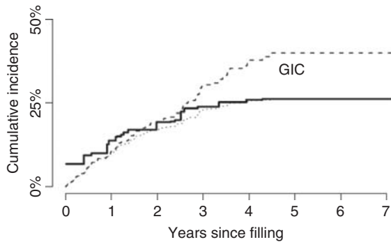
Figure 15.6 The cumulative incidence of filling fractures for the glass ionomer cement fillings. The solid line is obtained with the nonparametric maximum likelihood estimator for the competing risks model depicted in Figure 15.4. The dotted line is obtained with Aalen-Johansen estimator for the same model based on the interval midpoints and the dashed line is the Kaplan-Meier estimator based on the interval midpoints and treating competing risks as right censored.
