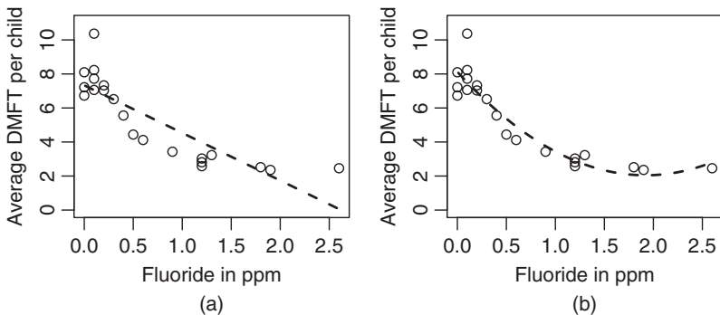
Figure 11.5 Fitted curves for the fluoride data based on (a) a model that is linear in fluoride concentration; and (b) a model that is quadratic in fluoride concentration.
