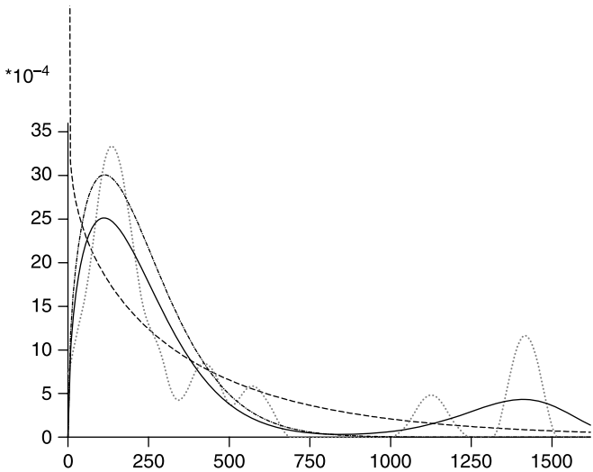
Figure 28.1 Kernel density estimate (dotted line), MLE Weibull fit (dashed line), MLE \alpha = 1 Weibull fit (dotted-dashed line), and MLE two-component mixture Weibull fit (solid line) for arm A of the Efron [18] data.
