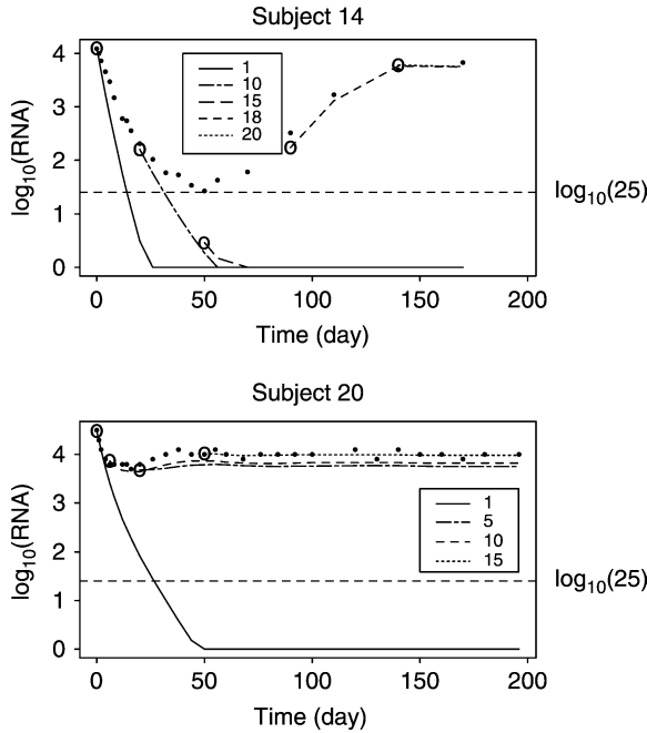
Figure 6.2 Generated viral load data in \log_{10} scale (solid circles) and individual prediction curves beginning at the point denoted by the circle for the two representative subjects. The values in the legend denote the number of viral load measurements used for predicting future virological responses. The HIV-1 RNA measurements below a limit of detection of 25 copies/mL are imputed by 25 copies/mL (dashed horizontal line).
