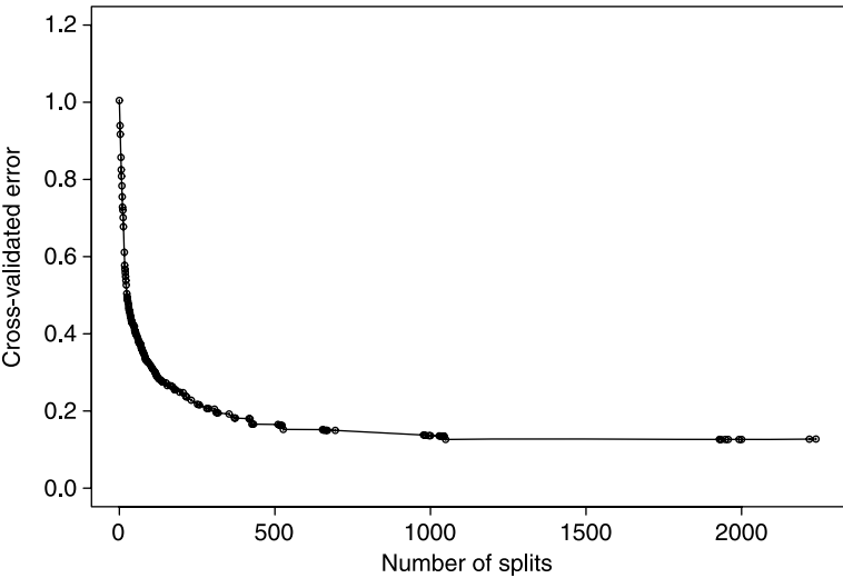
Figure 25.2 Cross-validated error profiles for classification trees grown to maximal size on the letter recognition data from mlbench.
