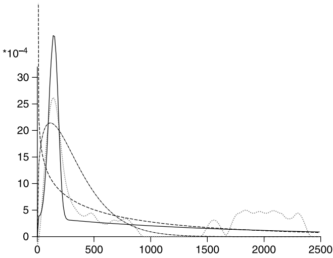
Figure 28.2 Kernel density estimate (dotted line), MLE Weibull fit (dashed line), MLE \alpha = 1 Weibull fit (dotted-dashed line), and MLE two-component mixture Weibull fit (solid line) for arm B of the Efron [18] data.
