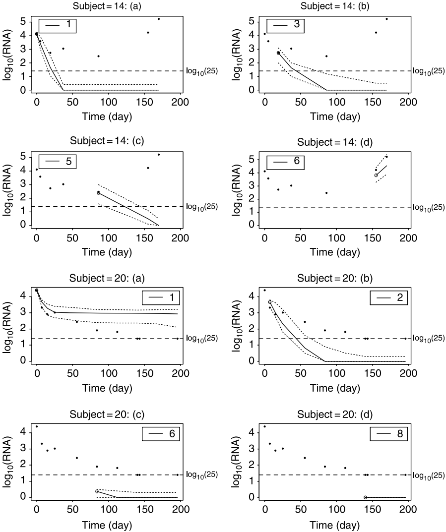
Figure 6.3 Observed viral load data in \log_{10} scale (solid circles) and individual prediction curves (solid) started at the point denoted by the circle as well as the corresponding 95% prediction credible intervals (dotted curves) for the two representative subjects. The values in the legend denote the number of viral load measurements used for predicting future virological responses. The HIV-1 RNA measurements below a limit of detection of 25 copies/mL are imputed by 25 copies/mL (dashed horizontal line).
