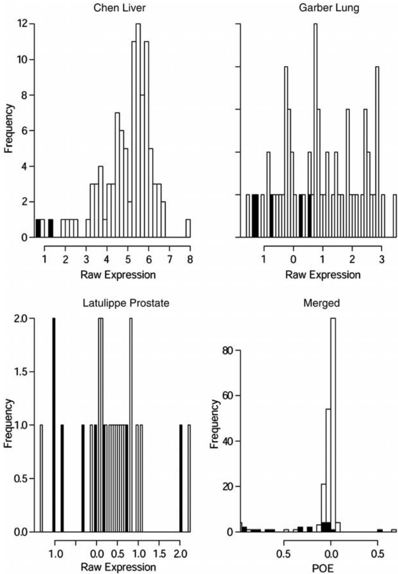
Figure 19.3 POE transformation of gene with Unigene cluster ID Hs.69771. This gene is the top-ranked gene in POEA signature. Unfilled and filled bars mark the expression of primary and metastatic tumors for this gene, respectively.
