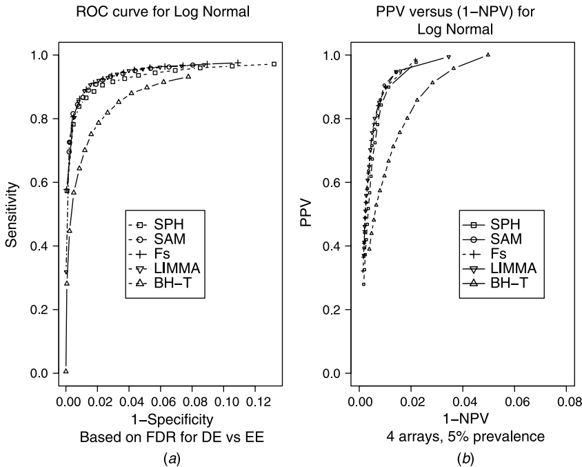
Figure 20.2 Performance evaluation of the five methods for controlling FDR, using ROC curves and predictive power curves for scenario 2 with 5% prevalence of DE genes.
