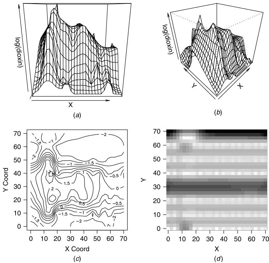
Figure 7.11 Kriged \log(\text{dioxin}) measurements: (a) mean of predictive distribution; (b) mean of predictive distribution; (c) mean of predictive distribution; (d) local variance of predictive distribution.
