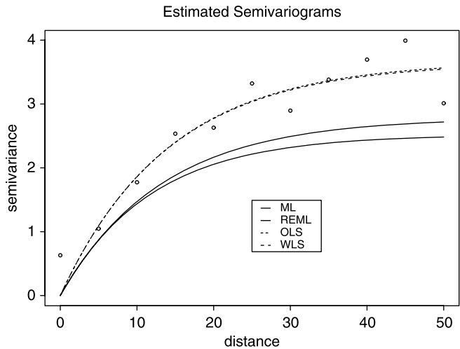
Figure 7.8 Semivariograms for dioxin measurements. The circles denote the empirical semivariogram and the lines denote the best-fitting exponential semivariogram under maximum likelihood (ML), restricted maximum likelihood (REML), ordinary least squares (OLS), and weighted least squares (WLS).
