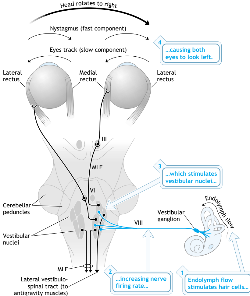
Figure 7-11. Vestibuloocular reflex. Abbreviation key: MLF, medial longitudinal fasciculus. Roman numerals indicate cranial nerves.
