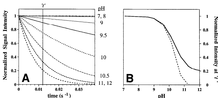
Fig. 2. Kinetic decay curves simulated at various pHs. (A) Simulations were performed using Eq. 10 and 140 s^{-1} and 20,000 s^{-1} and 1.9 \cdot 10^8 M^{-1}s^{-1} for k_{op} , k_{cl} , and k_b respectively. A vertical line is drawn at t_{ex} = 12 ms. (B) Simulated curves of the pH dependence of NH peak intensity at t_{ex} = 12 ms. The solid curve depicts a switch from EX2 to EX1 exchange at a very alkaline pH, while the dashed curve indicates the expected amplitudes for pure EX2 exchange.
