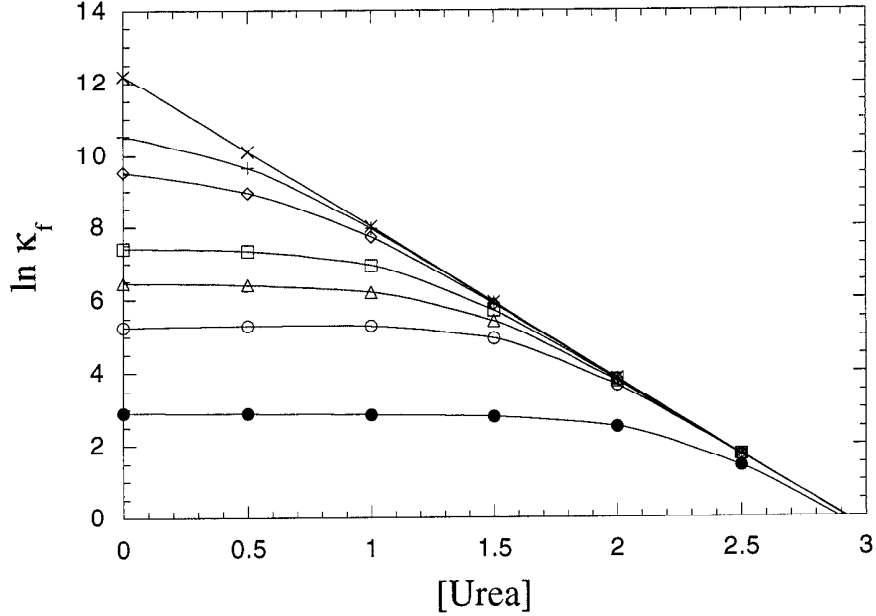
Fig. 5. Denaturant dependence of the stability constants for a subset of residues in SNase. Residues included are 9 ( open circle ), 10 ( open square ), 18 ( open diamonds ), 38 ( \times ), 39 ( + ), 40 ( open triangle ), and 41 ( closed circle ). The denaturant independent slope at low concentrations of urea occurs despite the significant surface area exposed (9% of structure unfolded). Modeling the denaturant unfolding of SNase was facilitated through a denaturant binding model based on parameters derived from (32).
