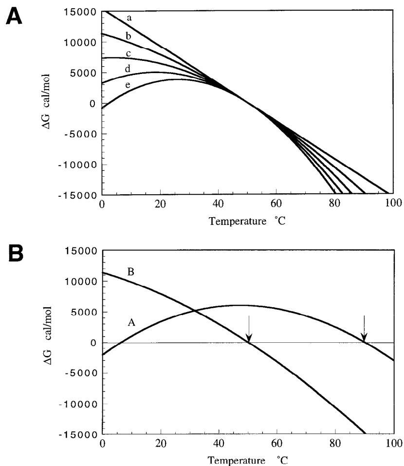
Fig. 1. (A) The temperature dependence of the Gibbs energy for different values of the heat-capacity change. In all cases, \Delta G is zero at 50 ^{\circ}\text{C} with an enthalpy change of 100 kcal/mol. The curves correspond to \Delta C_p values of: a) zero, b) 1000, c) 2000, d) 3000, and e) 4000 cal/K \cdot mol. (B) The temperature dependence of two hypothetical proteins is presented. Although protein A has a higher temperature stability than protein B, protein B is more stable at low temperatures. This example demonstrates that protein stability measured at room temperature (e.g., by urea or GuHCl denaturation) cannot be used as a predictor of high temperature stability.
