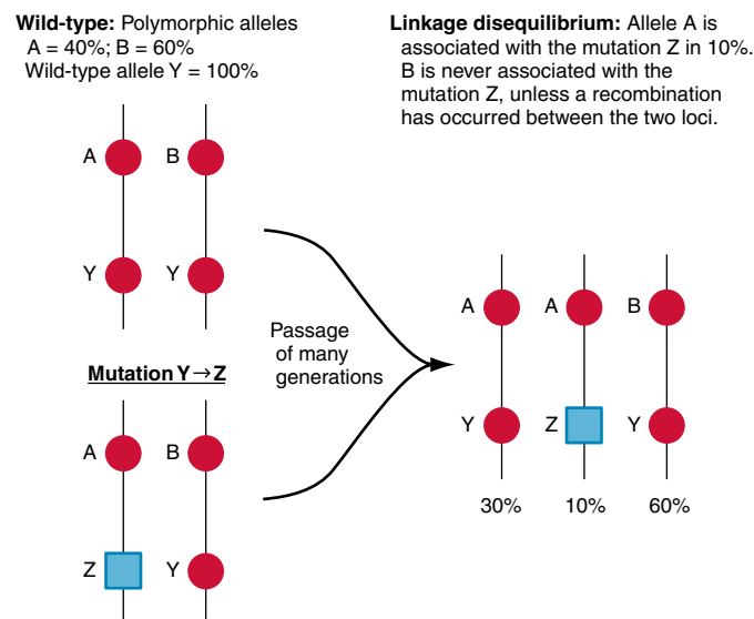
FIGURE 56-13 Linkage disequilibrium.
