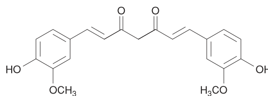
▲ FIGURE 34-3 Curcumin.
