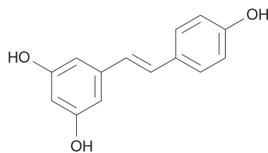
▲ FIGURE 34-8 Resveratrol.
