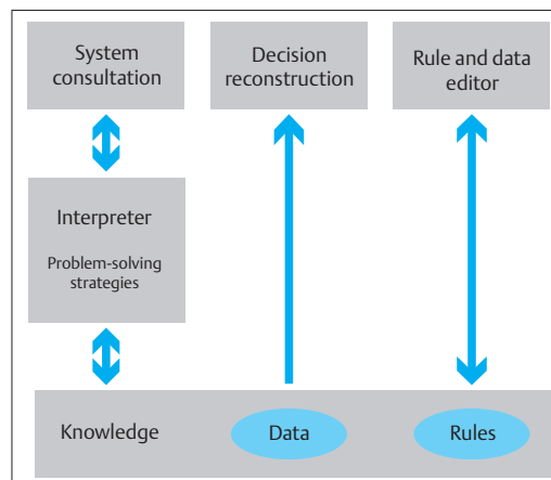
Fig. 5.2 Structure of an expert system.
