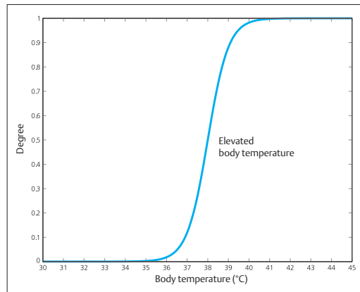
Fig. 5.3 Example of a fuzzy set.
