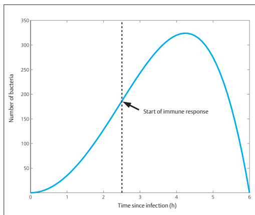
Fig. 5.1 Model for bacterial growth following an infection.
