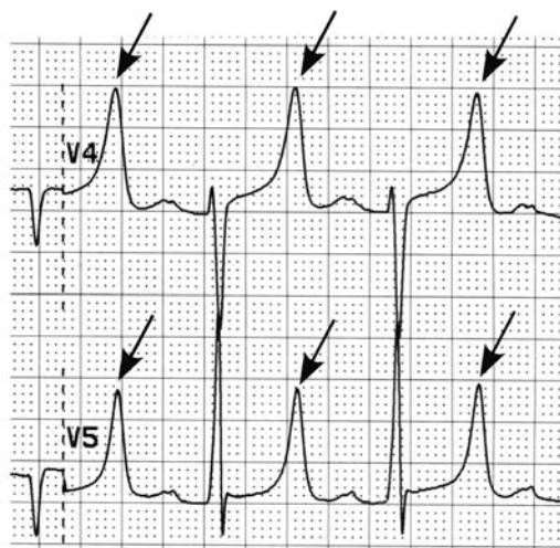
FIGURE 6-4. Peaked T waves in hyperkalemia.
