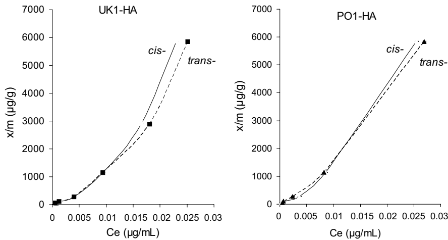
Figure 5. Freundlich (S-type) adsorption isotherms of cis - and trans -chlordane onto the HA examined
