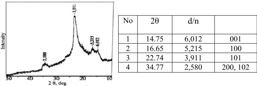
Figure 8. X-ray diffraction patterns of color transparent threads of carbon
