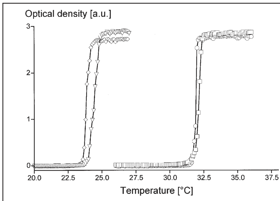
Figure 3.4. Thermoprecipitation curves of a) □ the nonconjugated AML-precursor and ○ the AML in pure water, b) ▽ only the AML in binding buffer, c) ◊ the affinity complex (AMLproduct) (reproduced with permission from reference 25).
