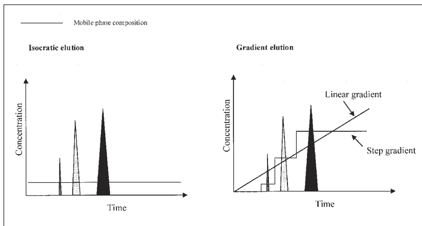
Figure 4.1. Schematic presentation of a separation by (gradient) elution chromatography.
