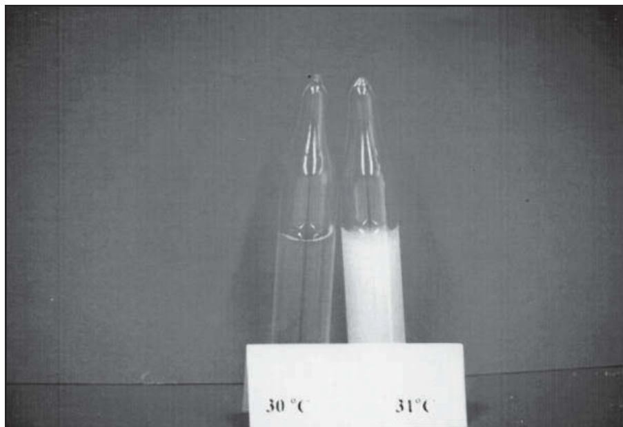
Figure 4.5. Thermosensitive displacer having a lower critical solution temperature between 30°C and 31°C.
