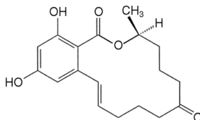
Fig. 25.6 The molecular structure of zearalenone.
