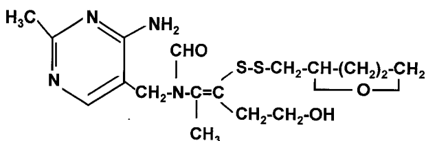
Thiamine tetrahydrofurfuryl disulfide
