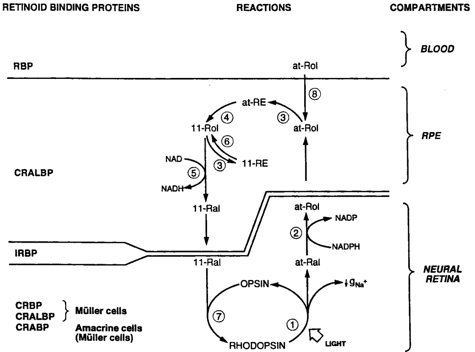
Fig. 8 Reactions of the mammalian visual cycle. Horizontal lines separate cellular and extracellular compartments in the retina involved in retinoid metabolism. Most of the enzymatic reactions of the cycle occur in RPE, including the generation of 11- cis retinol. The reactions shown below the double line occur within the photoreceptor cell. Retinoid-binding proteins found within the indicated compartments are shown on the left. CRALBP, cellular retinaldehyde-binding protein; CRBP, cellular retinol-binding protein; IRBP, interphotoreceptor retinoid-binding protein; RBP, retinol-binding protein; at-, all- trans -; 11-, 11- cis -; Rol, retinol; Ral, retinaldehyde; RE, retinyl ester; g_{Na^+} , sodium conductance; RPE, retinal pigment epithelium. Reactions shown are: 1, photoisomerization; 2, all- trans retinol dehydrogenase; 3, lecithin:retinol acyltransferase (LRAT); 4, retinyl ester isomerohydrolase; 5, 11- cis retinol dehydrogenase; 6, retinyl ester hydrolase; 7, regeneration of rhodopsin (nonenzymatic); 8, uptake of plasma retinol. (From Ref. 68.)
