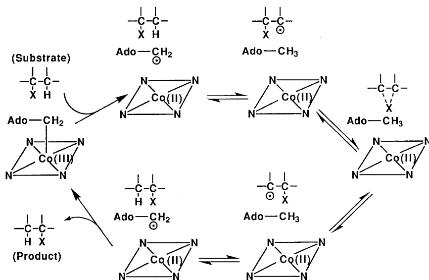
Fig. 13 Radical intermediates in vicinal rearrangements catalyzed by enzymes utilizing 5'-deoxyadenosyl-B 12 .
