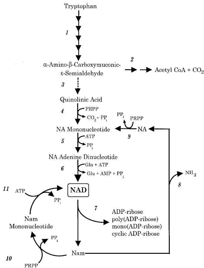
Fig. 3 Pathways of NAD + synthesis in mammals. Reactions 9, 5, and 6 comprise the Preiss-Handler pathway, while reactions 10 and 11 form the Dietrich pathway. The following enzymes correspond to the numbered reactions: (1) 5 step conversion; (2) picolinic carboxylase; (3) spontaneous chemical reaction; (4) quinolinic acid phosphoribosyltransferase; (5) NAMN adenylyltransferase (enzymes 5 and 11 may be identical proteins); (6) NAD synthetase; (7) NAD glycohydrolases, various ADP-ribosylation reactions; (8) nicotinamide deamidase; (9) nicotinic acid phosphoribosyltransferase; (10) nicotinamide phosphoribosyltransferase; (11) NMN adenylyltransferase.
