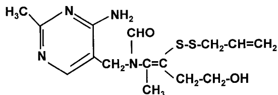
Thiamine allyl disulfide
