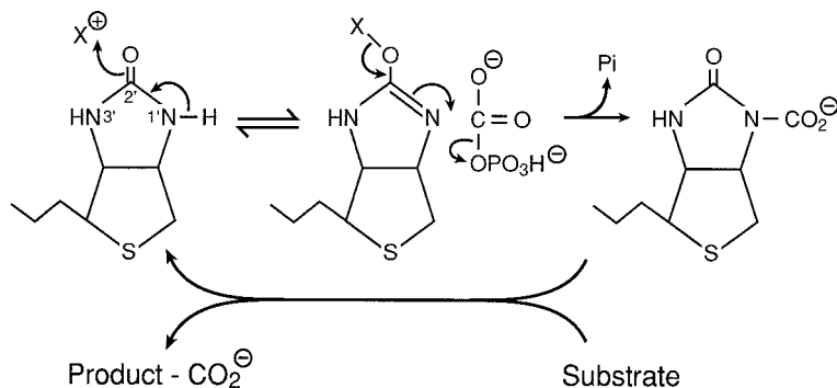
Fig. 9 Function of the biotinyl moiety within enzymes involved in carboxylations with the intermediacy of the putative carbonyl phosphate.
