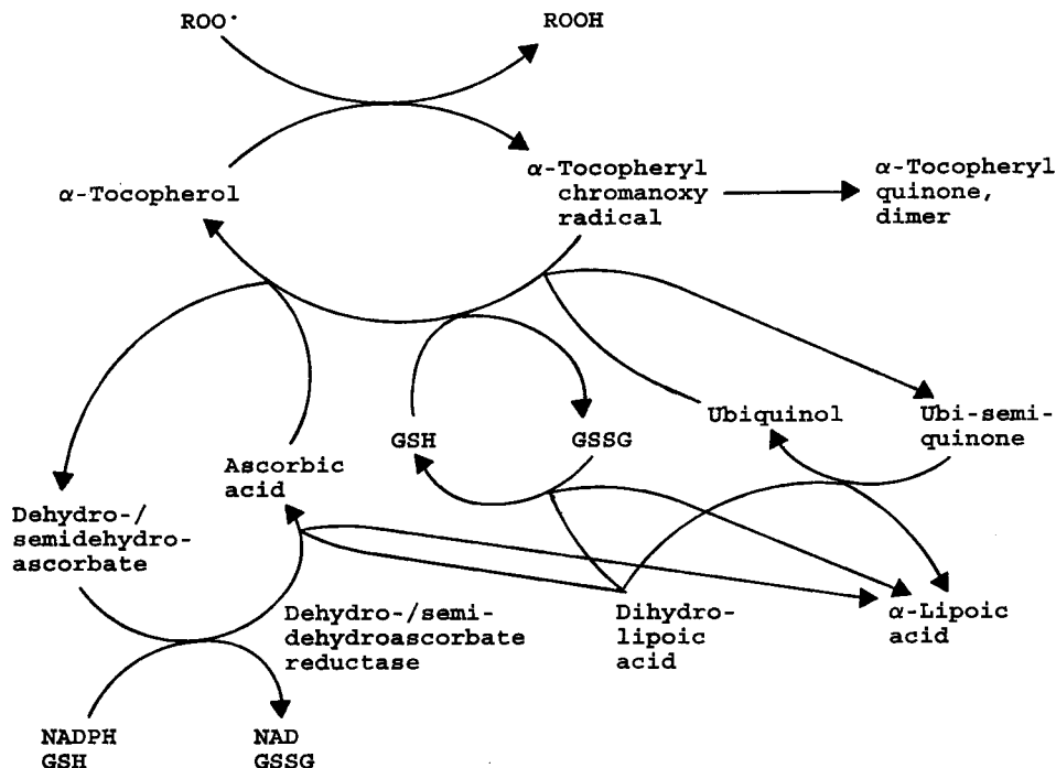
Fig. 4 Possible regeneration pathways of \alpha -tocopherol. LOOH represents lipid hydroperoxides; LOO', peroxy radical; GSH, reduced glutathione; GSSG, oxidized glutathione; NADH and NAD, reduced and oxidized nicotinamide adenine dinucleotide, respectively; NADPH and NADP, reduced and oxidized nicotinamide dinucleotide phosphate, respectively.
