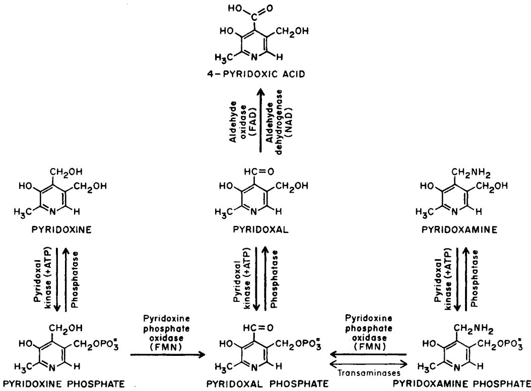
Fig. 4 Metabolic interconversions of the B 6 vitamers.
