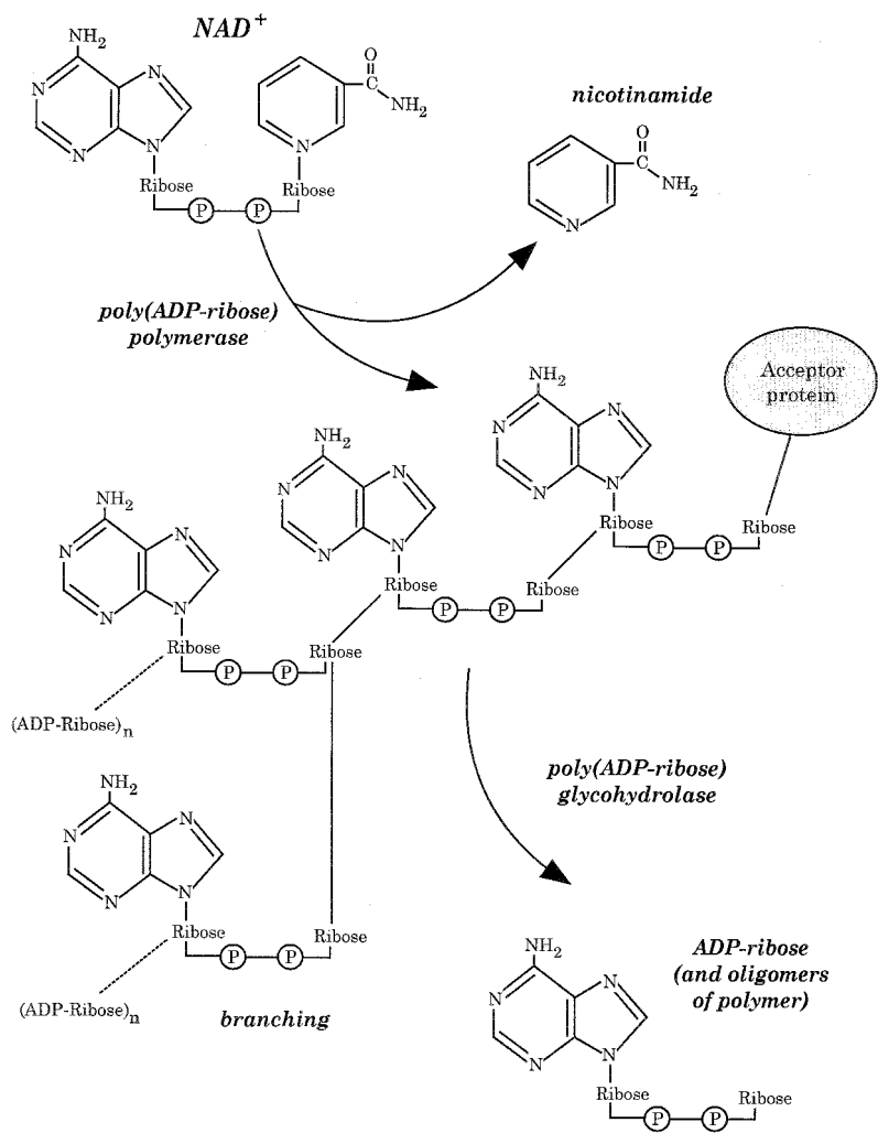
Fig. 5 Synthesis and degradation of poly(ADP-ribose).
