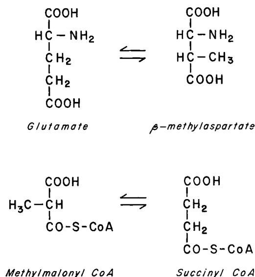
Fig. 5 Glutamate mutase, the first enzyme shown to require AdoCbl as coenzyme. It is here compared with methylmalonyl CoA mutase.
