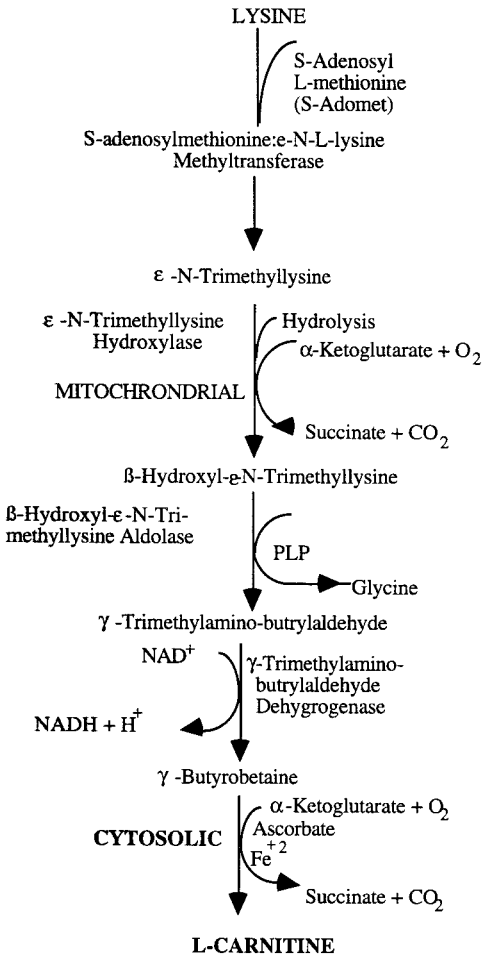
Fig. 3 Carnitine metabolic pathway. CO 2 , carbon dioxide; O 2 , oxygen; NAD + (NADH), nicotinamide dehydrogenase; Fe +2 , ferrous iron; PLP, pyridoxyl phosphate.
