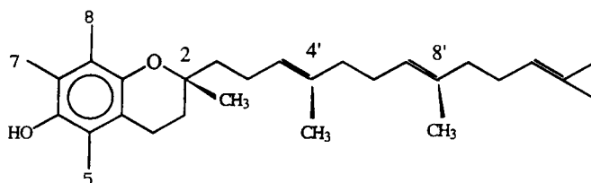
Tocotrienol Structure
