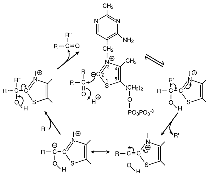
Fig. 5 Function of the thiazole moiety of thiamine pyrophosphate. In \alpha -keto acid decarboxylations, R' is a carboxylate lost as \text{CO}_2 and R'' is a proton generating an aldehyde. In ketolations (both trans- and phospho-), R and R' are part of a ketose phosphate generating a bound glycoaldehyde intermediate and R'' is an aldose phosphate or inorganic phosphate generating a different ketose phosphate or acetyl phosphate, respectively.
