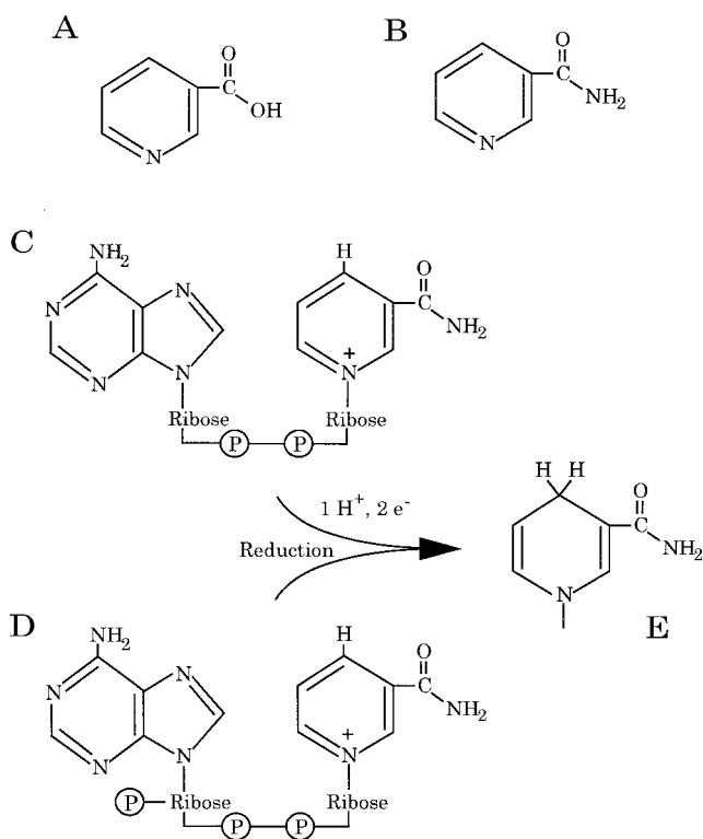
Fig. 2 Chemical structures of niacin compounds. (A) Nicotinic acid; (B) nicotinamide; (C) NAD + ; (D) NADP + ; (E) site of reduction.
