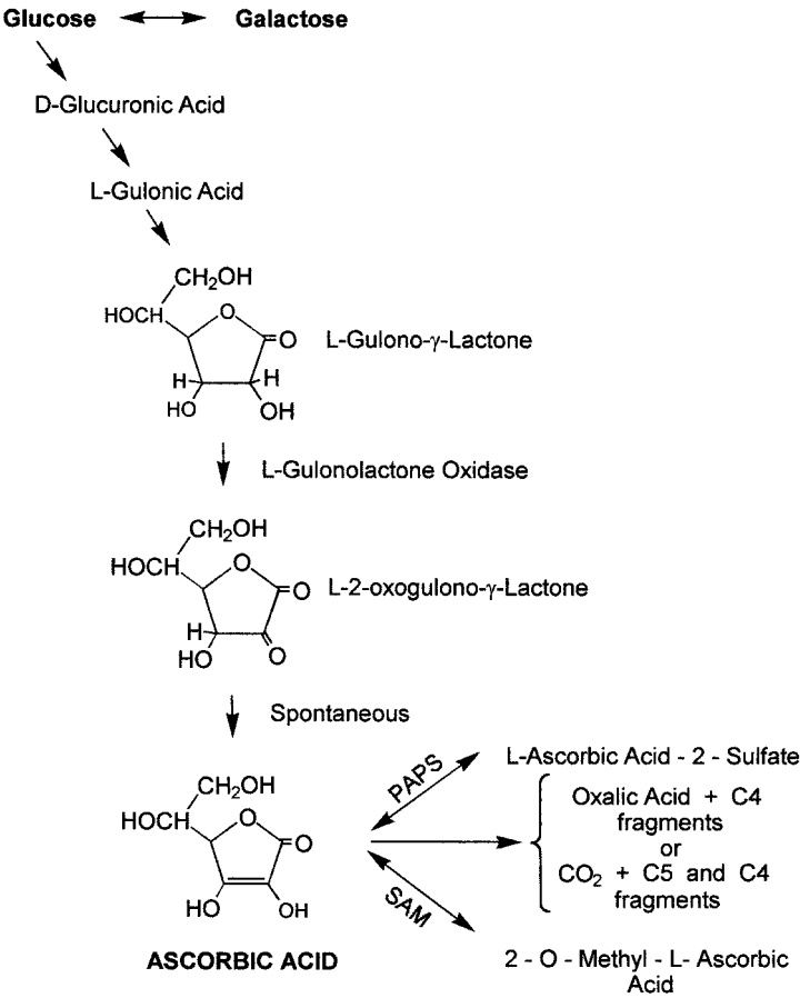
Fig. 3 Pathway for ascorbic acid synthesis from glucose in animal cells and examples of common adducts and degradation products.
