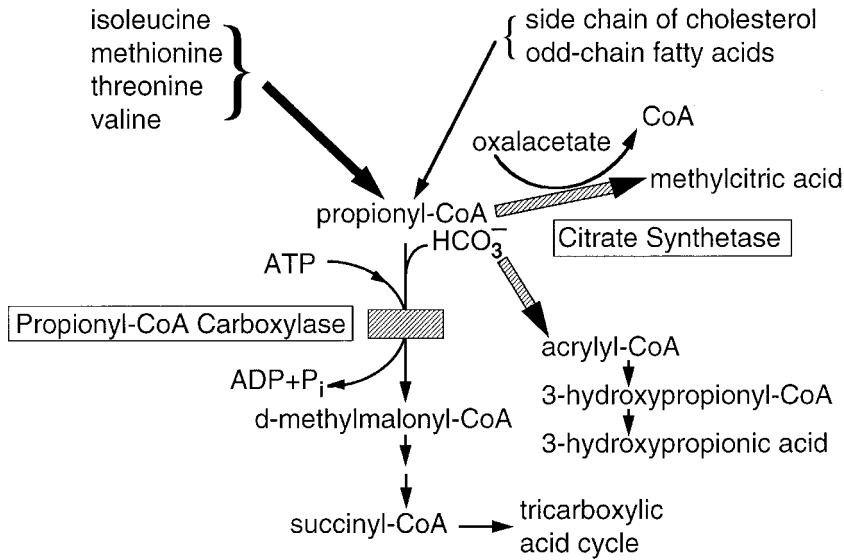
Fig. 4 Propionate metabolism. Propionate is derived primarily from amino acid degradation and to a lesser extent from cholesterol and odd-chain fatty acids, a deficiency [hatched box] of PCC causes increased urinary excretion of methylcitric and 3-hydroxypropionic acids. Abbreviations as in Fig. 1–3.
