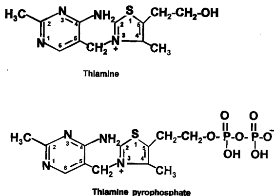
Fig. 1 Structural formulas of thiamine and thiamine pyrophosphate.
