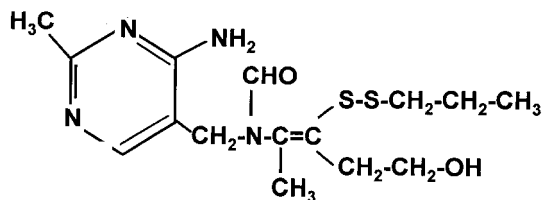
Thiamine propyl disulfide
