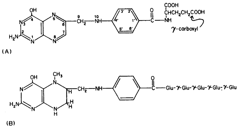
Fig. 1 Structure of (A) folic acid (PteGlu) and (B) 5-methyl-tetrahydrofolate pentaglutamate (5-Methyl- H_4 PteGlu _5 ). Although folic acid is not naturally occurring, it is readily transported and reduced to the natural forms of the vitamin. One-carbon substituents can be at the N-5 and/or N-10 positions of the reduced folate molecule.
