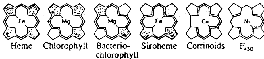
Fig. 2 Cyclic tetrapyrroles with biological functions. Stippled areas show double bonds and resonating conjugated bond systems. (From Ref. 32.)
