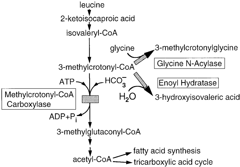
Fig. 3 Leucine degradation. A deficiency [hatched box] of MCC causes increased urinary excretion of 3-methylcrotonylglycine and 3-hydroxyisovaleric acid. Abbreviations as in Fig. 1 and 2.
