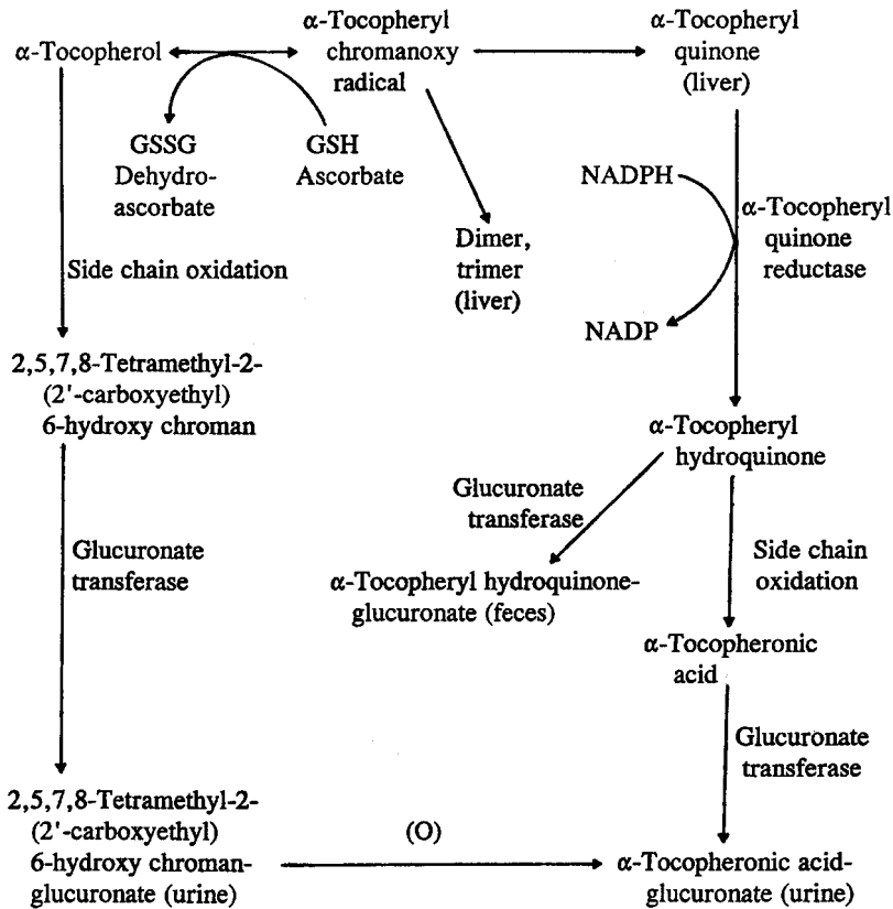
Fig. 2 Metabolic fate of α-tocopherol. GSH represents reduced glutathione; GSSG, oxidized glutathione; NADPH and NADP, reduced and oxidized nicotinamide dinucleotide phosphate, respectively.
