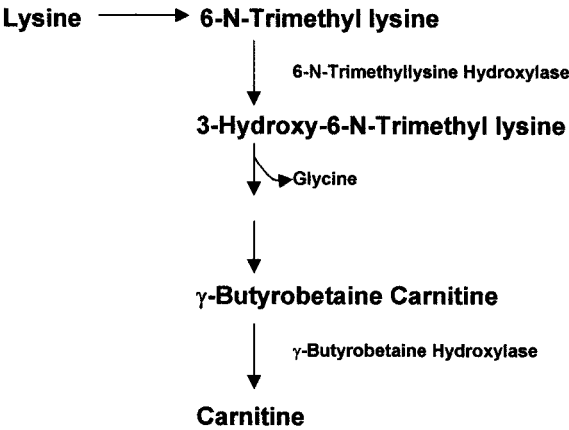
Fig. 6 Steps in carnitine biosynthesis.
