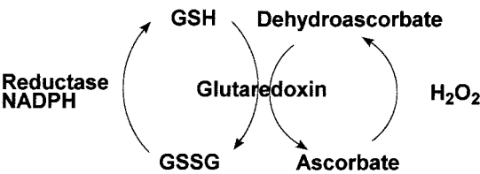
Fig. 4 Interaction between ascorbic acid and glutathione in its reduced (GSH and oxidized) forms (GSSG).
