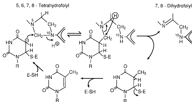
Fig. 12 The 1,3 hydrogen shift and redox nature of 5,10-methylene-tetrahydrofolyl coenzyme within thymidylate synthase.
