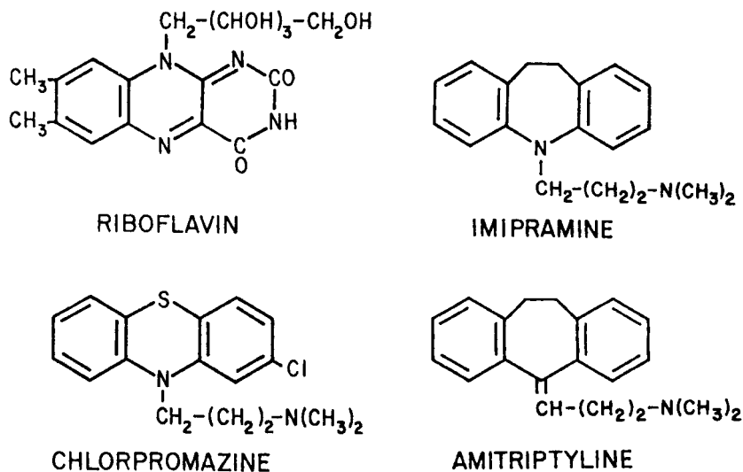
Fig. 4 Structural similarities among riboflavin, imipramine, chlorpromazine, and amitriptyline.
