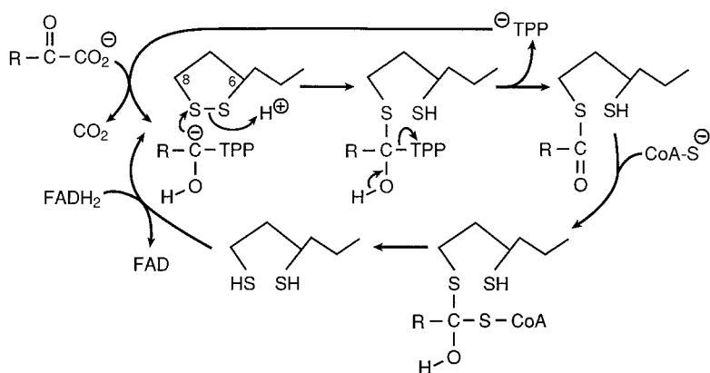
Fig. 8 Function of the lipoyl moiety within enzymes involved in transacylations following \alpha -keto acid decarboxylations (see Fig. 5). In multienzyme dehydrogenases, there is transfer of an acyl moiety from an \alpha -hydroxyalkyl thiamine pyrophosphate to the lipoyl group of a transacylase core and thence to CoA. This results in formation of the dihydrolipoyl group, which is cyclically reoxidized by the FAD-dependent dihydrolipoyl dehydrogenase.
