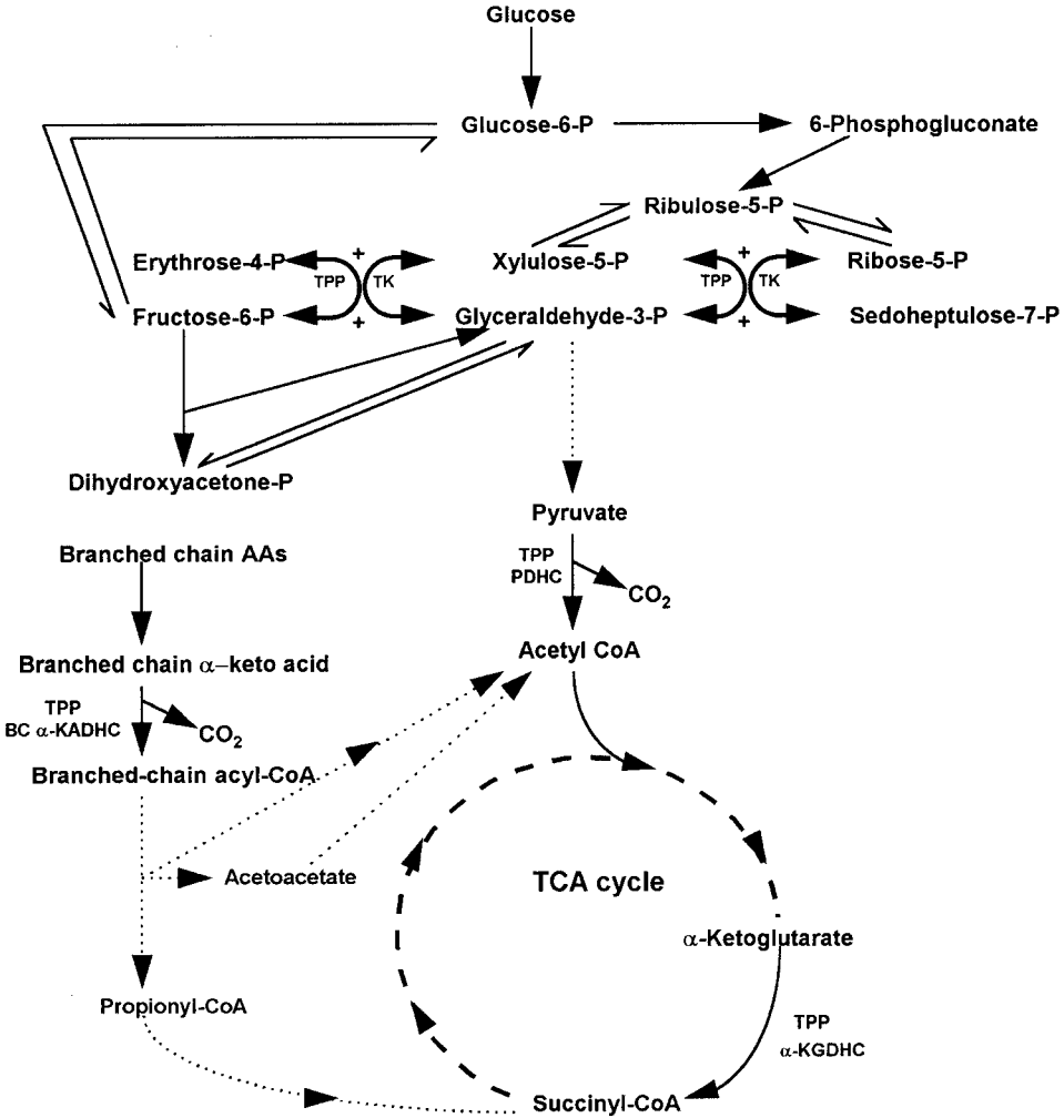
Fig. 8 Pathways dependent on thiamine pyrophosphate. P, phosphate; TPP, thiamine pyrophosphate; PDHC, pyruvate dehydrogenase complex; \alpha -KGDHC, \alpha -ketoglutarate dehydrogenase complex; BC \alpha -KADHC, branched-chain \alpha -keto acid dehydrogenase complex; TK, transketolase.
