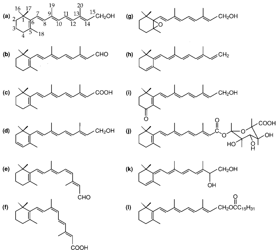
Fig. 1 Formulas for retinol and its derivatives. All are all- trans isomers except as noted. (a) retinol, (b) retinal, (c) retinoic acid, (d) 3,4-didehydroretinol, (e) 11- cis retinal, (f) 9- cis retinoic acid, (g) 5,6-epoxyretinol, (h) retro anhydroretinol, (i) 4-oxoretinol, (j) retinoyl β-glucuronide, (k) 14-hydroxy-4,14- retro retinol, (l) retinyl palmitate.
