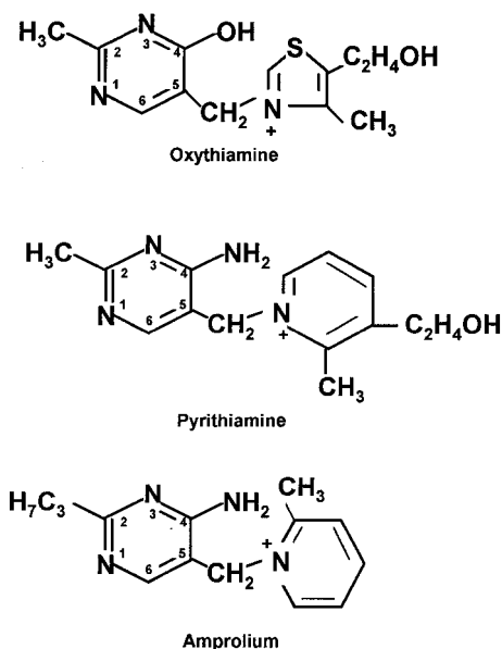
Fig. 5 Structural formulas of thiamine antagonists.
