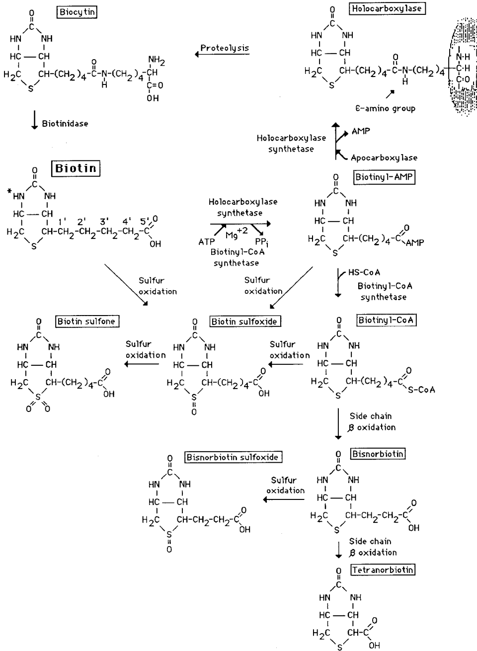
Fig. 1 Biotin metabolism. The specific systems leading to the sulfoxides have not been defined. ATP, adenosine triphosphate; AMP, adenosine monophosphate; HS-CoA, coenzyme A; PP i pyrophosphate; *, site of attachment of carboxyl moiety. (Courtesy of International Life Sciences Institute, Washington, D.C., M. Brown, ed.)
