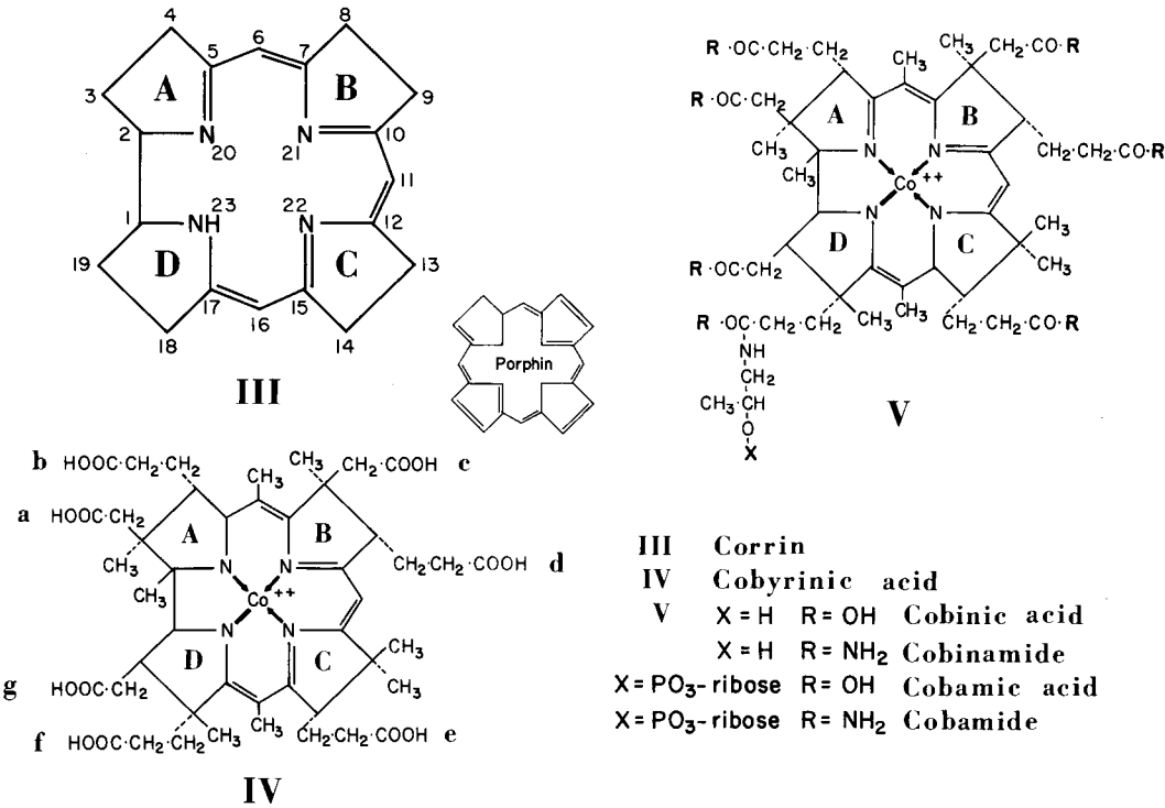
Fig. 3 Systematic nomenclature of cobalamin and related compounds. Inset shows porphyrin structure for comparison. Note that pyrrole rings of the corrin macro rings are designated A–D. Substituent acetamide and propionamide groups are designated a–g.
