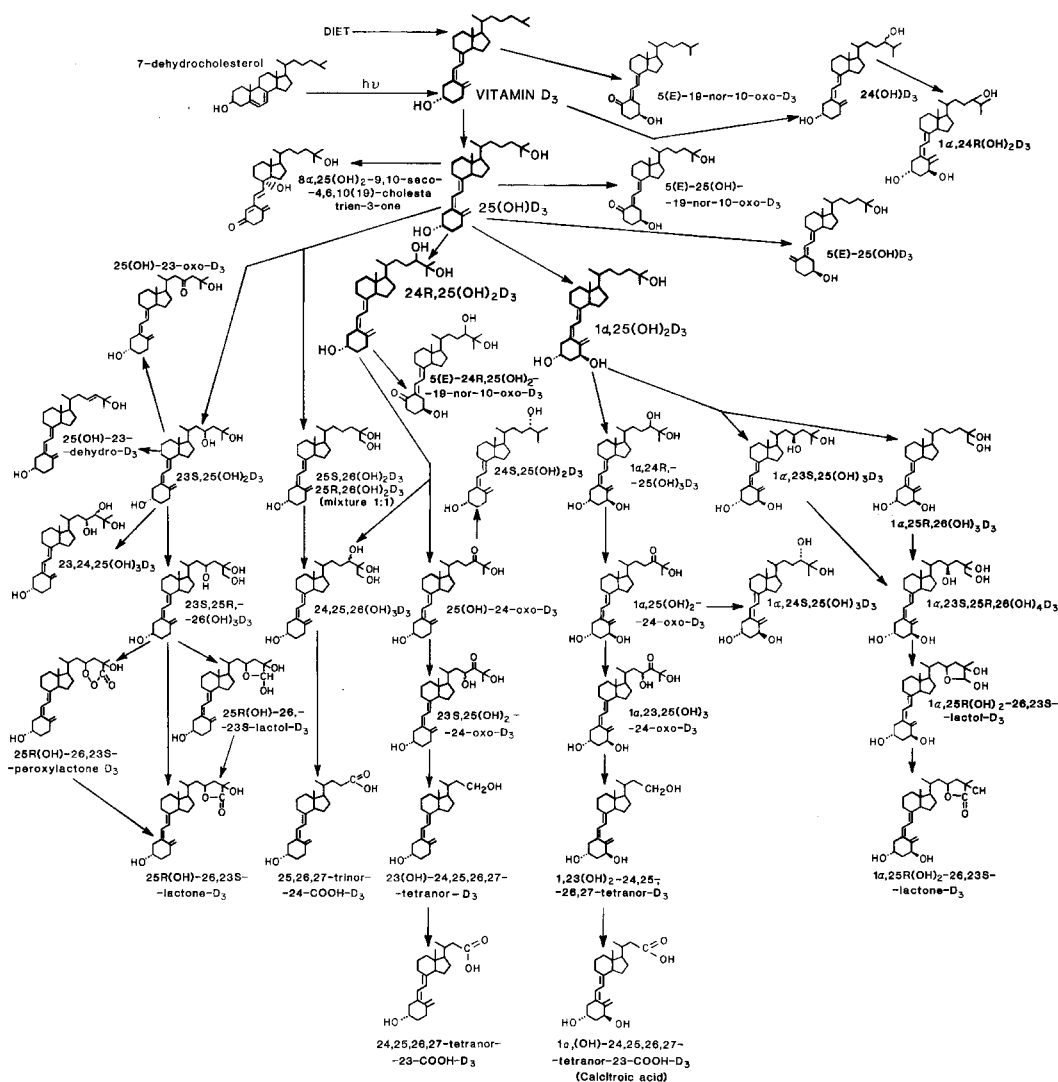
Fig. 5 Summary of the metabolic transformations of vitamin D_3 . Shown here are the structures of all known chemically characterized vitamin D_3 metabolites.
