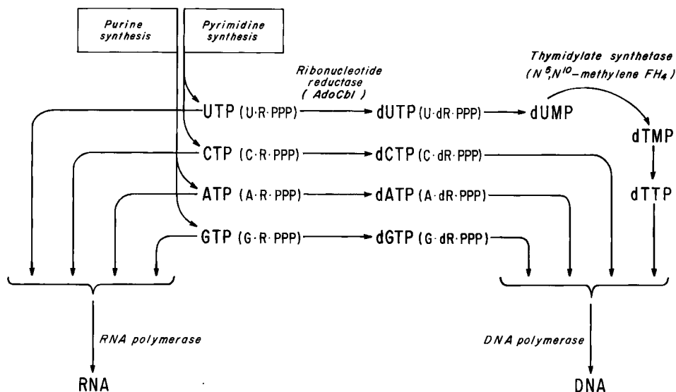
Fig. 8 Pathways of nucleotide and nucleic acid in Lactobacillus leichmannii .
