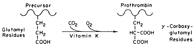
Fig. 4 The vitamin K-dependent carboxylation reaction.
