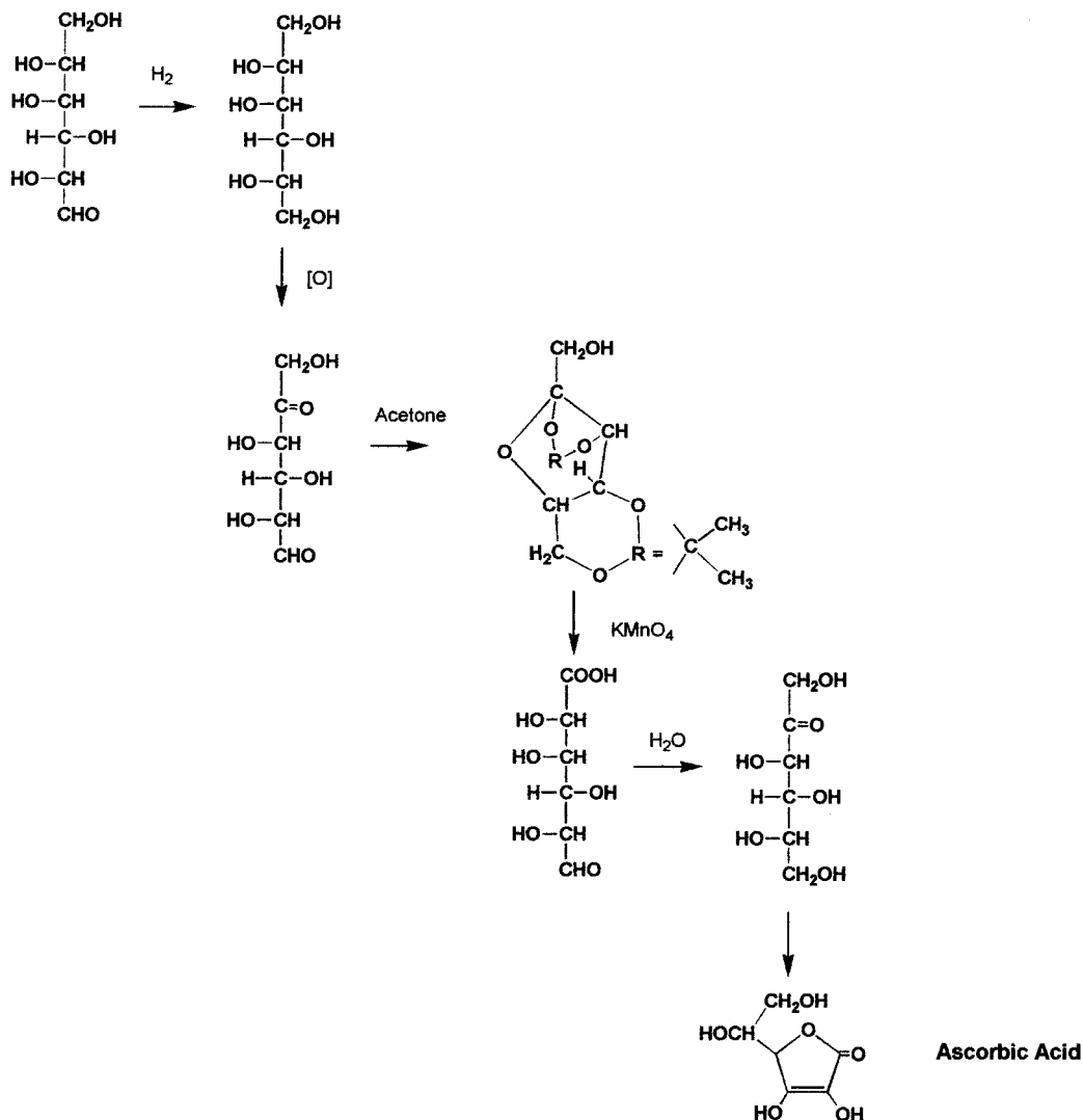
Fig. 2 Chemical synthesis of ascorbic acid from D-glucose.
