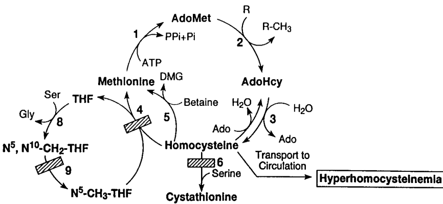
Fig. 4 The folate-dependent methionine resynthesis cycle and its relationship to transmethylation and transsulfuration cycles in tissues. The numbers refer to reactions catalyzed by the homocysteine remethylation cycle (8, serine hydroxymethyltransferase; 9, methylenetetrahydrofolate reductase; 4, B 12 -dependent methionine synthase; 5, betaine methyltransferase), the transmethylation cycle (1, adenosylmethionine synthetase; 2, R-methyltransferase; 3, adenosylhomocysteine hydrolase), and the transsulfuration pathway (6, cystathionine β-synthase). Genetic defects in key enzymes of homocysteine metabolism that lead to hyperhomocysteinemia and homocystinuria are indicated by the blocks. (From Ref. 125.)
