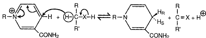
Fig. 1 The stereospecific hydride ion transfer to and from nicotinamide coenzymes generating prochiral R and S forms.
