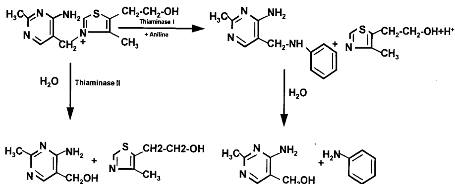
Fig. 6 Cleavage of thiamine by thiaminase I and thiaminase II. Thiaminase I activity requires organic bases or thiol compounds.
