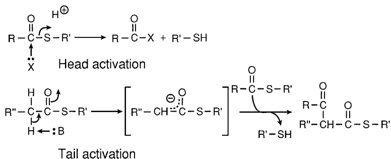
Fig. 7 Activations of acyl moieties enhanced by formation of thio esters with phosphopantetheine coenzymes.
