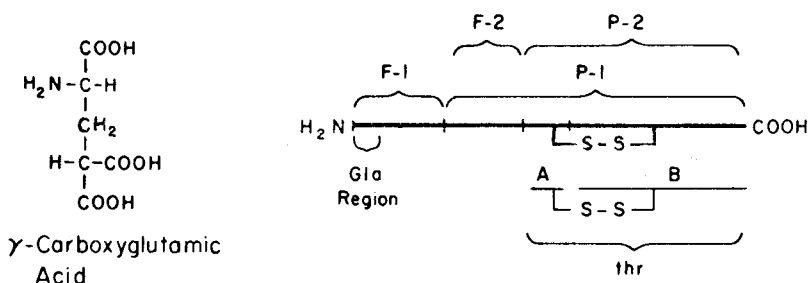
Fig. 3 Structure of \gamma -carboxyglutamic acid (Gla) and a diagrammatic representation of the prothrombin molecule. Specific proteolysis of prothrombin by factor \text{X}_s and thrombin will cleave prothrombin into the specific large peptides shown: fragment 1 (F-1), fragment 2 (F-2), prethrombin 1 (P-1), prethrombin 2 (P-2), and thrombin (thr). For details of the activation of prothrombin to thrombin and for sequences of vitamin K-dependent proteins, see Ref. (146). The Gla residues in bovine prothrombin are located at residues 7, 8, 15, 17, 20, 21, 26, 27, 30, and 33, and they occupy homologous positions in the other vitamin K-dependent plasma proteins.
