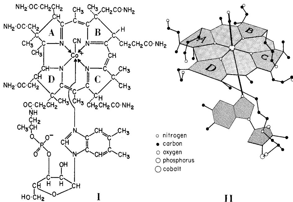
Fig. 1 Cobalamin. I , chemical structures of cyanocobalamin. II , semidiagrammatic representation of three-dimensional structure showing relations of planar and nucleotide moieties. Hydrogen atoms and a number of oxygen atoms are omitted.
