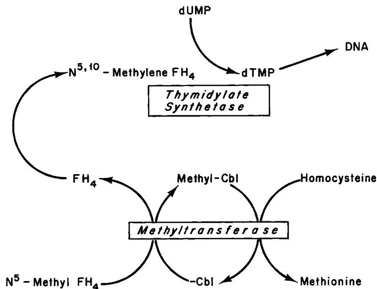
Fig. 9 Methylcobalamin-dependent pathway of methionine synthesis, showing essential role of cobalamin-dependent methyltransferase in conversion of N^5 -methyl FH_4 to FH_4 . If folate is “trapped” as N^5 -methyl FH_4 , it cannot be converted to N^{5,10} -methylene FH_4 , the cofactor of thymidylate synthetase.
