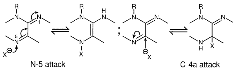
Fig. 4 Reaction types encountered with flavoquinone coenzymes and natural nucleophiles to generate N-5 and C-4a adducts as intermediates.
