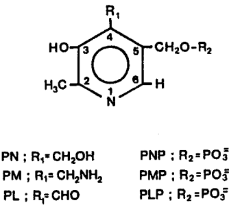
Fig. 1 Structure of B 6 vitamers.
