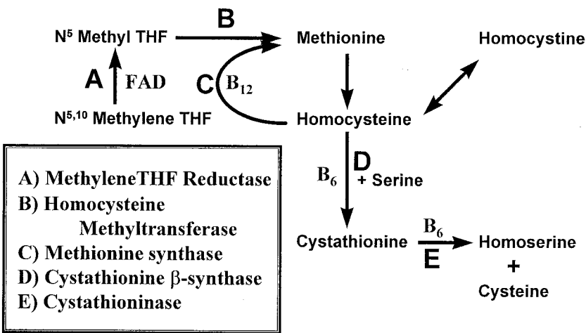
Fig. 5 Diagrammatic representation of homocysteine metabolism, showing the roles of folic acid, B 12 , B 6 , and riboflavin. FAD is the coenzyme for methylenetetrahydrofolate reductase.
