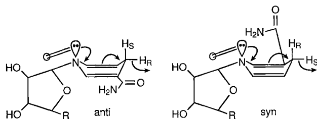
Fig. 2 The syn and anti conformations of bound nicotinamide coenzymes that putatively transfer pro-(S) and pro-(R) hydrogens, respectively.
