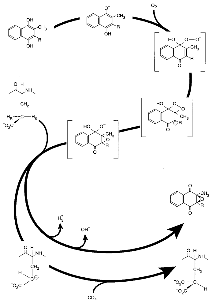
Fig. 5 Proposed mechanism of action for the vitamin K-dependent carboxylase enzyme. The available data support the interaction of O_2 with the reduced form of vitamin K to form an oxygenated intermediate that is sufficiently basic to abstract the \gamma -hydrogen of the glutamyl residue. The products of this reaction would be vitamin K epoxide and a glutamyl carbanion. The bracketed peroxy, dioxetane, and alkoxide intermediates have not been identified in the enzyme-catalyzed reaction but are postulated based on model organic reactions.
