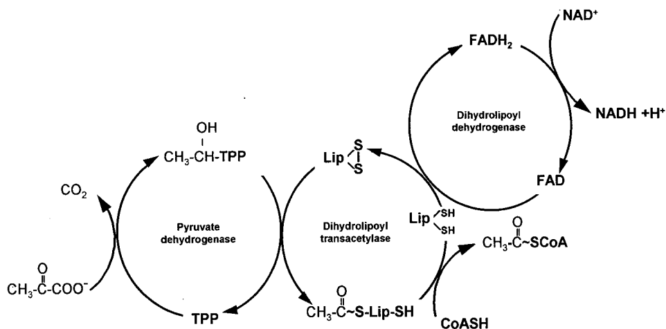
Fig. 7 The pyruvate dehydrogenase complex reactions. TPP, thiamine pyrophosphate; Lip, lipoic acid.
