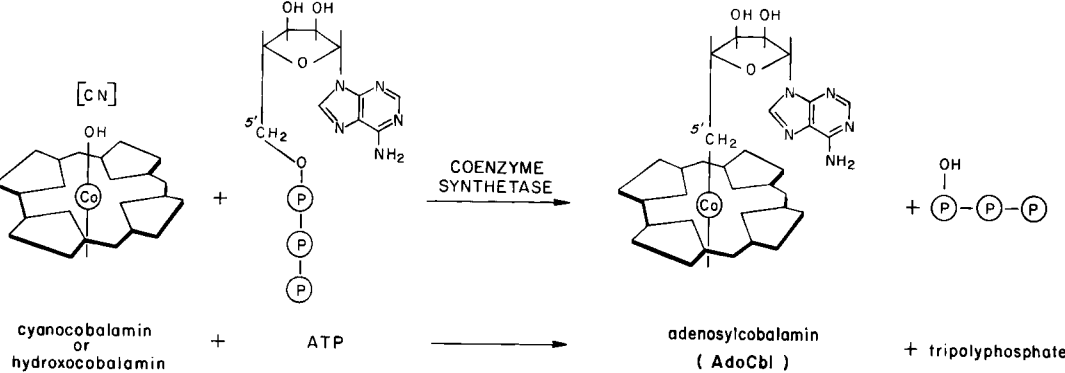
Fig. 4 The coenzyme synthetase reaction. ATP adenosylates cobalamin to form adenosylcobalamin.
