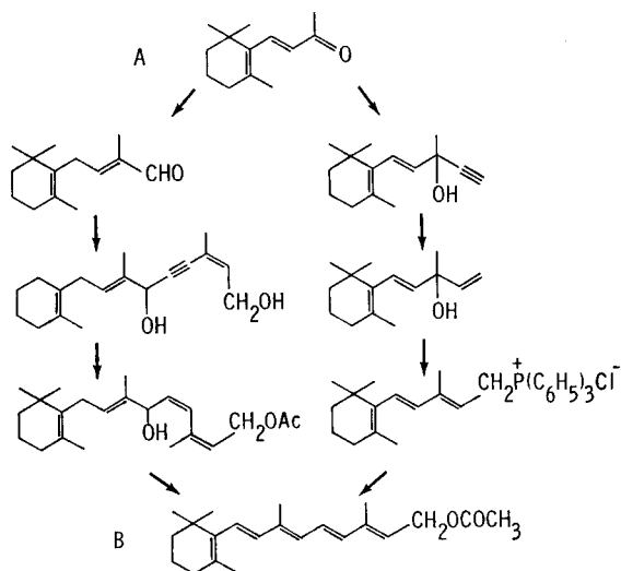
Fig. 4 Major commercial routes to the synthesis of retinyl acetate (B) from \beta -ionone (A). The Isler (Roche) procedure is on the left, the Wittig (BASF) method on the right.
