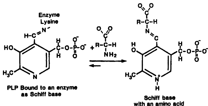
Fig. 2 Schiff base formation between pyridoxal-5'-phosphate and an amino acid.
