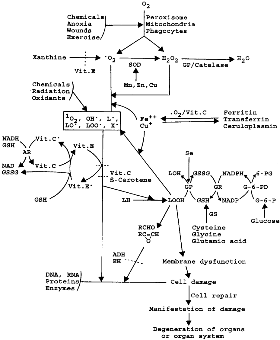
Fig. 3 Relationship between vitamin E and other antioxidant systems. LH represents membrane or polyunsaturated lipids; LOOH, lipid hydroperoxides, LOH, hydroxy acid; LOO \cdot , peroxy radical; L \cdot , alkyl radical; LO \cdot , alkoxy radical; OH \cdot , hydroxyl radical; \cdot O_2 , superoxide radical; X \cdot , other radicals; ^1O_2 , singlet oxygen; H_2O_2 , hydrogen peroxide; RCHO, aldehydes; \begin{matrix} RC=CH \\ \diagup \quad \diagdown \\ O \end{matrix} , epoxides; Vit.E \cdot , vitamin E radical; Vit.C \cdot , ascorbate radical or dehydroascorbate; 6-PG, 6-phosphogluconate; GSH, reduced glutathione; GSSG, oxidized glutathione; NADH and NAD, reduced and oxidized nicotinamide adenine dinucleotide, respectively; NADPH and NADP, reduced and oxidized nicotinamide dinucleotide phosphate, respectively; Se selenium; SOD, superoxide dismutase; GP, GSH peroxidase or phospholipid hydroperoxide GSH peroxidase; GR, GSSG reductase; G-6-PD, glucose-6-phosphate dehydrogenase; ADH, aldehyde dehydrogenase; EH, epoxide hydrazase; AR, ascorbate or dehydroascorbate reductase.
