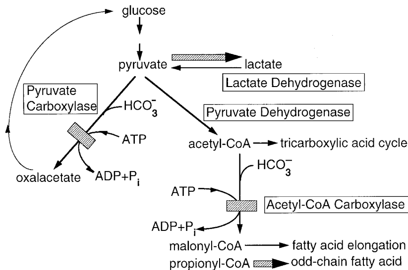
Fig. 2 Lactate and pyruvate metabolism. Deficiencies (▨) of PC and ACC can redirect intermediates into unusual pathways (▨→). Abbreviations as in Fig. 1. ADP, adenosine diphosphate; P i , inorganic phosphate.
