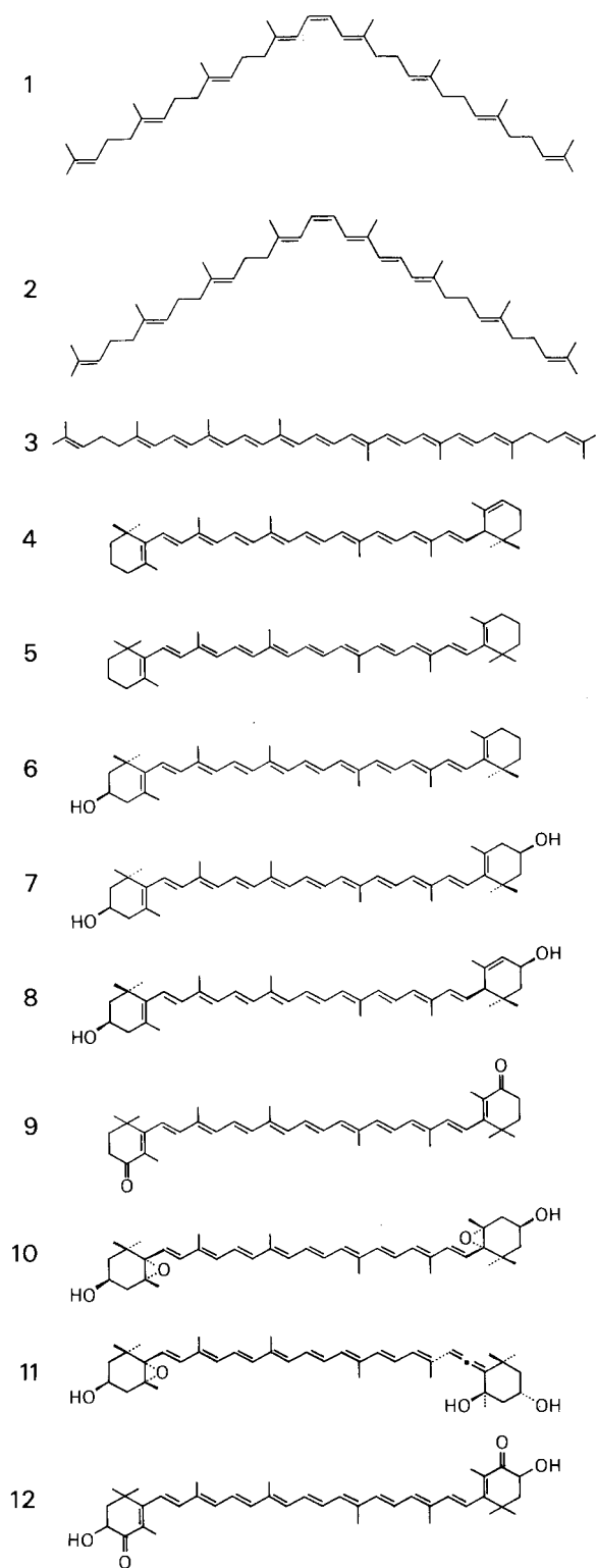
Fig. 2 Polyenes and carotenoids in foods that may also be found in animal tissues. 1, phytoene; 2, phytofluene; 3, lycopene; 4, \alpha -carotene; 5, \beta -carotene; 6, \beta -cryptoxanthin; 7, zeaxanthin; 8, lutein; 9, canthaxanthin; 10, violaxanthin; 11, neoxanthin; 12, astaxanthin. (From Ref. 139.)
