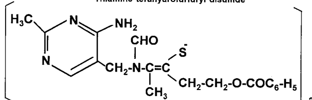
O-Benzoylthiamine disulfide
