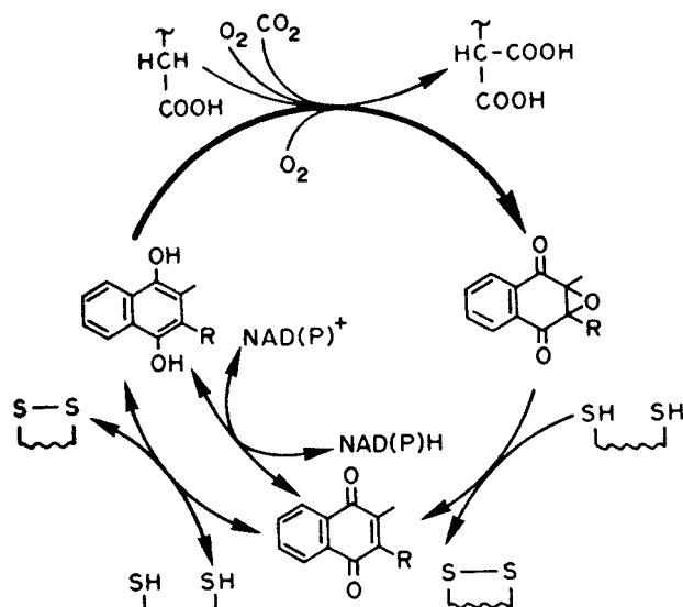
Fig. 6 Vitamin K-related activities in rat liver microsomes. Vitamin K epoxide formed in the carboxylation reaction is reduced by a warfarin-sensitive pathway “vitamin K epoxide reductase” that is driven by dithiothreitol (DTT) as a reducing agent in in vitro studies. The quinone form of the vitamin can be reduced to the hydroquinone either by a warfarin-sensitive DTT-driven quinone reductase or by one or more nicotinamide nucleotide-linked quinone reductases which are less sensitive to warfarin. Warfarin and other coumarin anticoagulants do not have a significant effect on the carboxylase/epoxidase activity.
