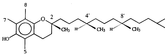
Toco Structure
