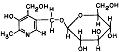
Fig. 3 Structure of 5'-O-(β-D-glucopyranosyl)pyridoxine.
