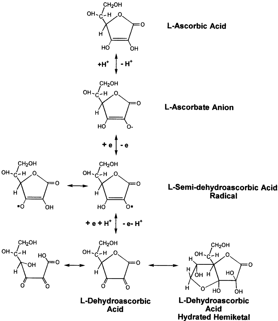
Fig. 1 Ascorbic acid and various oxidation products. The two predominant forms of ascorbic acid and their associated oxidation products are shown. In solution, ascorbic acid probably exists as the hydrated hemiketal.
