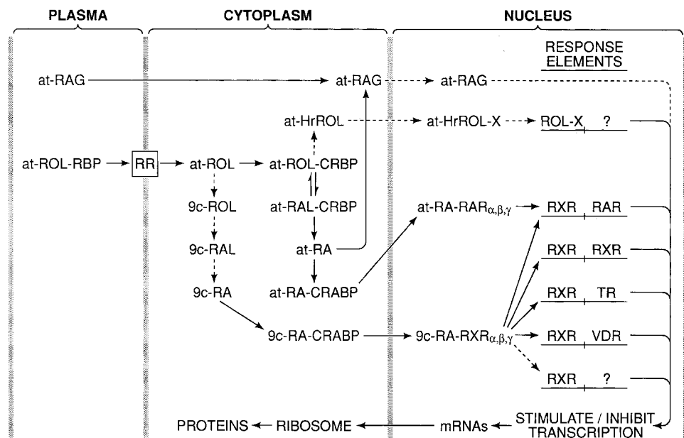
Fig. 9 Roles of retinoids in cellular differentiation at, All- trans ; 9 c , 9- cis , ROL, retinol; HrROL, 14-hydroxy-4,14- retro retinol; RAL, retinal; RA, retinoic acid; RAG, retinoyl \beta -glucuronide; RR, cell surface receptor for holo-RBP; BBP, plasma retinol-binding protein; CRBP, cellular retinol-binding protein; CRABP, cellular retinoic acid-binding protein; RAR _{\alpha, \beta, \gamma} , nuclear retinoic acid receptors, forms \alpha , \beta , and \gamma ; RXR _{\alpha, \beta, \gamma} , nuclear 9- cis retinoic acid receptors, forms \alpha , \beta , \gamma ; TR, triiodothyronine bound to the nuclear thyroid receptor; VDR, calcitriol bound to the nuclear vitamin D receptor; X, unknown nuclear receptors; solid arrows, known transformations or effects; dashed arrows, postulated transformations or effects; ?, unknown occupancy. (From Ref. 39.)
