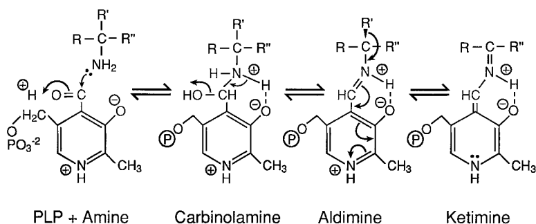
Fig. 6 Operation of pyridoxal-5'-phosphate with a biological primary amine. Loss of R' shown from the aldimine can be generalized for side-chain cleavages and eliminations, loss of CO_2 in decarboxylations, or loss of a proton in aminotransferations and racemizations.
