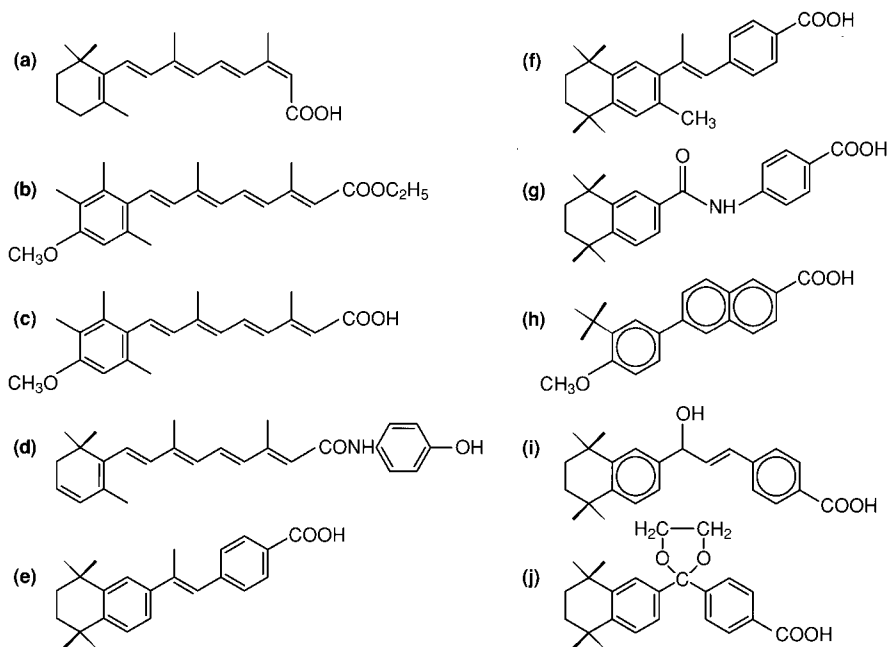
Fig. 3 Some synthetic retinoids with specific therapeutic or protein-binding properties. (a) 13- cis retinoic acid, (b) etretinate, (c) acitretin, (d) 4-hydroxyphenylretinamide (HPR, Fenretinide), (e) tetrahydrotetramethylnaphthalenylpropenylbenzoic acid (TTNPB), (f) 3-methyl TTNPB, (g) AM-580, (h) CD-417, (i) CD-666, (j) SR-11237.
