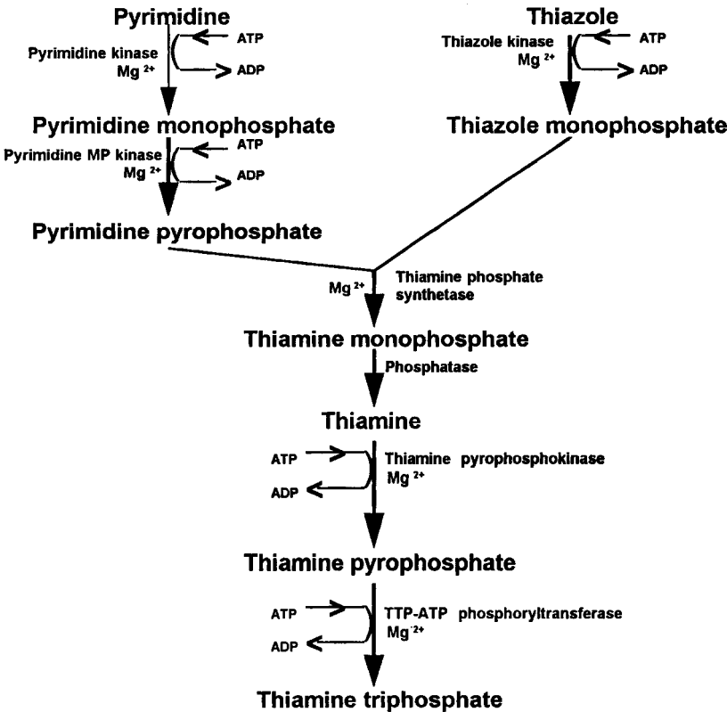
Fig. 2 Biosynthetic pathway of thiamine and its phosphorylated derivatives. Pyrimidine, 2-methyl-4-amino-5-hydroxymethylpyrimidine; thiazole, 4-methyl-5-(2-hydroxymethyl)thiazole; MP, monophosphate; TTP, thiamine triphosphate.
