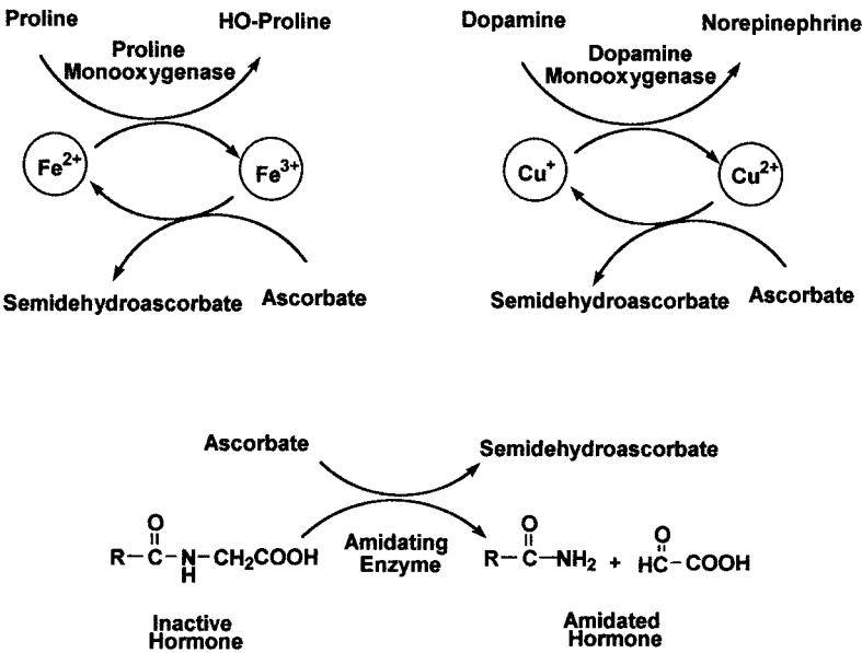
Fig. 5 Reactions catalyzed by mono- and dioxygenases for which ascorbic acid and iron or copper are catalyst. Reaction sequences for hydroxyprolyl synthesis, norepinephrine synthesis, and C-terminal amidation formation are indicated.
