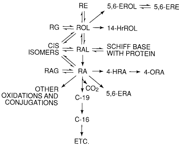
Fig. 6 Major metabolic transformations of vitamin A. ROL, retinol; RE, retinyl ester; RAL, retinal; RA, retinoic acid; RG, retinyl \beta -glucuronide; RAG, retinoyl \beta -glucuronide; 5,6-EROL, 5,6-epoxyretinol; 5,6-ERE, 5,6-epoxyretinyl ester; 14-HrROL, 14-hydroxy-4,14-retinol; 4-HRA, 4-hydroxyretinoic acid; 4-ORA, 4-oxoretinoic acid; 5,6-ERA, 5,6-epoxyretinoic acid; C-19 and C-16, chain-shortened, oxidized products with the indicated number of carbon atoms. Double arrows indicate reversible reactions; single arrows irreversible changes. (From Ref. 39.)
