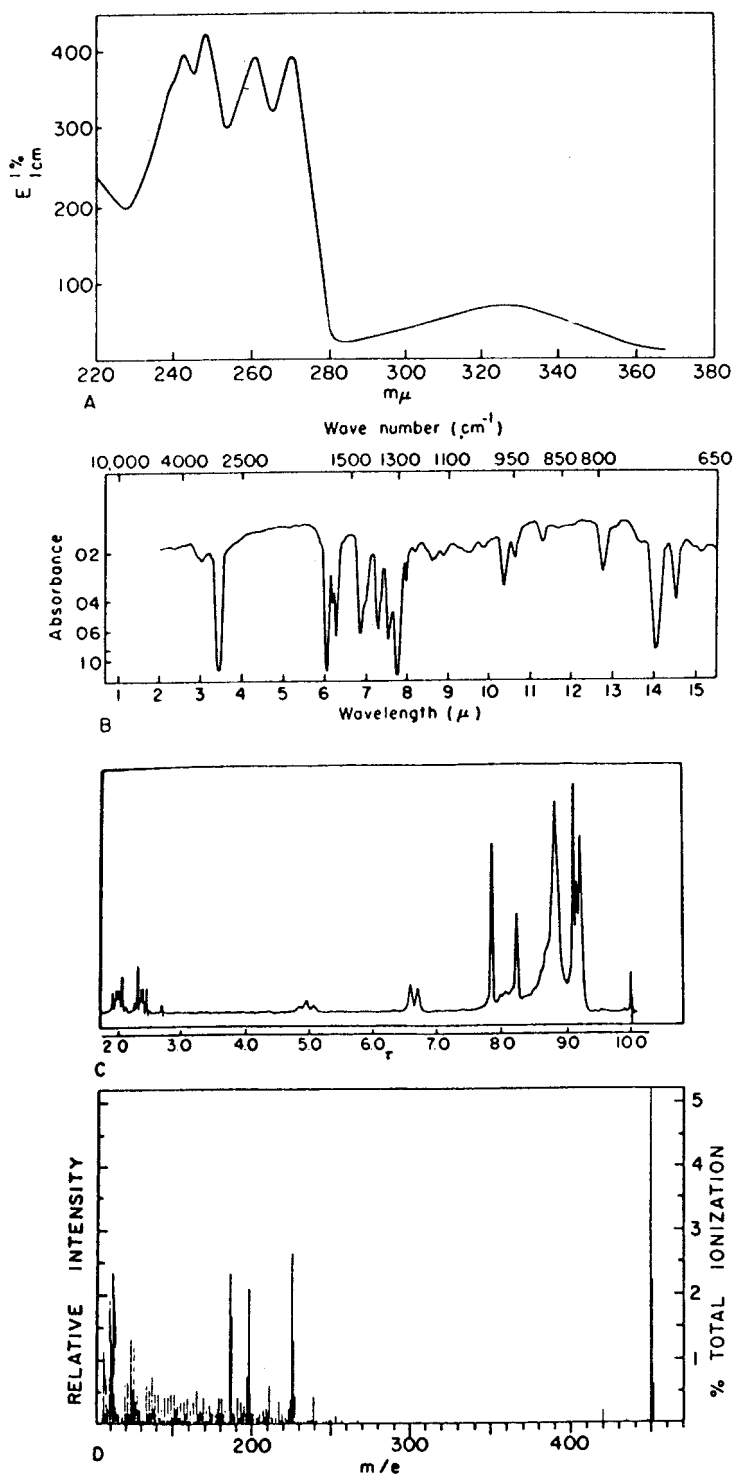
Fig. 1 Physical properties of phylloquinone. (A) Ultraviolet absorption spectra in petroleum ether. (B) Infrared absorption spectra. (C) Nuclear magnetic resonance spectra in CDCl_3 at 60 Mc. (D) Mass fragmentation spectrum of the parent molecular ion is seen at m/e 450.
