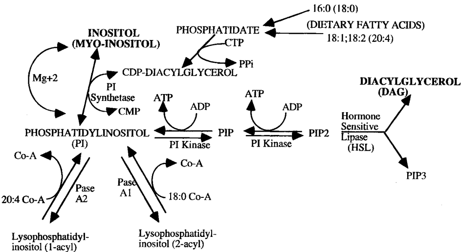
Fig. 2 Myoinositol metabolic pathway. Mg+2, magnesium; PI kinase, phosphoinositol kinase; Pase A1, phospholipase A1; Pase A2, phospholipase A2; Co-A, coenzyme A; PIP, phosphoinositol phosphate; PIP2, phosphoinositol biphosphate; PIP3, phosphoinositol triphosphate.
