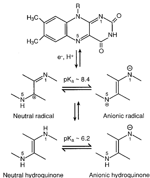
Fig. 3 Biologically important redox states of flavocoenzymes with \text{pK}_a values for interconversions of the free species.
