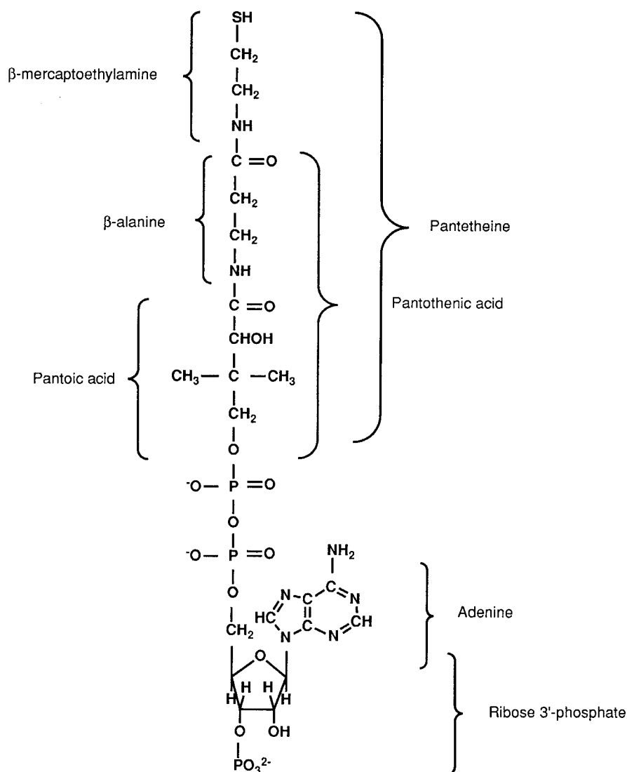
Fig. 1 Coenzyme A and intermediates.
