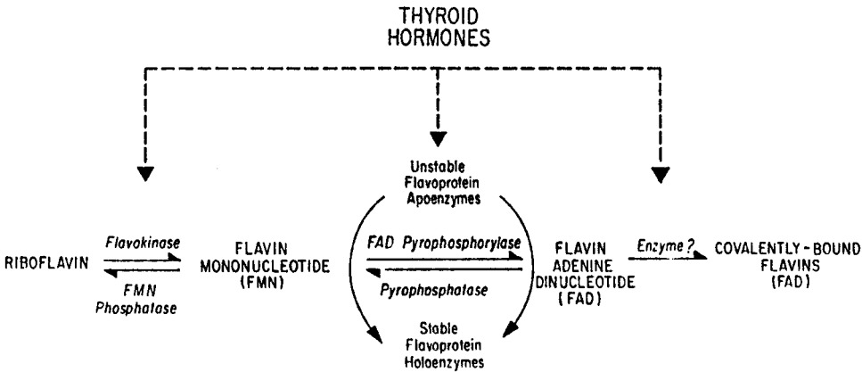
Fig. 2 Metabolic pathway of conversion of riboflavin into FMN, FAD, and covalently bound flavin, together with its control by thyroid hormones (12).
