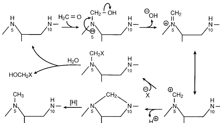
Fig. 11 Reaction of formaldehyde with the basic N-5 of tetrahydrofolyl coenzyme to generate an N-hydroxymethyl intermediate that leads to a mesomeric carbocation. This latter can react intermolecularly in a Mannich-like reaction or intramolecularly to form 5,10-methylene tetrahydrofolate.
