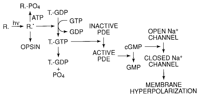
Fig. 7 Possible sequence of steps between the light-induced activation of rhodopsin and hyperpolarization of the rod cell membrane. R., Rhodopsin; R: light-activated metarhodopsin II; R-PO 4 , phosphorylated rhodopsin; ATP, adenosine triphosphate; GTP, guanosine triphosphate; GDP, guanosine diphosphate; cGMP, cyclic 3'-5'-guanosine monophosphate; GMP, guanosine monophosphate; T., transducin; T.-GDP, a complex of transducin with GDP; T.-GTP, a complex of transducin with GTP; PDE, phosphodiesterase. (From Ref. 39.)
