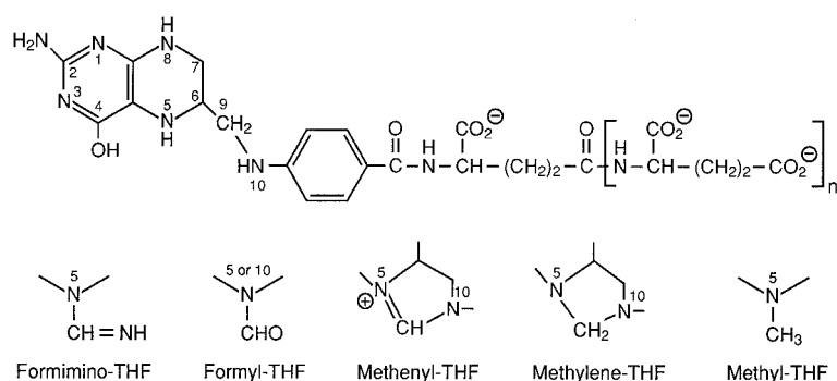
Fig. 10 Structures with numbering for tetrahydropteroyl-L-glutamates, including the biological derivatives for one-carbon transfers.
