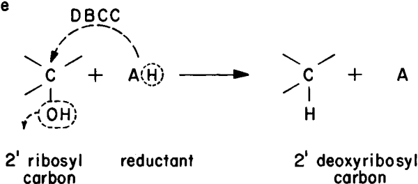
Fig. 7 Parallel mechanisms in reactions catalyzed by dioldehydrase and ribonucleotide reductase. In both, an H displaces an OH. The H derives from an outside reductant only in the reductase reaction. Note: DBCC is AdoCbl.
