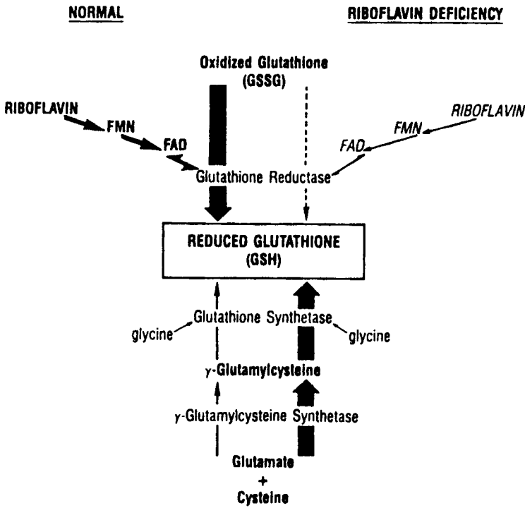
Fig. 3 Diagrammatic representation of metabolic adaptations to riboflavin deficiency. Diminished conversion of oxidized glutathione to reduced glutathione occurs as a result of decreased activity of glutathione reductase, an enzyme that utilizes FAD as a coenzyme. Levels of reduced glutathione are maintained by enhanced de novo synthesis from precursors (31,32).
