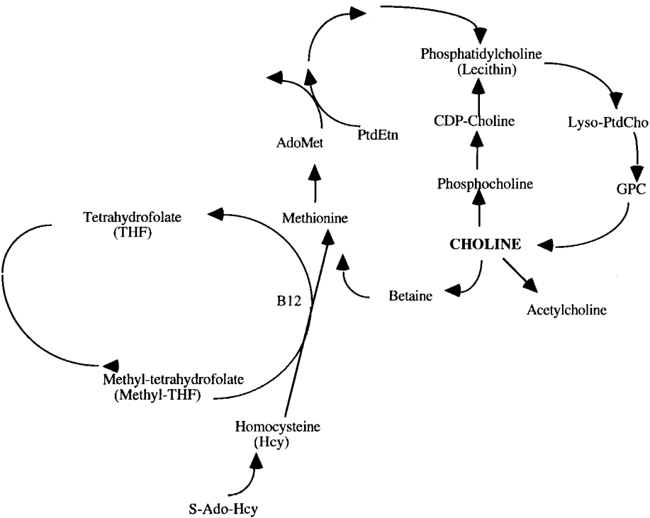
Fig. 1 Choline metabolic pathway is interrelated with folate, methionine, and B 12 metabolism. S-AdoMet, S-adenosylmethionine; CDP-Choline, choline–cytidine diphosphocholine; PtdEtn, phosphatidylethanolamine; GPC, glycerophosphocholine; LysoCho, lysophosphatidylcholine; S-AdoHcy, S-adenosylhomocysteine.
