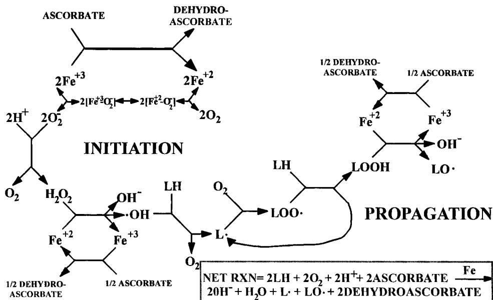
Fig. 1 Mechanism of ascorbate-induced lipid peroxidation (99).
