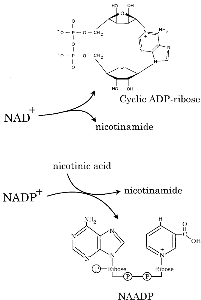
Fig. 4 Structures and origin of cyclic ADP-ribose and NAADP.
