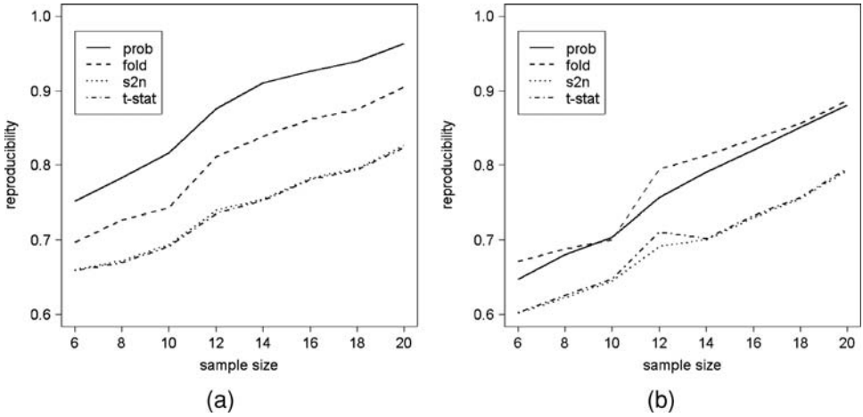
FIGURE 4. (a) Reproducibility of: the posterior probability (solid line); the estimate of the fold change (dashed line); the t -statistic (dash-dot line) and the signal-to-noise ratio (dotted line) for different sample sizes, for the 1329 genes selected as most differentially expressed by BADGE on the whole data set; (b) the same analysis for the 1329 genes selected as most differentially expressed by the t -statistic. The reproducibility is measured by (1 + \rho_i)/2 , where \rho_i is the average correlation between statistics in samples of size n_i (= 6, \dots, 20) .
