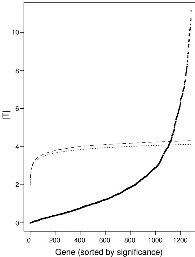
FIGURE 1. Ordered |T_i| values (solid dots) with normal distribution critical values (dotted line) and bootstrap critical values (dashed line) for the stepdown method.
