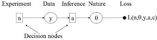
FIGURE 5. A decision tree for the choice of sample size and inference method. The first decision node represents the choice of the sample size n . After this decision, the experiment is conducted and generates the data y that are assumed to follow a distribution with parameter \theta . The data are used to make an inference on the parameter \theta , and the second decision node a represents the statistical procedure that is used to make this inference. The last node represents the loss induced by choosing such an experiment.
