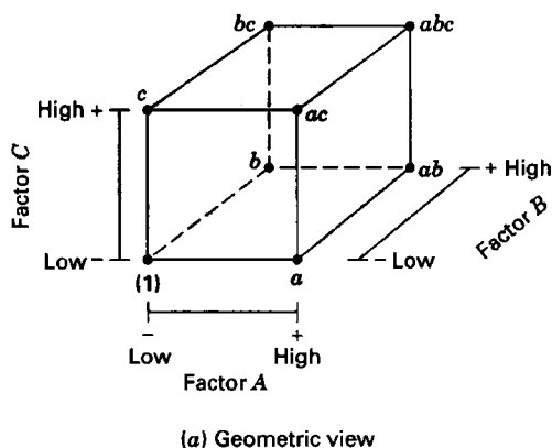
FIGURE 1. A 2^3 factorial design.
