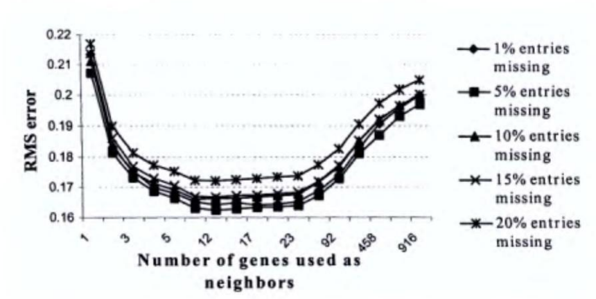
Figure 3.1. Effect of number of nearest neighbors ( K ) parameter on KNN-based estimation (on noisy time series data). Different curves correspond to experiments performed for data sets with different percent of entries missing.
