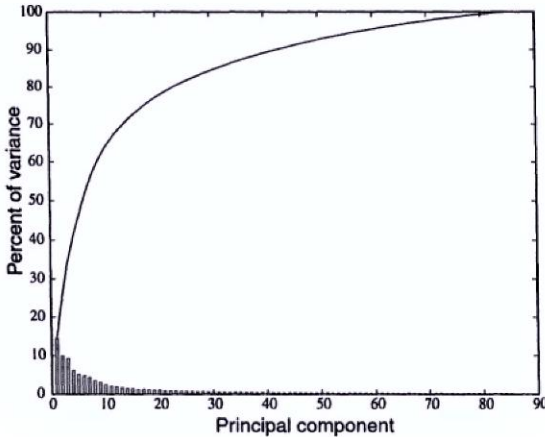
Figure 11.1. The percent of variance in the SRBCT gene expression data matrix (all 88 samples) contained by each principal component (bars). The cumulative contained variance is also shown (solid line). The 10 first principal components contain more than 60% of the variance in the data matrix for this example.
