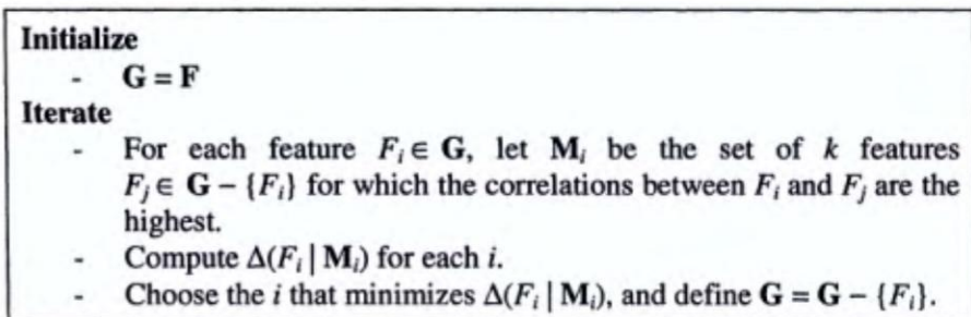
Figure 6.3. The Markov blanket filtering algorithm.
