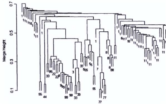
Figure 14.9. Adaptive single linkage dendrogram of the lymphoma data following imputation for missing values, with known tissue classes labeled.
