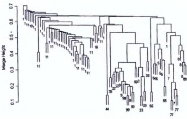
Figure 14.7. Adaptive single linkage dendrogram of the lymphoma data set with known tissue classes labeled.
