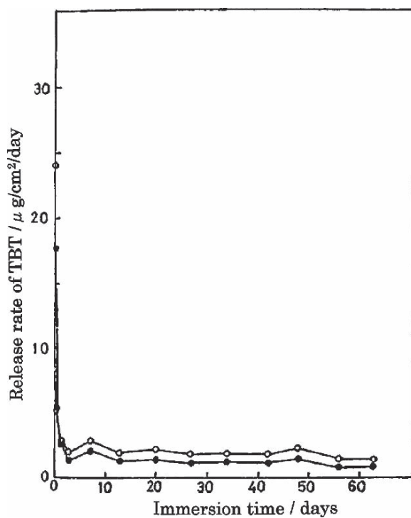
Fig. 1.9 The TBT release rate curves from TBT-SPC antifouling paints ○: ASTM/ISO method and ●: Ketchum method
