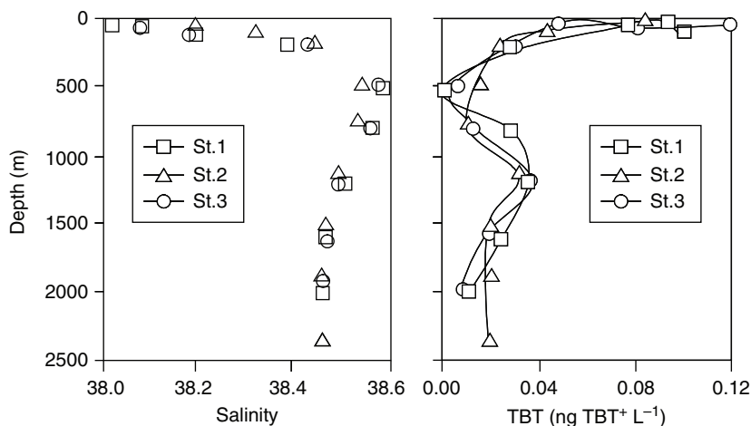
Fig. 6.1 The vertical profile of TBT and salinity in Mediterranean Sea (Borgi and Porte 2002)
