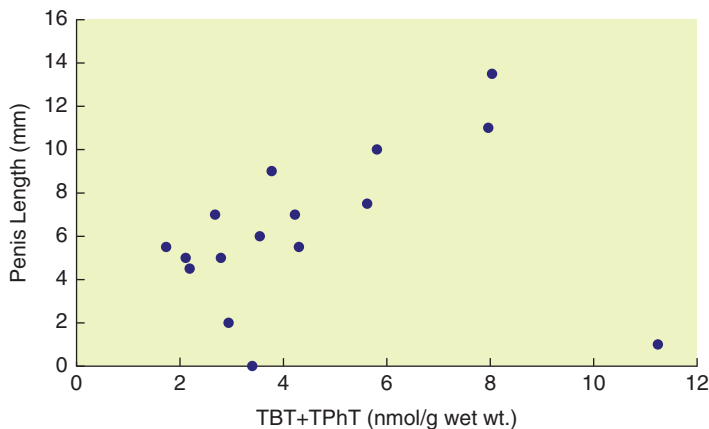
Fig. 8.6 Relationship between triorganotin (the sum of tributyltin and triphenyltin) concentrations in gonads and penis length in female Babylonisa japonica (Horiguchi et al. 2006)
