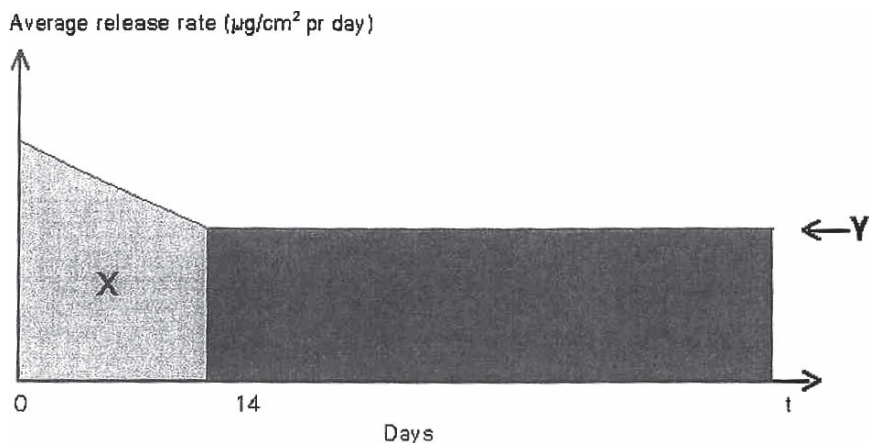
Fig. 1.6 CEPE/mass-balance calculation model X: the amount of biocide released during the first 14 days ( \mu\text{g}/\text{cm}^2 ); Y: the average release rate during the rest of the lifetime ( \mu\text{g}/\text{cm}^2/\text{day} )
