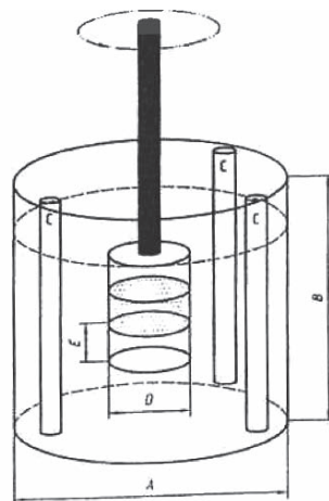
Fig. 1.4 The release rate measuring container and test cylinder in ISO 15181-1 standard method
