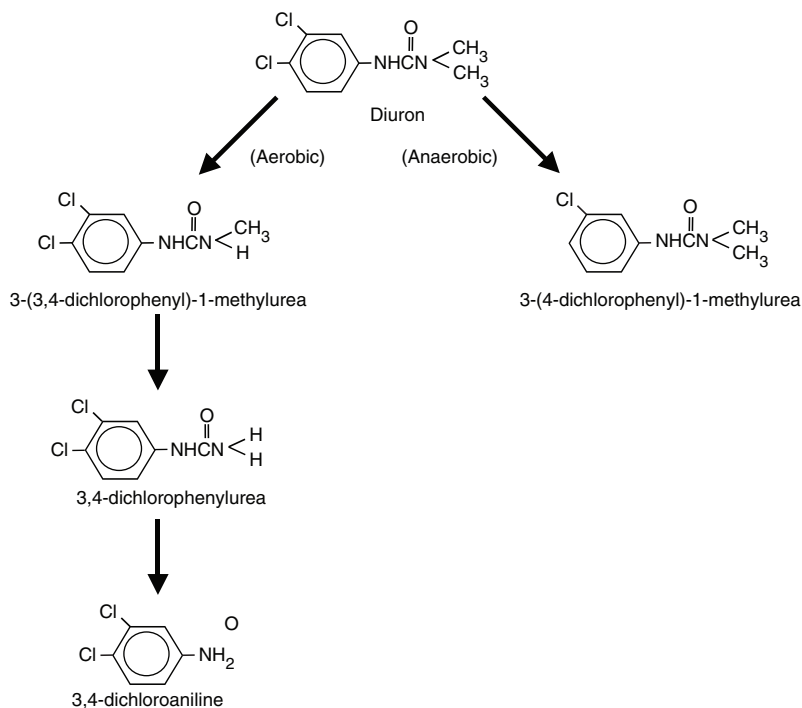
Fig. 23.4 Degradation pathway of diuron (Ellis and Camber 1982)
