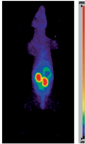
FIG. 7.13. Ventrordorsal static image of a healthy dog 4 h post-injection of ^{99m}\text{Tc} -HYNIC-TATE.
