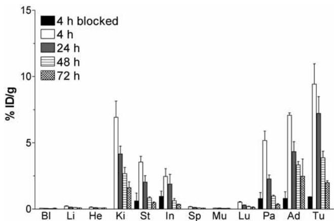
FIG. 6.9. Biodistribution of ^{177}\text{Lu} -DOTATATE in AR42J tumour bearing athymic mice (given as the percentage of injected dose per gram of tissue) at 4, 24, 48 and 72 h post-injection; Bl = blood, Li = liver, He = heart, Ki = kidneys, St = stomach, In = intestine, Sp = spleen, Mu = muscle, Lu = lungs, Pa = pancreas, Ad = adrenal glands and Tu = AR42J tumour; uptake was blocked by co-injection of 100 \mu\text{g} of TATE.
