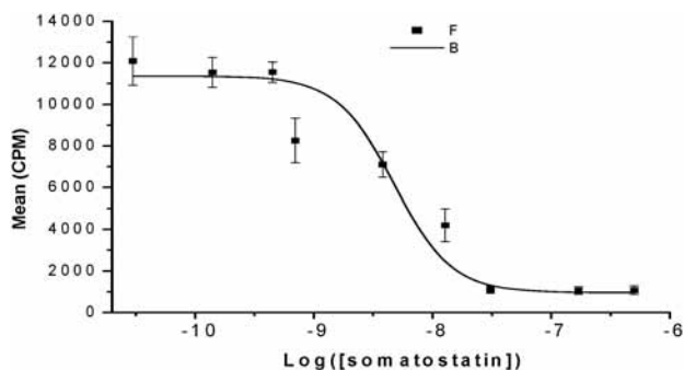
FIG. 14.5. Competitive binding curve for cold Lu-DOTATATE.
