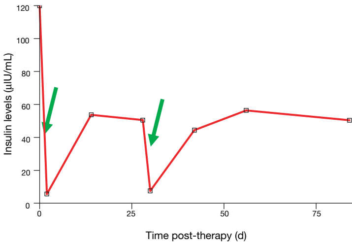
FIG. 7.19. Insulin levels in an insulinoma bearing dog treated with 90 Y-DOTATOC; the arrows indicate therapy cycles.
