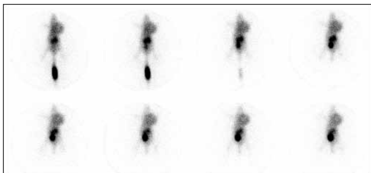
FIG. 3.11. Dynamic flux of [^{177}\text{Lu}]\text{DOTATATE} in a tumour bearing nude mouse, 3 min per image.
