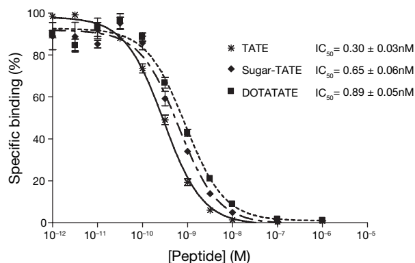
FIG. 6.6. Comparative displacement curves of [^{125}\text{I-Tyr}^3]\text{octreotide} from somatostatin receptor subtype 2 in AR42J cell membranes with increasing concentrations of TATE, Sugar-TATE and DOTATATE.
