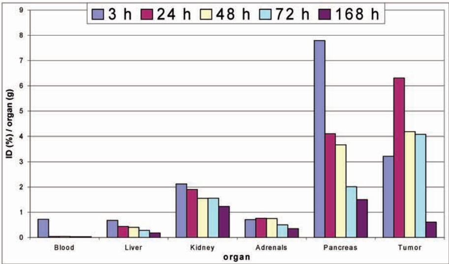
FIG. 14.8. Biodistribution of ^{177}\text{Lu} -DOTATATE in tissue expressing somatostatin subtype 2 receptors (adrenal gland, pancreas and tumour) compared with uptake in transport, metabolic and elimination tissues at various times post-injection.
