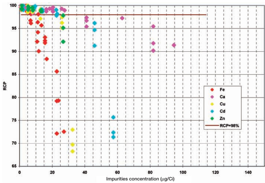
FIG. 13.11. Influence of chemical impurities on labelling yield of ^{90}\text{Y} -DOTATATE.
