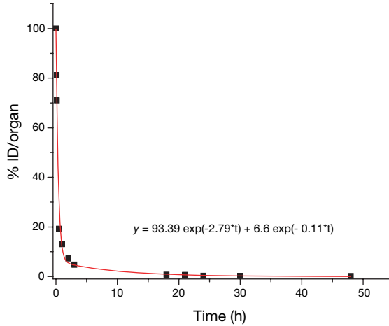
FIG. 7.17. Representative time versus blood activity curve of ^{90}\text{Y} -DOTATOC in a healthy dog.
