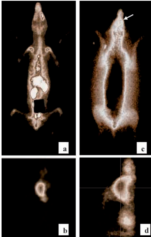
FIG. 7.5. Uptake of ^{99m}\text{Tc-DMSA(V)} and ^{188}\text{Re-DMSA(V)} in a dog with a fibrosarcoma: (a) ^{99m}\text{Tc-DMSA(V)} AP whole body image; (b) ^{99m}\text{Tc-DMSA(V)} sagittal SPECT plane of head; (c) ^{188}\text{Re-DMSA(V)} AP whole body image; (d) ^{188}\text{Re-DMSA(V)} sagittal SPECT plane of head.
