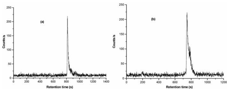
FIG. 8.6. HPLC patterns of ^{177}\text{Lu} -DOTATATE: (a) complexation at a concentration of 25 \mu\text{g} of peptide and (b) radiochemical purity after 7 d.
