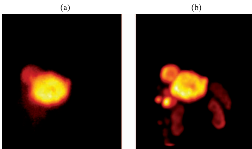
FIG. 13.13. Results of the first clinical trials with ^{90}\text{Y} -DOTATATE; diagnostic images of a 36 year old patient (patient No. 1) with a low grade neuroendocrine carcinoma: (a) ^{111}\text{In} -octreotide scan; (b) ^{99\text{m}}\text{Tc} -HYNIC-TATE scan.
