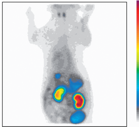
FIG. 7.15. Ventrordorsal static scintigram of an insulinoma bearing dog 4 h post-injection of ^{99m}\text{Tc} -HYNIC-TATE.
