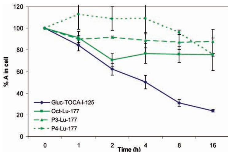
FIG. 16.10. Externalization of ^{177}\text{Lu} -OCT, ^{177}\text{Lu} -P3, ^{177}\text{Lu} -P4 and ^{125}\text{I} -Gluc-TOCA, expressed as the percentage of initial activity remaining in membrane and inside cell at different incubation times.
