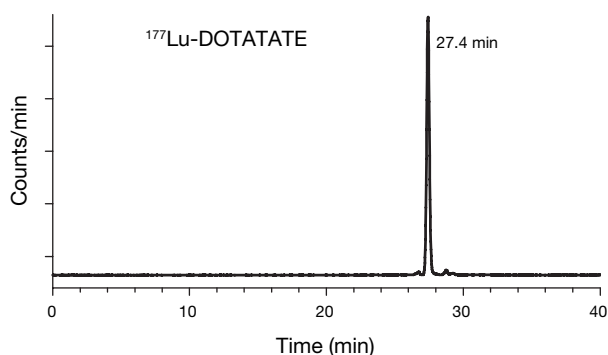
FIG. 6.5. HPLC analysis of ^{177}\text{Lu} -DOTATATE labelling reaction mixture.
