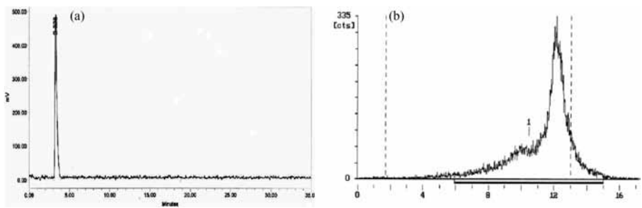
FIG. 10.2. HPLC and ITLC-SG analyses of ^{166}\text{Ho-DOTA} : (a) 10 \mu\text{L} of ^{166}\text{Ho-DOTA} injected into the HPLC system (retention time: 3.3 min); (b) ITLC (75% MeOH) with R_f = 0.9 (100% labelling yield).
