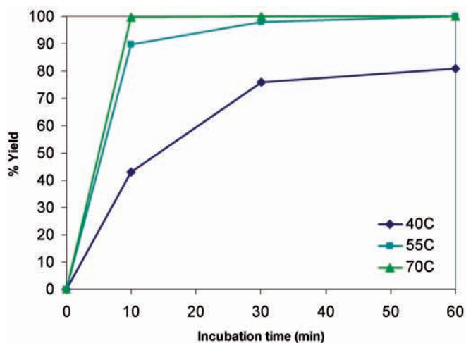
FIG. 16.6. Kinetics of ^{177}\text{Lu} -P3 labelling at different incubation temperatures, as determined by reversed phase HPLC.
