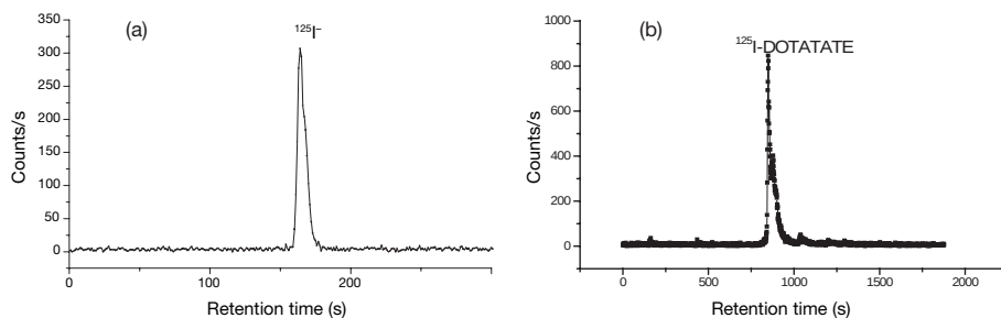
FIG. 8.11. HPLC patterns of (a) ^{125}\text{I} and (b) ^{125}\text{I} -DOTATATE.
