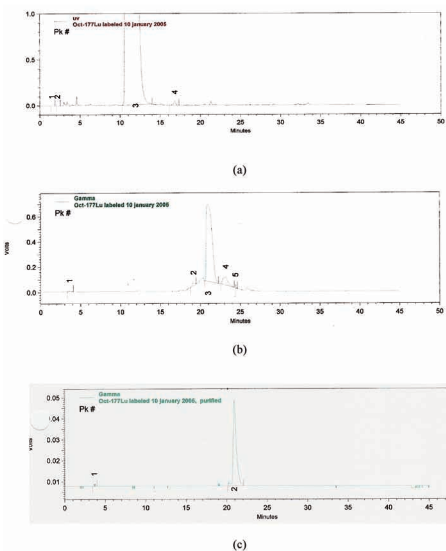
FIG. 16.7. HPLC purification of ^{177}\text{Lu} -OCT: (a) UV detection at 220 nm, (b) gamma detection of the labelling mixture and (c) control of the radiochemical purity of the radioreptide after further purification by SepPak.
