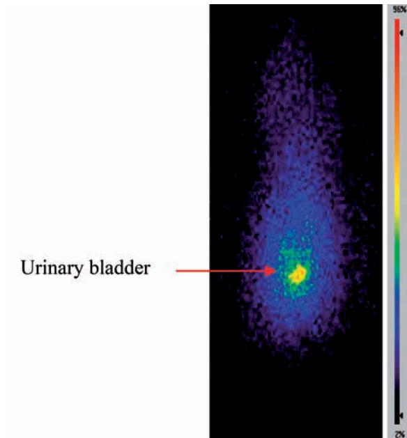
FIG. 7.10. Image of a healthy dog injected with 185 MBq of ^{90}\text{Y} -DOTATOC.
