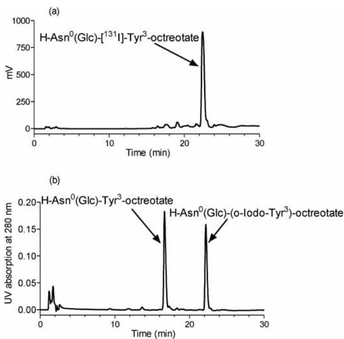
FIG. 6.4. (a)Radioactive and (b) UV absorption of ^{131}\text{I} -Sugar-TATE during HPLC analysis.
