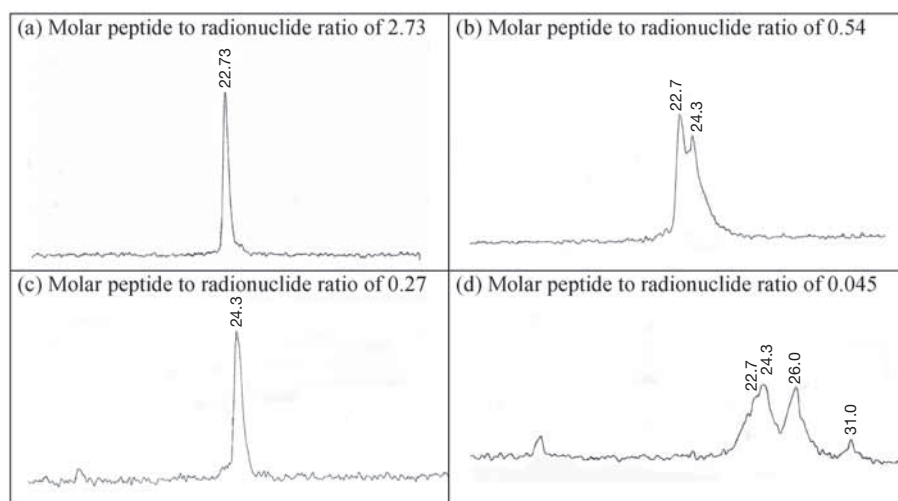
FIG. 3.1. HPLC profiles of [ ^{131}\text{I} ]DOTATATE using different molar peptide to radionuclide ratios (ethanol fraction of SepPak purification).
