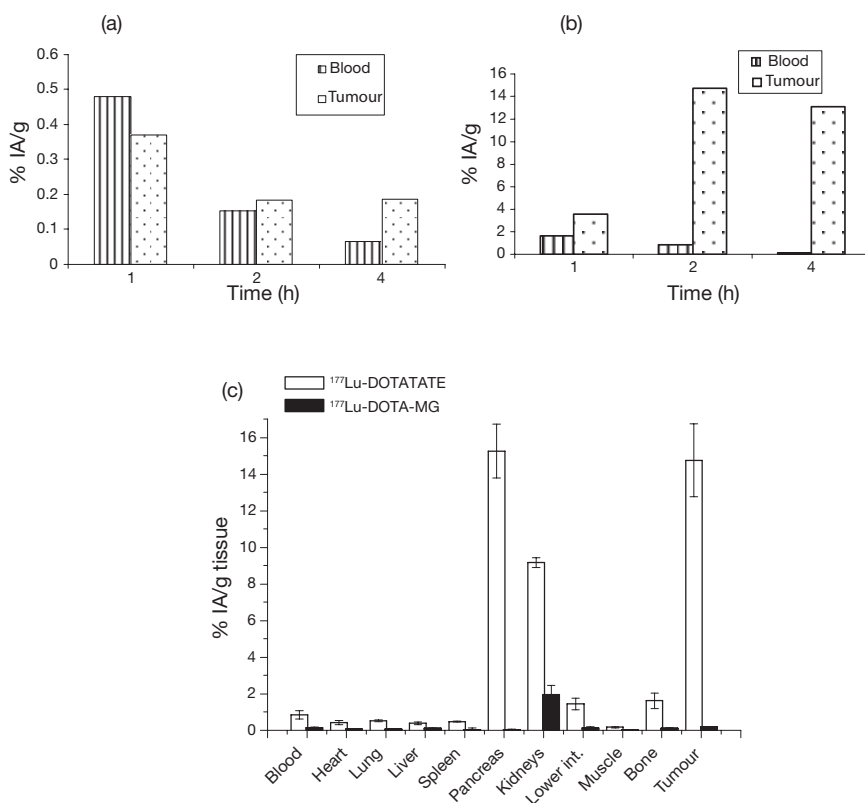
FIG. 11.3. In vivo tumour uptake of (a) ^{177}\text{Lu} -DOTA-MG and (b) ^{177}\text{Lu} -DOTATATE, and (c) biodistribution of both conjugates in athymic mice.
