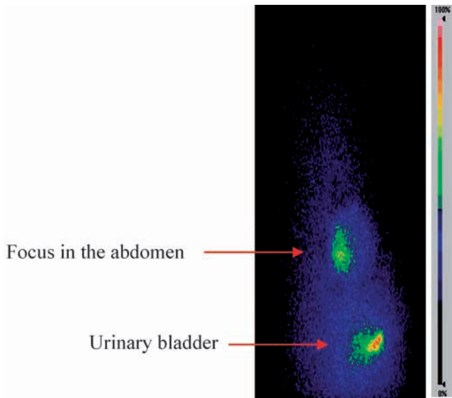
FIG. 7.11. Image of a dog with an insulinoma 4 h post-injection of 370 MBq of ^{90}\text{Y} -DOTATOC.
