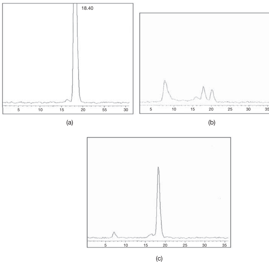
FIG. 3.2. HPLC profile of [ ^{177}\text{Lu} ]DOTATATE (a) immediately and (b) 48 h post-labelling using 200 \mu\text{g} of peptide and 140 mCi of radionuclide, and (c) 24 h after SepPak purification (ethanol fraction).
