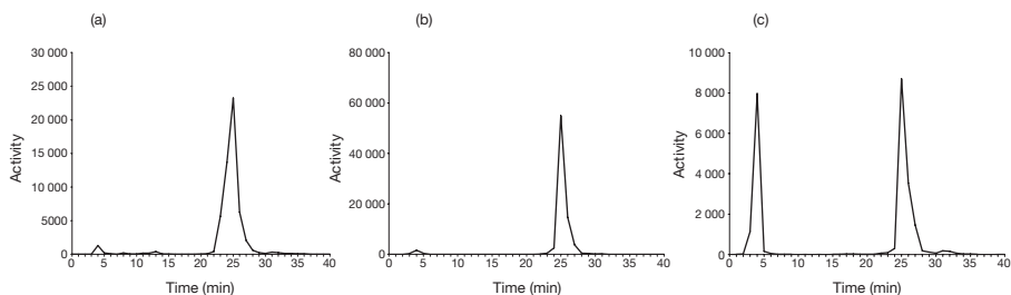
FIG. 5.7. HPLC analysis of urine after injection of ^{125}\text{I} -DOTATATE in rats: (a) standard, (b) 2 h post-injection and (c) 24 h post-injection.
