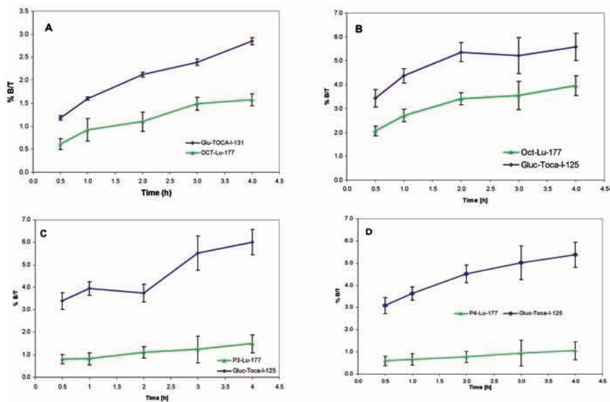
FIG. 16.8. Specific binding of (a) ^{177}\text{Lu} -OCT and ^{131}\text{I} -Gluc-TOCA, (b) ^{177}\text{Lu} -OCT and ^{125}\text{I} -Gluc-TOCA, (c) ^{177}\text{Lu} -P3 and ^{125}\text{I} -Gluc-TOCA and (d) ^{177}\text{Lu} -P4 and ^{125}\text{I} -Gluc-TOCA to D341 cells in paired assays, expressed as percentage of bound activity minus non-specific binding at 0.5, 1, 2, 3 and 4 h.
