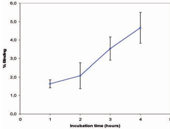
FIG. 16.3. Binding of ^{125}\text{I} -DOTATATE to whole AR42J cells calculated as percentage of activity corrected for non-specific binding in the presence of 26\mu\text{M} unlabelled peptide.
