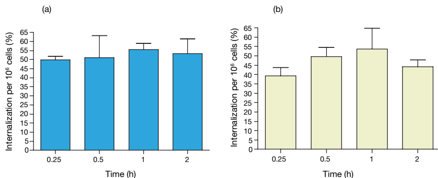
FIG. 3.5. Internalization of (a) [^{131}\text{I}]\text{DOTATATE} and (b) [^{177}\text{Lu}]\text{DOTATATE} into AR42J tumour cells.
