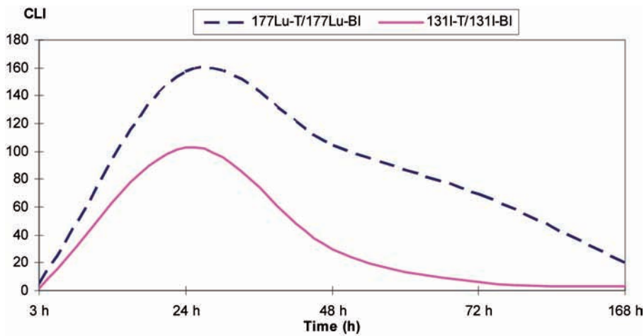
FIG. 14.9. Competitive uptake of ^{177}\text{Lu} -DOTATATE and ^{131}\text{I} -DOTATATE.
