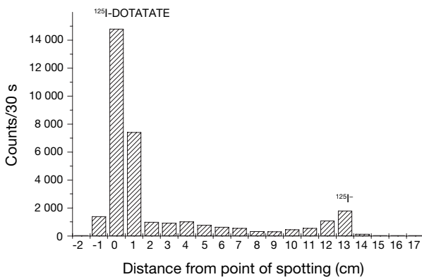
FIG. 8.10. Paper electrophoresis pattern of reaction mixture.
