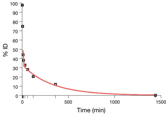
FIG. 7.18. Representative time versus blood activity curve for ^{99\text{m}}\text{Tc} -HYNIC-TATE in a dog with an insulinoma.
