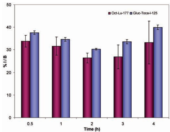
FIG. 16.9. Internalization pattern of ^{177}\text{Lu} -OCT and ^{125}\text{I} -Gluc-TOCA in D341 cells in paired assays, expressed as the percentage of internalized activity over specific bound activity at 30 min, and 1, 2, 3 and 4 h.
