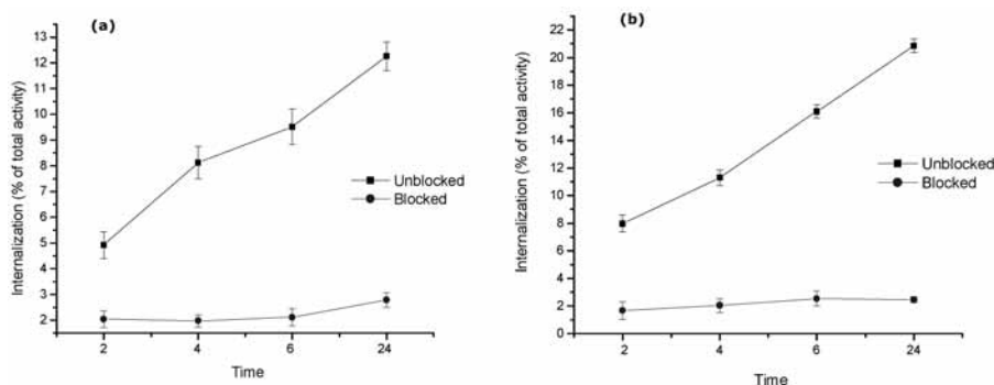
FIG. 11.5. Time dependent internalization of (a) ^{99m}\text{Tc} -EDDA/HYNIC-TOC in unblocked and blocked AR42J cells and (b) ^{99m}\text{Tc} -EDDA/HYNIC-[Lys 3 ]BN in blocked and unblocked PC3 cells, expressed as percentage of total activity (mean \pm sd, n = 3).
