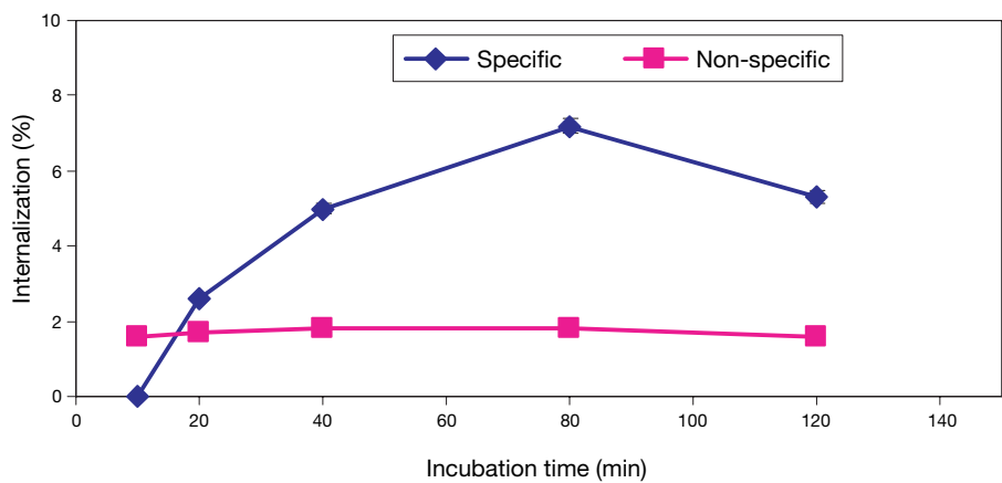
FIG. 12.2. Internalization of 177 Lu DOTATATE into AR42J cells.
