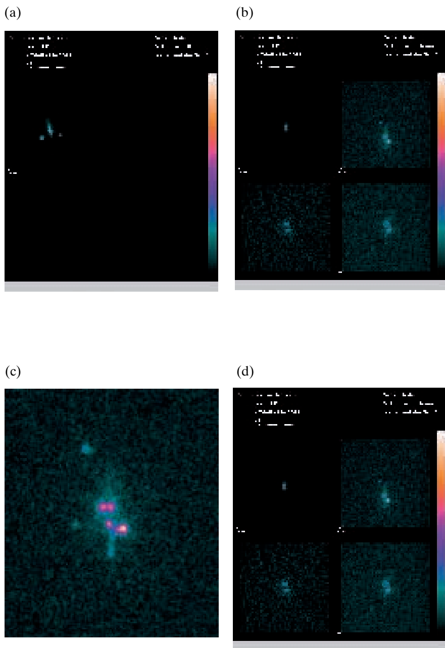
FIG. 8.8. Gamma scintigraphic images of a nude mouse bearing an HT-29 tumour at (a) 1, (b) 2, (c) 3 and (d) 18 h post-injection.
