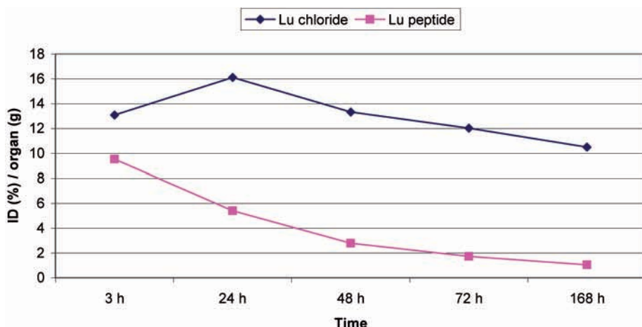
FIG. 14.8. Uptake of ^{177}\text{Lu} -DOTATATE and ^{177}\text{LuCl}_3 in bone.
