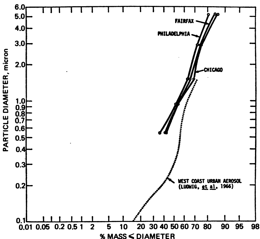
FIGURE 4-7 Cumulative particle size distributions of chloride in Chicago; Philadelphia; Fairfax, Ohio; and on the West Coast. (Reprinted with permission from Lee and Patterson. 242 )
