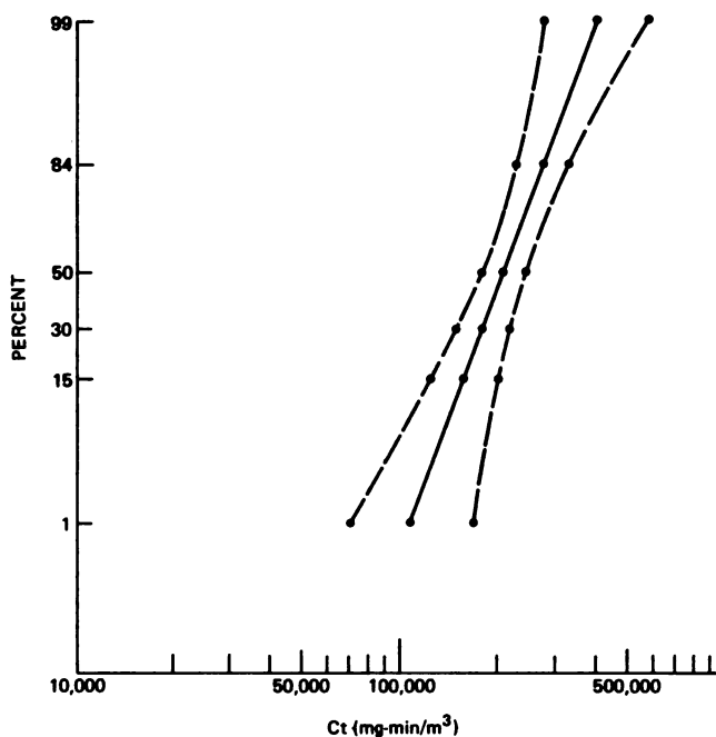
FIGURE 5-5 Lethal Ct's (mg-min/m 3 ) and 95% confidence limits of hydrogen chloride vapor to rats following total body exposure for 30 minutes.
