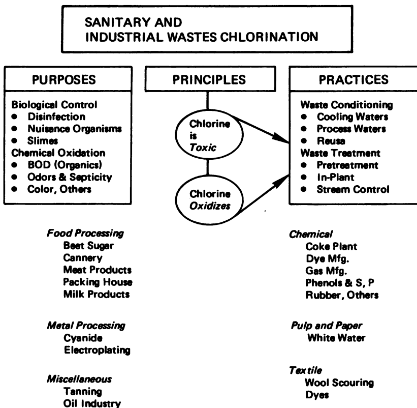
FIGURE 3-2 Typical applications of chlorine in waste treatment for resource conservation and pollution abatement. (Reprinted with permission from Laubusch. 239 )
