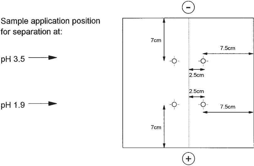
Fig. 2. Template for the application of samples to thin-layer chromatography plates. A transparent plastic sheet (e.g., acetate or overhead projection sheet) is cut to 20 cm × 20 cm. A series of circles is drawn, as indicated, using a permanent marker pen. This is placed over a light box and under the thin-layer chromatography plate, to allow application of the sample.
