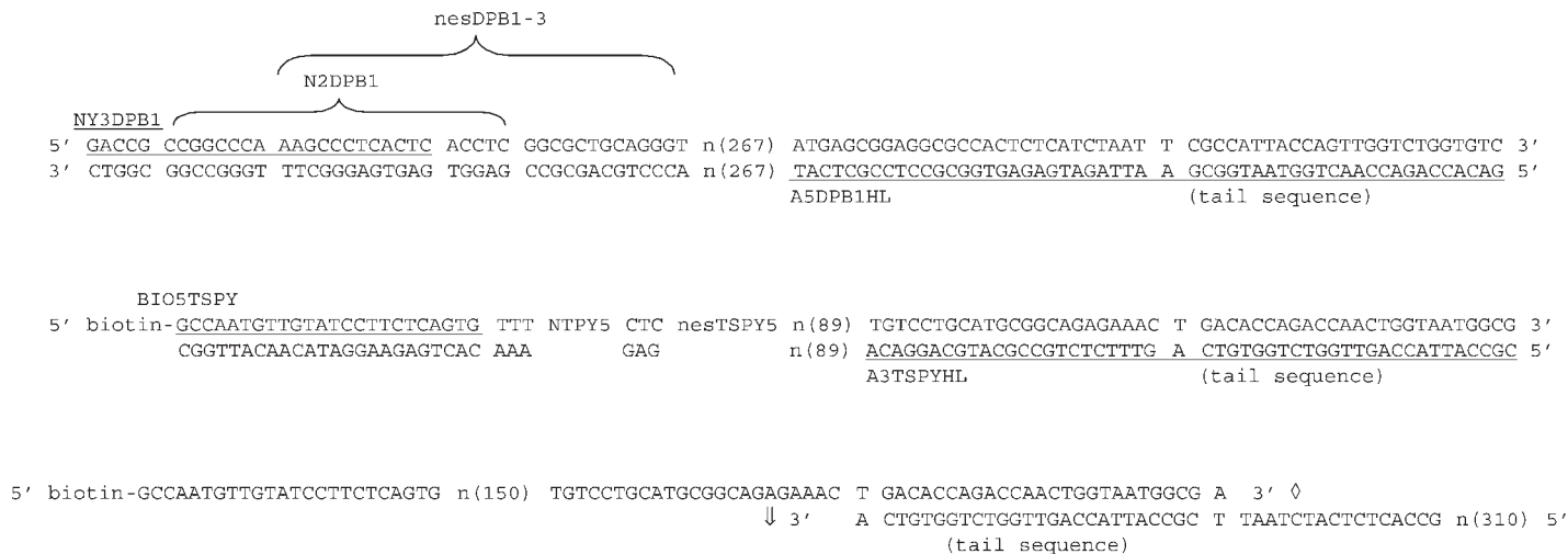
Fig. 1. Primer sequences and generation of a linked polymerase chain reaction (PCR) product. All primer sequences of the model system of the in-cell linker PCR principle are shown as parts of the two PCR products of HLA-DPB1 and TSPY , respectively, amplified in the first PCR step. Below is the formation of the linked PCR product illustrated ( n = number of nucleotides). An extra adenosine is included between the A5DPB1HL (or A3TSPYHL) primer sequence and the tail-linker sequence. This is because the Taq polymerase incorporates an adenosine on the 3' end of the new DNA strand.
