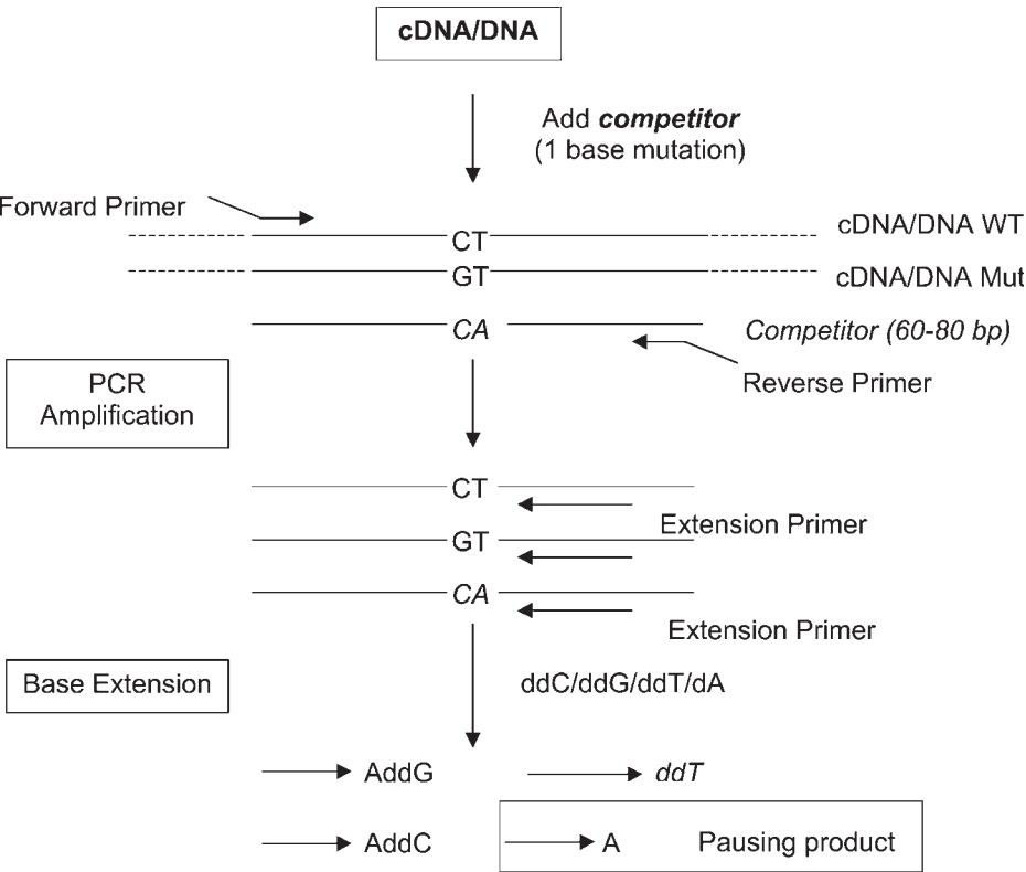
Fig. 2. Schematic representation of allele-specific quantification. When both the wild-type and the mutation DNA are present, the competitor is designed to have a synthetic mutation next to the natural mutation. Three extension products from the wild-type DNA, the mutant DNA, and the competitor are designed to have different molecular weights, and thus can be detected by matrix-assisted laser desorption/ionization time-of-flight mass spectrometry.
