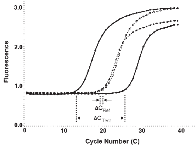
Fig. 3. Relative quantification by real-time polymerase chain reaction (PCR). (A) The amount of target in an experimental sample and a control sample are compared after PCR amplification and fluorescence monitoring at each cycle. For example, genomic DNA may be analyzed to assess gene amplification or deletion. Expression
