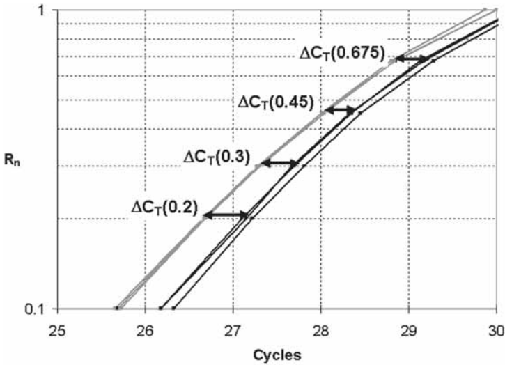
Fig. 2. Change in threshold cycle ( \Delta C_T ) in the amplification plot (magnification of Fig. 1). The \Delta C_T s of the four thresholds, indicated by double-headed arrows.
