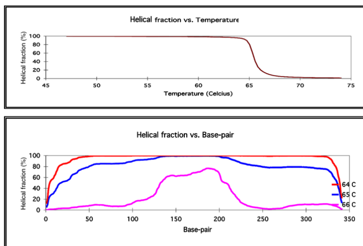
Fig. 2. The melting profile of exon 3 of the G6PT1 gene. The DNA sequence of the amplicon is: CTGCCCCATCTGACCCCACCCTCAacatgggcagtaggctggacacctacgtgtcgccctctgccacagtggttgagccatctcagtttggcacttgggtgggccatctgtcaaccagcatgaacctggctgg agg gctgggccctatcctggcaaccatcctggccagagctacagctggcgcagcacgctggccctatctgggcaactgtgtgtgtgtgtgtctctcctctgtctcctgtctatccacaatgaacctgctgatgttgactccgcaacctggaccccatgccctctgagggaagaagggtGAGCCCCCACCAGACCGACCACT. The uppercase letters are primer sequences. The letter in bold type is the nucleotide position of the mutation in the wild-type sequence, i.e., 1563G>A. The mutation is located at nucleotide position 136 of the amplicon. The sequence is shown in the sense of direction.
