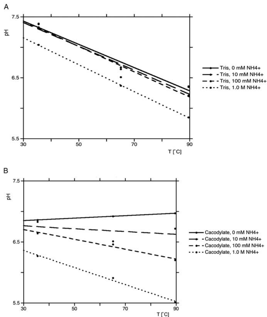
Fig. 25.3. (A) Temperature dependency of pH in Tris- or cacodylate-buffered solutions of \text{NH}_4\text{Cl} . Conditions: 50 mM Tris, pH 7.5 or 10 mM sodium cacodylate, pH 7.0 (100 mM NaCl, 0.5 mM EDTA).
