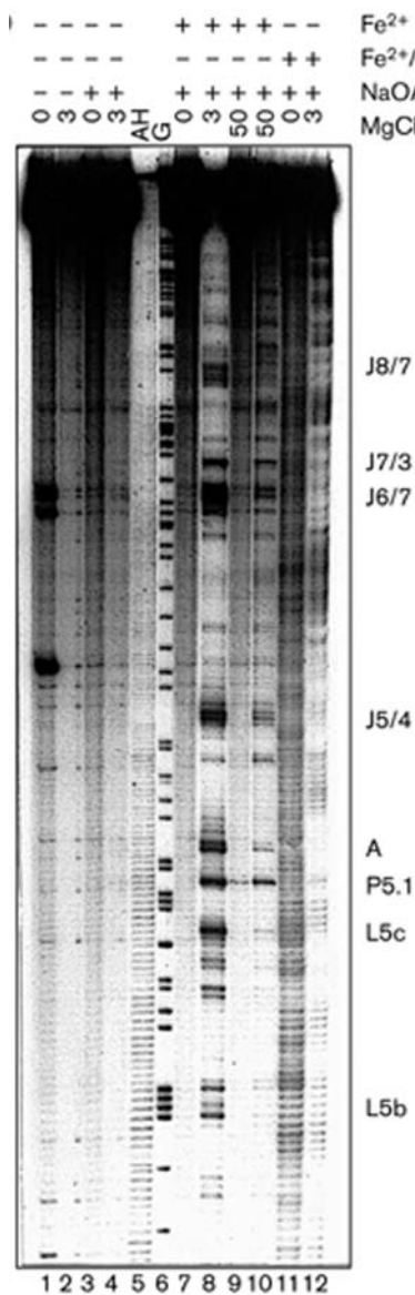
Fig. 15.1. Mapping the Fe 2+ cleavage sites in the Tetrahymena LSU group I intron. Autoradiogram of a 6% denaturing polyacrylamide gel with 5'-end-labeled Tetrahymena L-21 RNA cleaved with 10 \mu M Fe 2+ (lanes 7 and 9), 250 \mu M Fe 2+ (lane 8 and 10) or with 250 \mu M Fe 2+ /500 \mu M EDTA (lanes 11 and 12). Controls with untreated RNA (lanes 1 and 2) and in which Fe 2+ was omitted (lanes 3 and 4), as well as competition of Fe 2+ cleavage by 50 mM Mg 2+ (lanes 9 and 10) are
