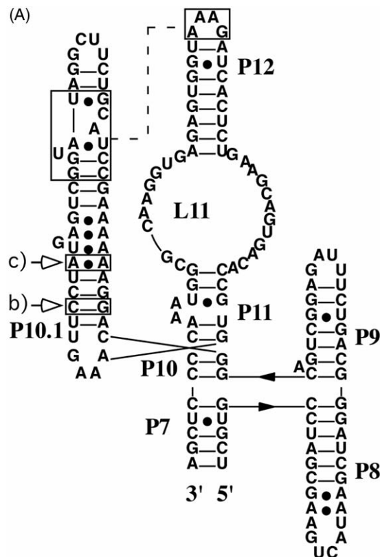
Fig. 32.2. Examples of covariance matrices taken from stem P10.1 in a subset of the S domain RNase P sequences related to the Bacillus subtilis type [35]. (a) Secondary structure of the S domain. Arrows point towards boxed base pairs that have been analyzed using the program coseq. For a base pair analysis coseq typically outputs 5 \times 5 covariance matrices corresponding to all nucleotide and gap combinations [(ACGU-) \times (ACGU-)] . The numbers in parentheses stand for the statistically expected occurrences of each pair calculated on the
