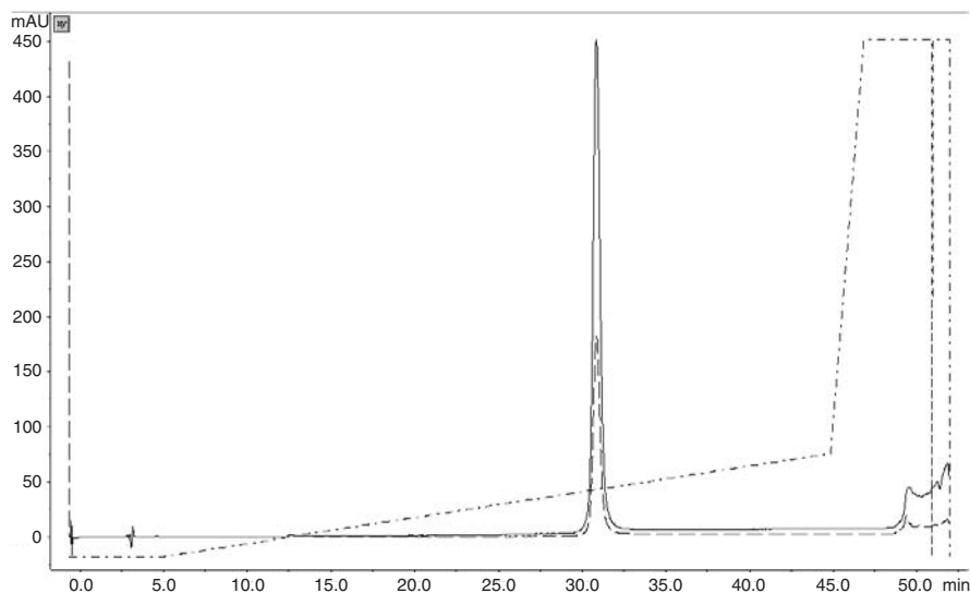
Fig. 7.6. Analytical reversed-phase HPLC trace of double HPLC-purified 27mer oligoribonucleotide run on a 5- \mu m XTerra™ RP 8 , 4.6 \times 250 mm column. The column was eluted with a linear gradient from 0–40% B
