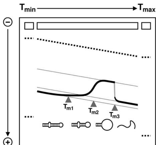
Fig. 24.1. Principle of TGGE. A linear temperature gradient is applied perpendicular to the electric field. The sample is applied to the long slot; small marker slots are on the left and right side of the gel. The mobility of an RNA with secondary structure is slightly decreased after a cooperative, reversible transition at T_{m1} , it is drastically decreased after a further transition at T_{m2} and it is increased after the irreversible transition at
