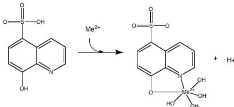
Fig. 16.1. The chemical structure of HQS binding to metal as seen in the nickel crystal structure [10]. The magnesium–HQS complex is assumed to have a similar structure.
