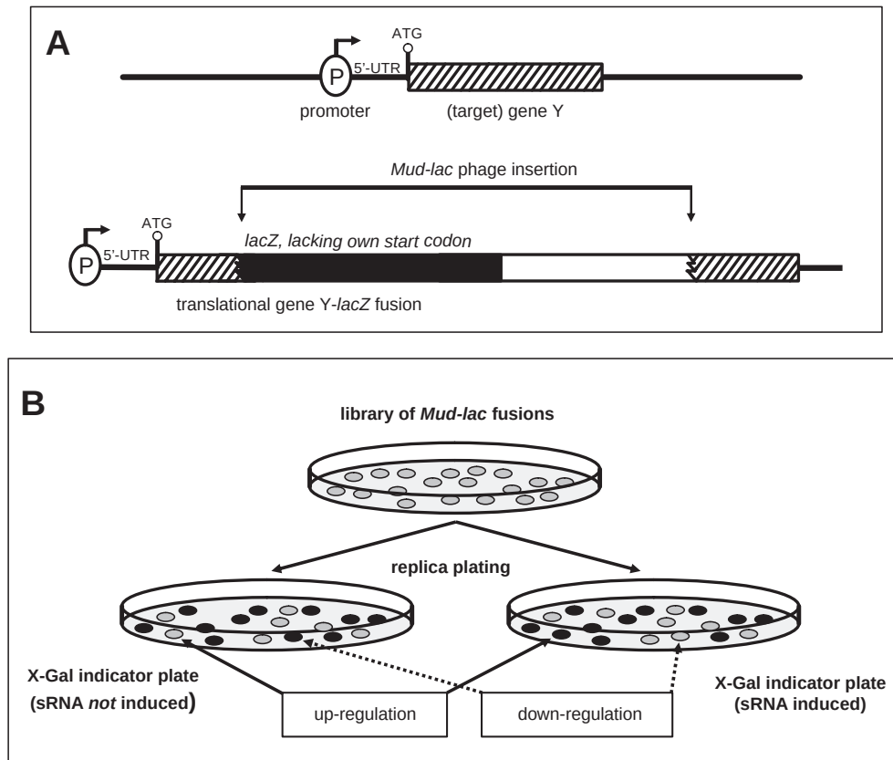
Fig. 37.1. Strategy for the identification of sRNA targets by reporter gene fusion. (A) A putative protein target gene (arbitrarily termed gene Y) of an sRNA is shown at the top, including its promoter (P), the 5'-untranslated region (5'-UTR) of its mRNA, the ATG start codon (open circle) and the coding region (hatched). One strategy to identify such an sRNA target gene is the use of engineered Mud-lac phages that carry a promoterless lacZ -coding region lacking a ribosome-binding site and start codon immediately adjacent to one end of the phage sequence, oriented "inwards". Random Mud-lac chromosomal insertion events which have resulted in in-frame fusion of a gene Y 5' segment and the lacZ -coding region (A, lower panel) then permit to monitor sRNA-mediated effects on transcription, translation and stability of the target Y mRNA. (B) Analysis of sRNA effects using a library of transcriptional/translational Mud-lac fusion insertions; the strain in this
