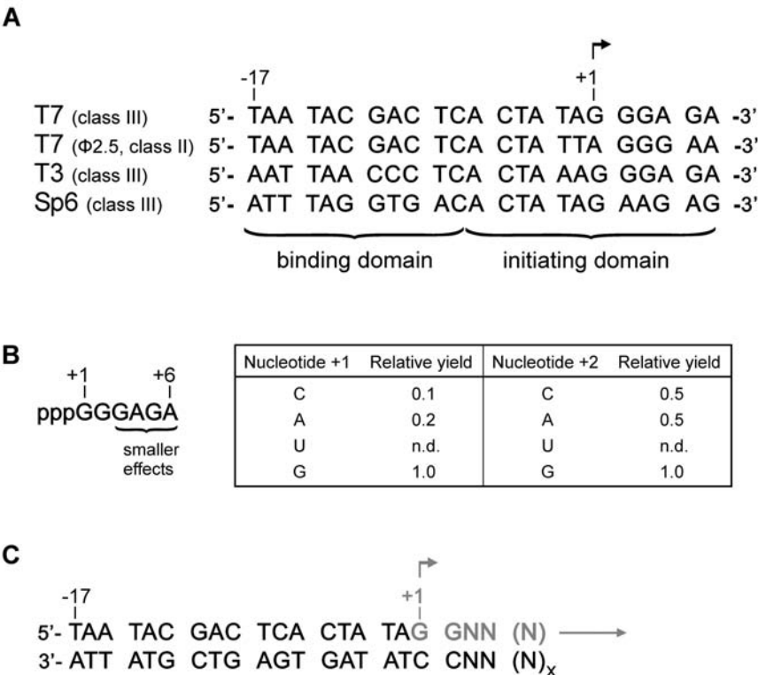
Fig. 1.1. (A) Consensus sequences of class III promoters of bacteriophages T7, T3 and SP6, and sequence of the T7 \phi 2.5 class II promoter [5, 34–36]. Phage polymerase initiating domains also include the first 5–6 nt of the transcribed template strand. The transcription start (position +1) is indicated by the arrow. The phage T7 genome encodes a total of 17 promoters, including five class III promoters and one replication promoter ( \phi OR), which are all completely conserved in the region from nt –17 to +6. In addition, there are 10 T7 class II promoters plus one more replication promoter ( \phi OL); among these 11 promoters, which display some sequence variation within the –17 to +6 region, only the \phi 2.5 and \phi OL promoter initiate transcription with an A instead of G residue [35] (B) Effect of sequence variations in the +1 to +6 region of the T7 class III promoter on transcription efficiency (adapted from Milligan and Uhlenbeck [7]); n.d.: not determined. (C) T7 class III promoter region with the recommended G identities at positions +1 and +2 of the RNA transcript shown in grey.
