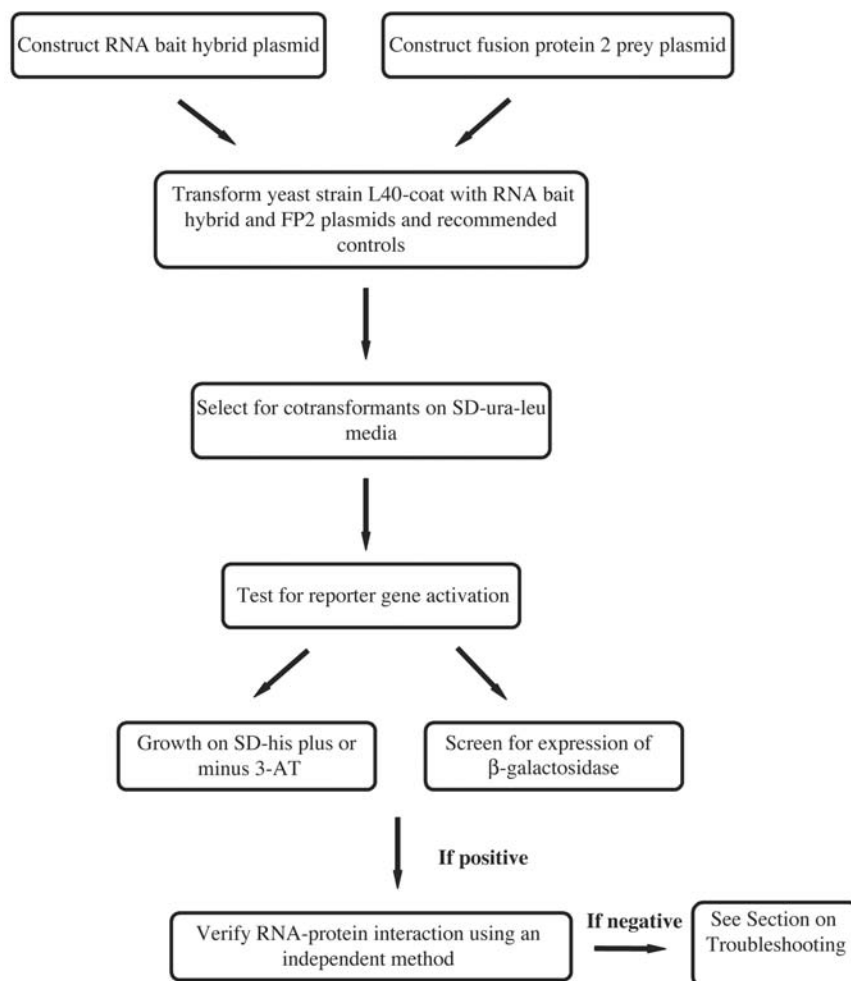
Fig. 45.3. Experimental outline of three-hybrid protocol.
