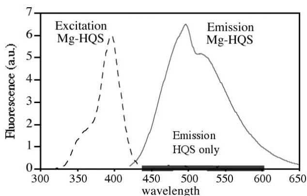
Fig. 16.3. The excitation and emission spectra of \text{Mg}^{2+} -HQS with the emission spectra of HQS shown as a reference. The spectra were collected on an Amico-Bowman Series 2 spectrometer (ThermoSpectronic, Rochester, NY) by exciting the fluorophore at 397 nm. The slit width for both excitation and emission spectra was kept at 8 nm. The sample was placed in 0.1 M Tris, pH 8, 2 mM HQS and with or without 1 mM magnesium at 25 °C.
