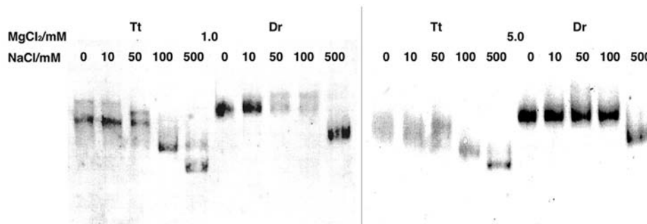
Fig. 25.7. Native gel electrophoresis (5% polyacrylamide). Tt and Dr RNase P RNA has been annealed in 10 mM sodium cacodylate, pH 7, 0–500 mM NaCl before addition of 1.0 (left) or 5.0 mM (right) \text{MgCl}_2 .
