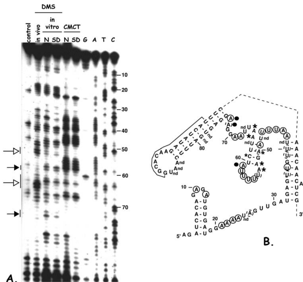
Fig. 10.2. Chemical probing on S. aureus RNAIII performed in vivo and in vitro (A), and part of the secondary structure of S. aureus RNAIII (B). (A) DMS and CMCT modifications were performed in vitro under native conditions (N) and semi-denaturing conditions (SD), and in vivo for DMS. Experimental details are given in the text. (Control) incubation control; (lanes G, A, T, C) DNA sequencing ladders. (B) Circled nucleotides are reactive towards DMS
