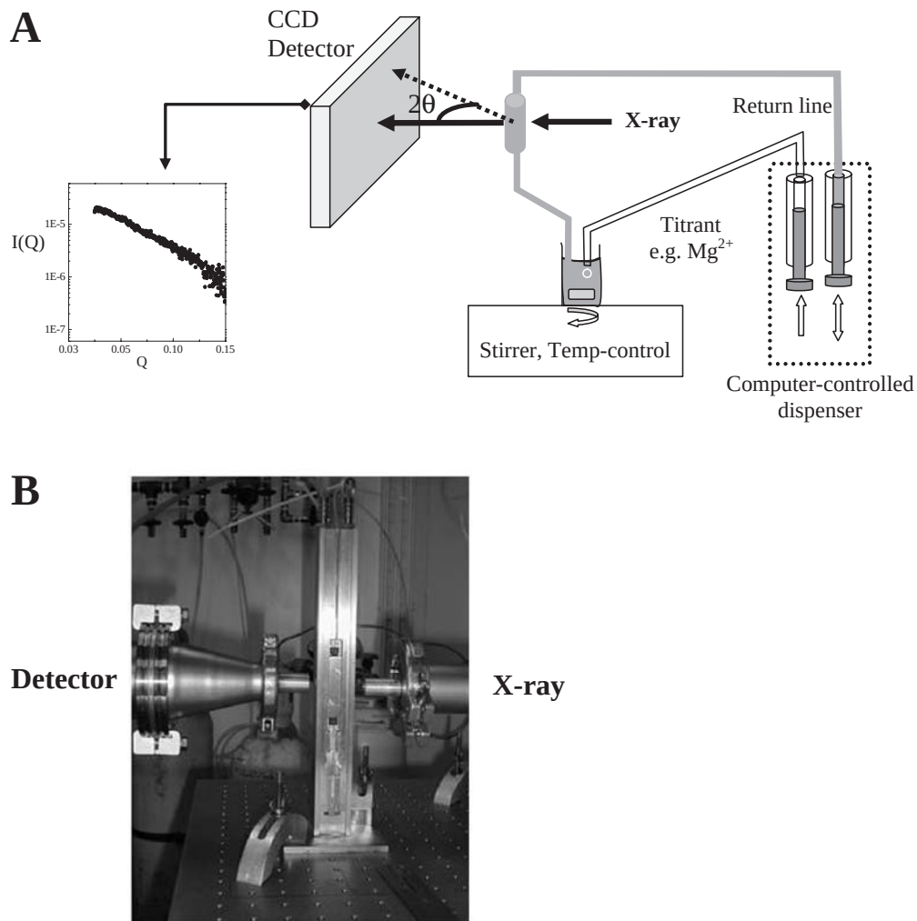
Fig. 23.2. (A) Experimental setup of SAXS at a synchrotron facility. (B) The sample holder used in our SAXS studies, sandwiched between the X-ray beam on the right and the CCD detector on the left.
