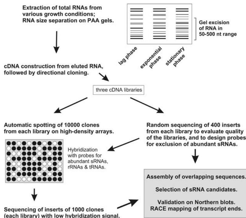
Fig. 36.2. Flow chart of the RNomics screen in E. coli as published by Vogel et al. [54]. See text for a more detailed explanation of the individual steps. For experimental details on RNomics, see Chapter 38.
