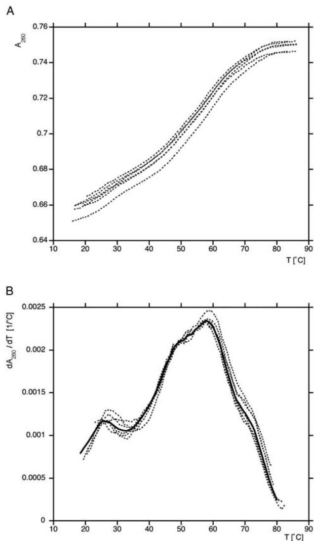
Fig. 25.1. UV melting profile of an RNase P RNA annealed in 10 mM sodium cacodylate pH 7, 10 mM NaCl and 0.5 mM \text{MgCl}_2 . (A) Absorbance melting curve, three subsequent
