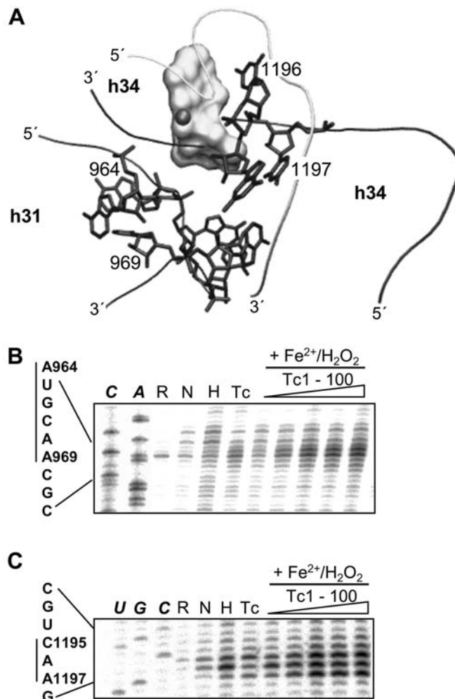
Fig. 15.3. Fe 2+ -mediated hydroxyl radical cleavage of the 16S rRNA. (A) Surface structure of tetracycline complexed with Mg 2+ (shown as a grey sphere) bound to the ribosomal binding site-1 which is formed by helix 34 (h34) and the internal loop of helix 31 (h31 [57]). The phosphodiester backbones of RNA strands containing bases that are attacked by hydroxyl radicals are shown as closed black ribbons, the unaffected backbone strand is shown as a light grey ribbon. Residues that are cleaved by Fe 2+ are shown as black sticks. Bases 964, 969, 1196 and 1197 are marked for orientation. Coordinates were taken from the RCSB entry 1197 [57]. (B) Autoradiograph of a polyacrylamide gel showing cleavage sites in the internal loop of
