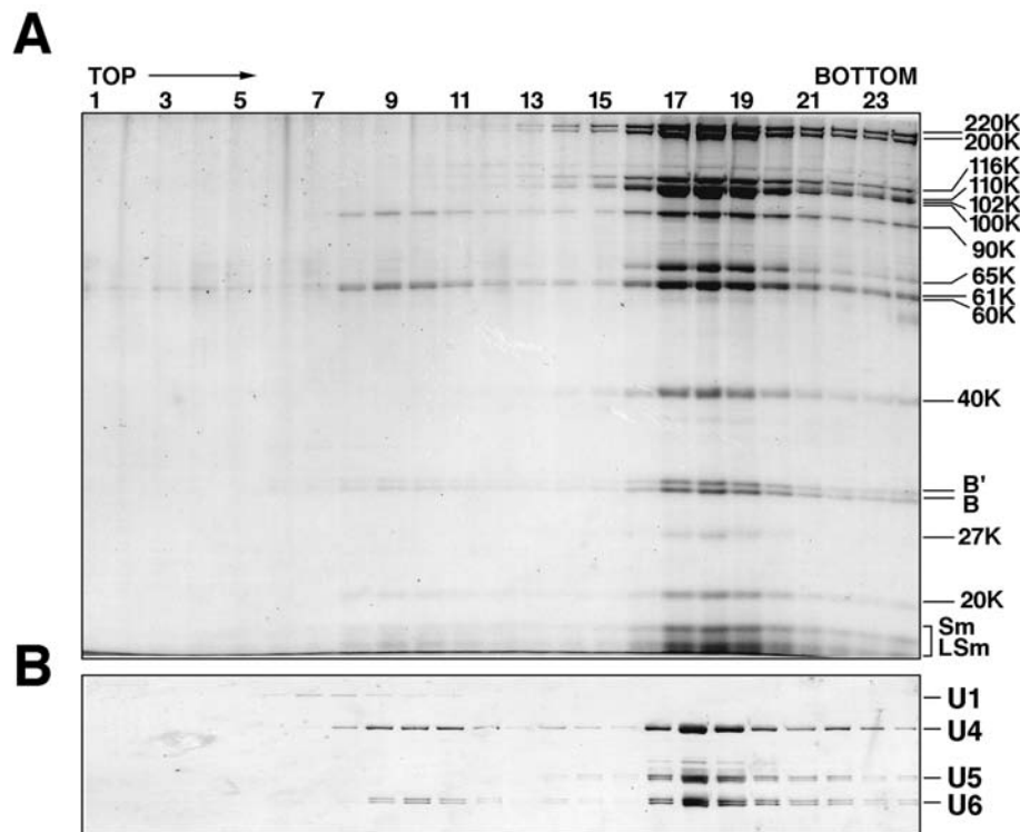
Fig. 42.1. Immunoaffinity-purified 25S U4/U6.U5 tri-snRNPs. Human 25S U4/U6.U5 tri-snRNPs were isolated from a mixture of anti- m_3G purified, HeLa spliceosomal snRNPs with anti-peptide antibodies against the U4/U6 61K protein and subjected to 10–30% glycerol gradient centrifugation. Distribution of (A) protein and (B) snRNA across the gradient. Proteins were separated by SDS-PAGE and visualized by staining with Coomassie. RNA was fractionated by denaturing PAGE and stained with silver. Gradient fraction numbers are indicated at the top and the identities of tri-snRNP proteins are shown on the right.
