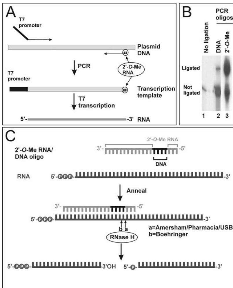
Fig. 3.3. (A) Production of T7 transcripts with homogeneous 3' ends. The template for T7 transcription is produced by PCR. The upstream primer contains a promoter for T7 RNA polymerase, while the downstream primer contains two 2'-O-methyl RNA residues at the 5' end of the oligonucleotide. Both primers are incorporated into the PCR product and during transcription with T7 RNA polymerase, the 2'-O-methyl RNA residues prevent the addition of non-template nucleotides to the 3' end of the RNA molecules. (B) Comparison of the ligation efficiencies when a standard DNA oligonucleotide and a hybrid DNA/2'-O-Methyl RNA oligonucleotide (depicted in panel A) were used as the downstream primer in the
