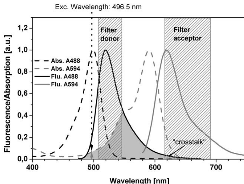
Fig. 28.1. Donor (Alexa 488) and acceptor (Alexa 594) spectra are shown. FRET occurs if the donor emission overlaps with the acceptor absorption; illustrated here by the grey area. Fluorescence detection with different filters allows detection of donor and acceptor
