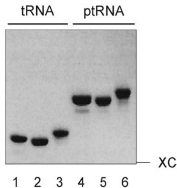
Fig. 6.2. Denaturing 9% polyacrylamide gel showing a \text{tRNA}^{\text{Gly}} (79 nt, lanes 1–3) and its 93-nt precursor (lanes 4–6) – both with homogeneous 3' ends due to release from a primary transcript carrying a 3'-terminal cis -hammerhead – after hammerhead self-removal and gel purification (lanes 2 and 5), after subsequent 3' dephosphorylation (lanes 1 and
