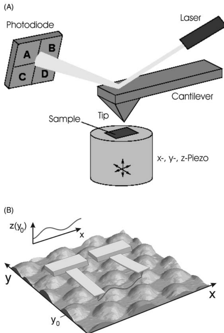
Fig. 29.1. (A) The principle of the scanning force microscope: see text for details. (B) Scanning of a 3-D surface. The cantilever is moving in the x -direction across the sample,
