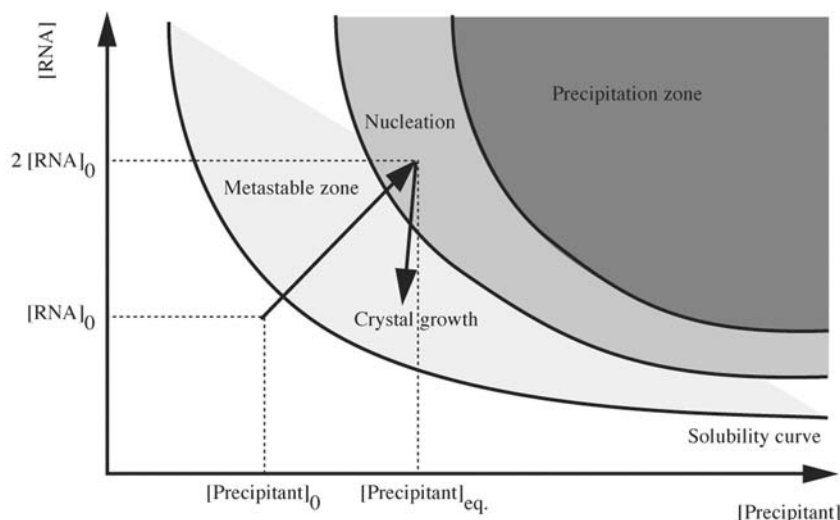
Fig. 27.1. Solubility diagram. During equilibration, the concentration of both precipitant and macromolecule increase until precipitation occurs. The formation of crystal
