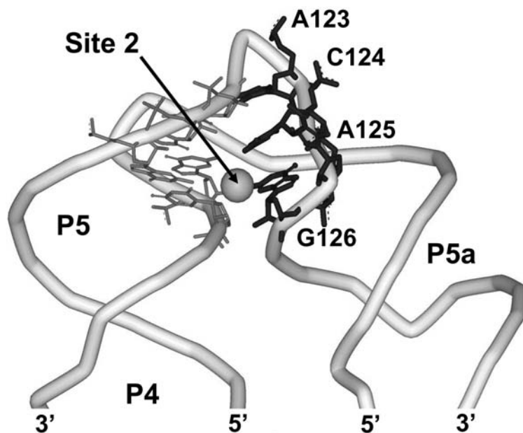
Fig. 15.2. Correlation between a computationally predicted \text{Mg}^{2+} -binding site and \text{Fe}^{2+} cleavage sites in the Tetrahymena P4P6 domain. The phosphodiester backbones of the two RNA strands in the hinge region of the P4P6 domain of the Tetrahymena LSU group I intron are shown as closed white ribbons with their polarity and the secondary structure
