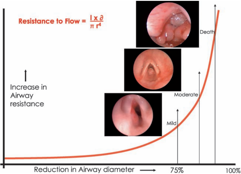
Fig. 21.1 Illustration showing the rapid rise in airway resistance with reducing airway diameter, as dictated by Poiseuille's law
