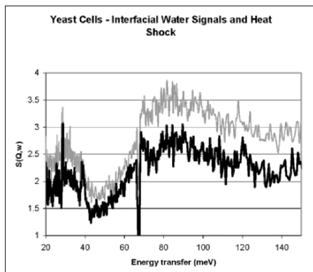
Figure 6. Effect of heat shock on the interfacial water signal and content in yeast cells. Bottom trace – yeast cells (control). Upper trace – yeast cells after heat shock at 323 K. The signals are normalized to the total water signal. The spike at 67 meV is an artefact remaining after subtraction of the bulk water signal due to small errors in the time-of-flight measurement between different runs.
