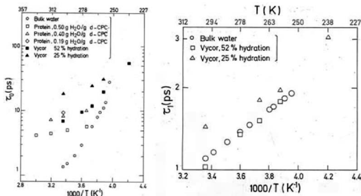
Figure 8. (a) (left side) Arrhenius plot of the residence Time \tau_0 for bulk water and for hydrated Vycor and C-phycocyanin protein.
