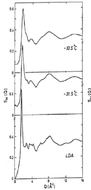
Figure 1. Structure factors S_M(Q) of supercooled \text{D}_2\text{O} , at normal pressure, as compared with that of low-density amorphous ice (LDA) at 77 K. 29
