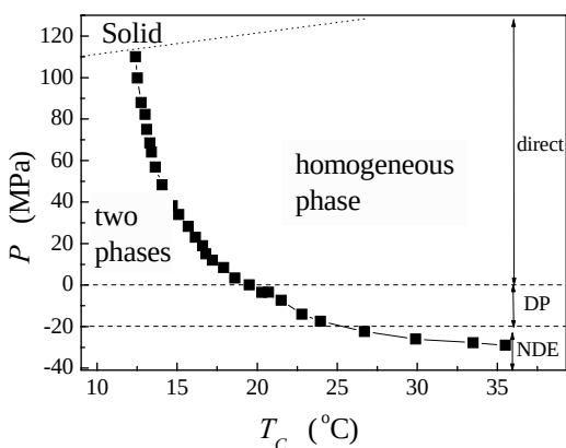
Figure 4. Liquid-liquid locus of nitrobenzene/n-hexane mixture (0.43 mole fraction of nitrobenzene). From 0 to 110 MPa the data was obtained directly, from -20 MPa to 0 by the extrapolation of Dielectric Permittivity (DP), and below -20 MPa by extrapolation of nonlinear dielectric effect.
