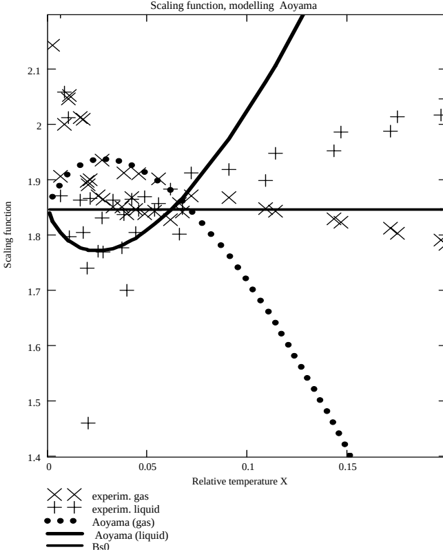
Figure 2. The scaling function for R236ea. X = \tau^{1-\alpha-\beta} Aoyama, gas – \psi_g calculated with Model 12 ; Aoyama, liquid – \psi_l calculated with Model 12 ; B_{s0} – a leading amplitude.
