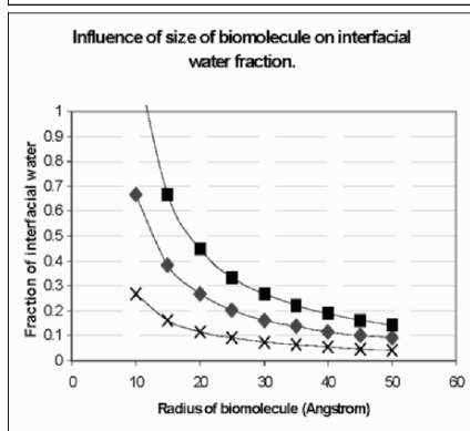
Figure 2. Theoretical calculation of the interfacial water as a fraction of total water in a cell at 300 mg/ml protein and with a cylindrical-shaped protein of mass 50 kDa. The radius of the hypothetical protein is allowed change from 2.5 to 27.5 Å, hence changing its shape to a thin rod at low values for the radius. The three curves show calculations for one, two, and three shells of interfacial water molecules (filled squares, squares and triangles respectively).
