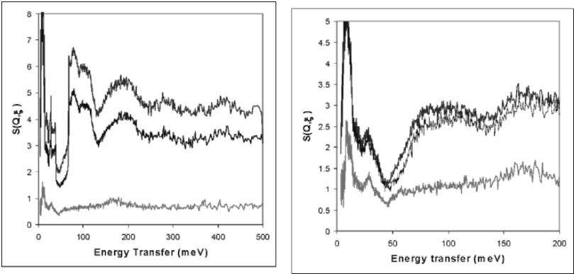
Figure 7. (Above left) IINS data in the 1–500 meV energy transfer range for E. coli cells: dry (bottom/gray), control cells (center), and after 2.5OsM hypertonic shock (upper trace). (Above right) after subtraction of the bulk water signal (same sequence of traces).
