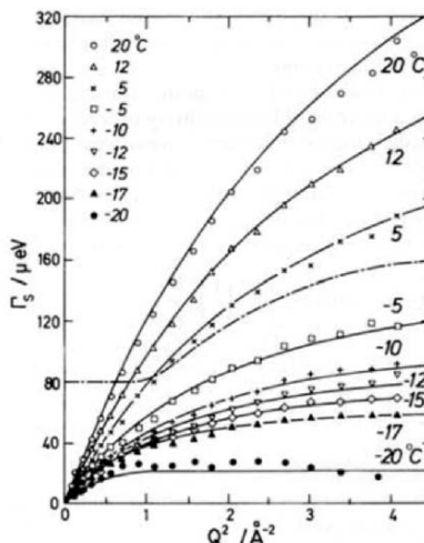
Figure 7. Linewidths of the quasi-elastic incoherent neutron scattering of bulk water at different temperatures. 40 The solid lines are the resulting fitting with the random jump diffusion model. 39 The plateau at large Q is proportional to the residence time of the molecules. The dashed line represents the Lorentzian linewidth for water bound to C-phycocyanin at room temperature. 41
