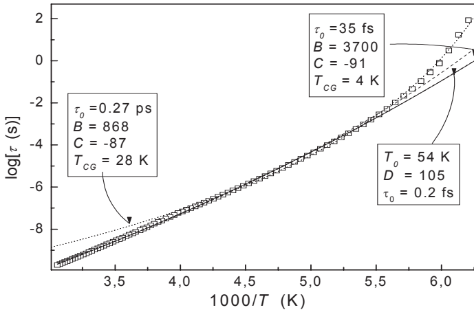
Figure 11. The Arrhenius plot of dielectric relaxation time. Black solid curve shows the single VFT fit results function. The dotted and dashed–dotted curves portray the Cohen–Grest function, based on low- and high-temperature data respectively. Fitted parameters, according to relations (1) and (4), are given in the figure.
