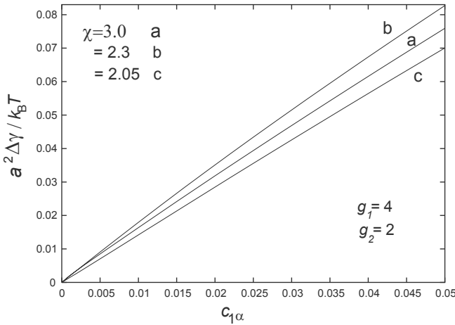
Figure 3. Normalized excess surface tension a^2 \Delta\gamma/k_B T vs the normalized ion density c_{1\alpha} in phase \alpha .
