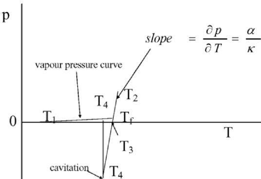
Figure 7. The change of pressure in a Berthelot tube by changing the temperature.
