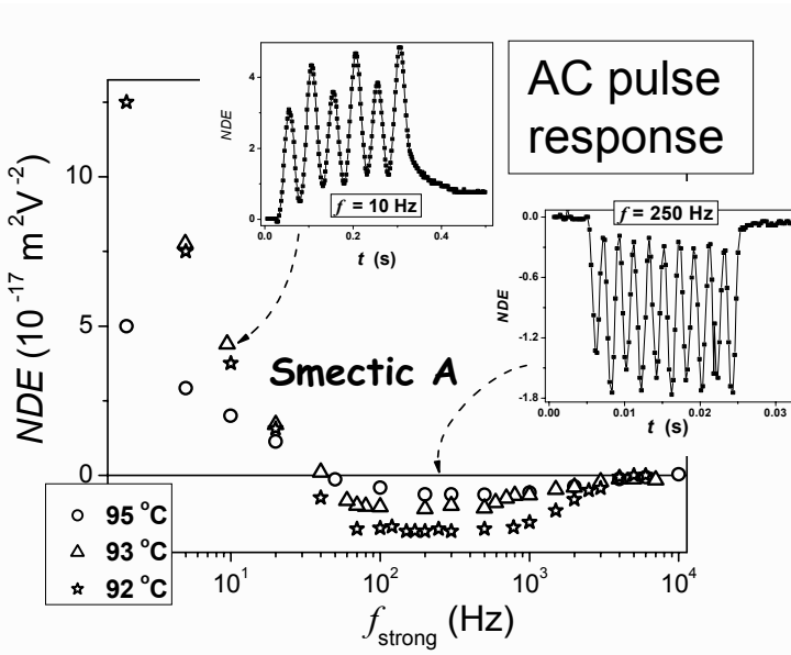
Figure 6. Basic results for the frequency selective NDE studies in SmA phase of DOBAMBC, on approaching SmC* ferroelectric mesophase. Insets show nonlinear dielectric responses associated with sine wave pulses of different frequencies, given in presented plots.
