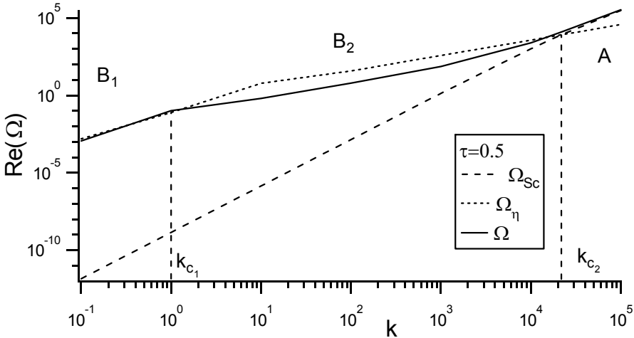
Figure 7. The damping rate for nematic–non-nematic mixture for \tau = 0.5 . The general dispersion relation (continuous curve), the inner region dispersion relation (dashed line), and the outer region dispersion relation (dotted curve).
