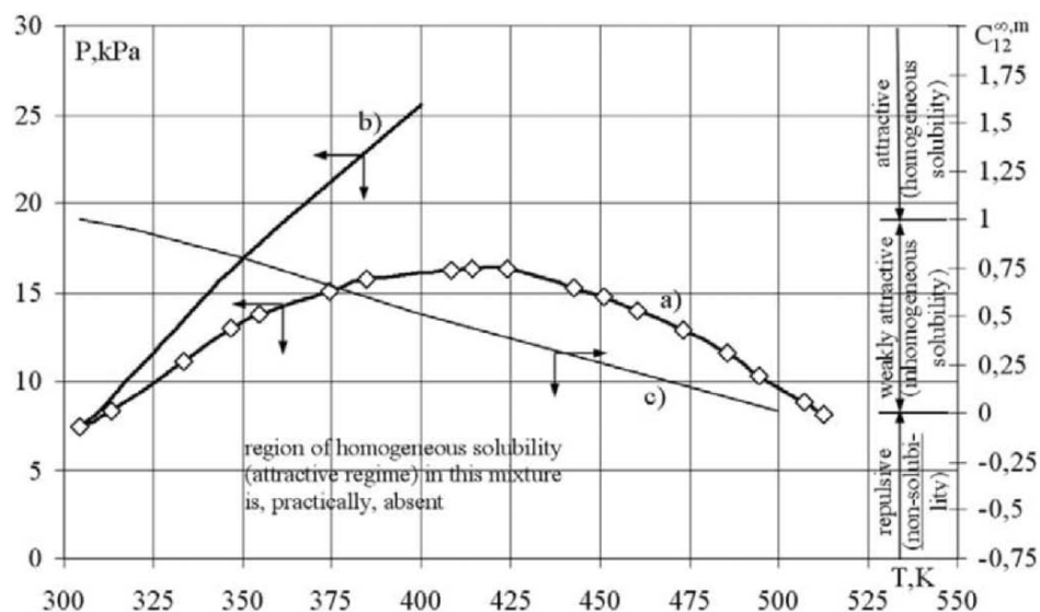
Figure 5. LPD of binary mixture SCF(CO 2 )–cosolvent (CH 3 OH): a) critical curve P^c(T) ; 14 b) maxima-of-pressure curve P^m(T) , corresponding to the best miscibility of components; c) decreasing of methanol solubility in carbon dioxide with temperature increasing.
