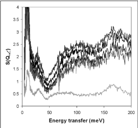
Figure 8. Osmotic effect on the interfacial water IINS signal associated with yeast cells: From bottom to top: dried yeast cells; 25 mOsM; 0.3 mOsM; 1.25 OsM; and 2.5 OsM.
