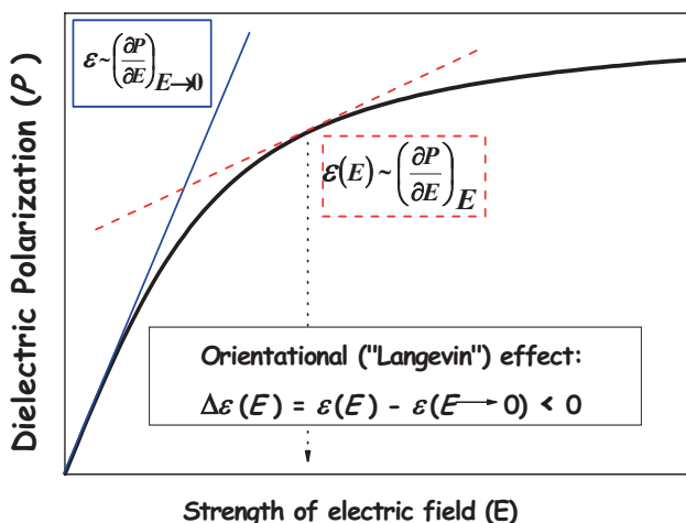
Figure 1. The behavior of dielectric polarization when increasing the intensity of a strong electric field. The value of NDE is determined by the difference of slopes of the dashed and the solid line. 1–3
