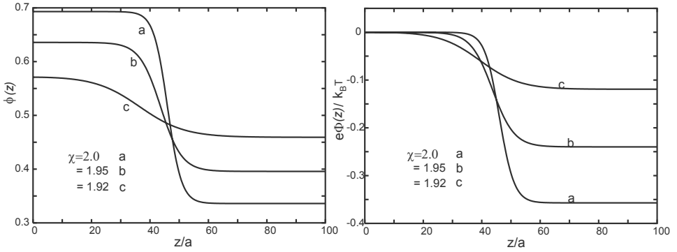
Figure 1. Composition \phi(z) (left) and normalized electric potential e\Phi(z)/k_B T (right) near an interface with varying \chi = 2, 1.95 , and 1.92 for g_1 = 4 , g_2 = 2 , and \sqrt{n_{1\alpha} n_{1\beta}} = 0.01a^{-3} .
