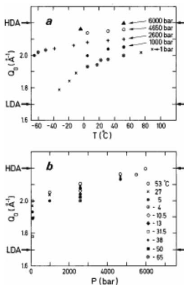
Figure 5. Evolution of the main diffraction peak position Q_0 of the structure factor (a) at constant pressure as a function of temperature and (b) at constant temperature as a function of pressure.
