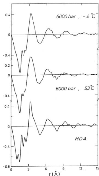
Figure 6. Pair correlation functions d_L(r) of liquid D_2O , under 6000 bar, as compared with that of high-density amorphous ice (HDA) at 77 K. 30
