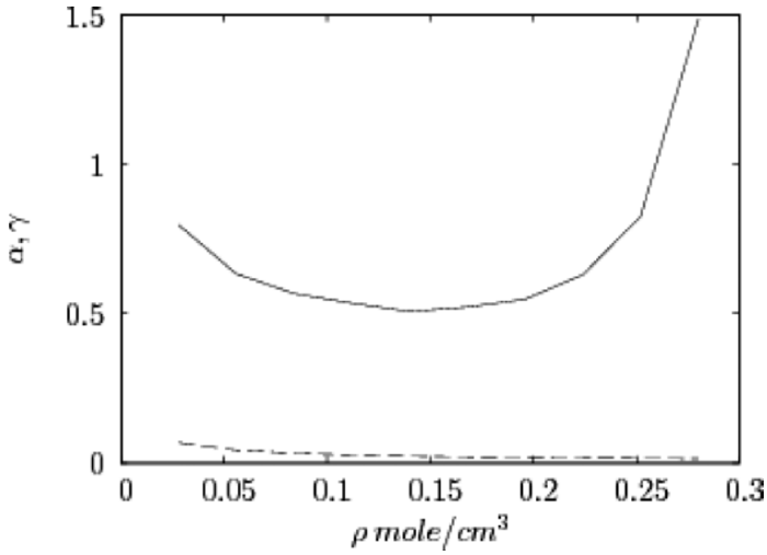
Figure 7. The density dependence of the nearly free electrons model applicability criterion and degeneracy parameter at the temperature T = 3000 K.
