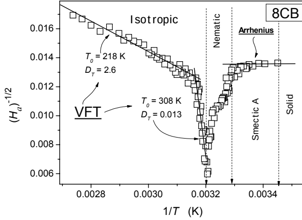
Figure 2. The linearized, derivative-based transformation of dielectric relaxation data from focused on the validity of the VFT relation in the description of dynamics in 8CB (see relations (1) and (2)). All parameters given in the figure were determined from the linear regression analysis as discussed below relation (2) and derived in Ref. 15.
