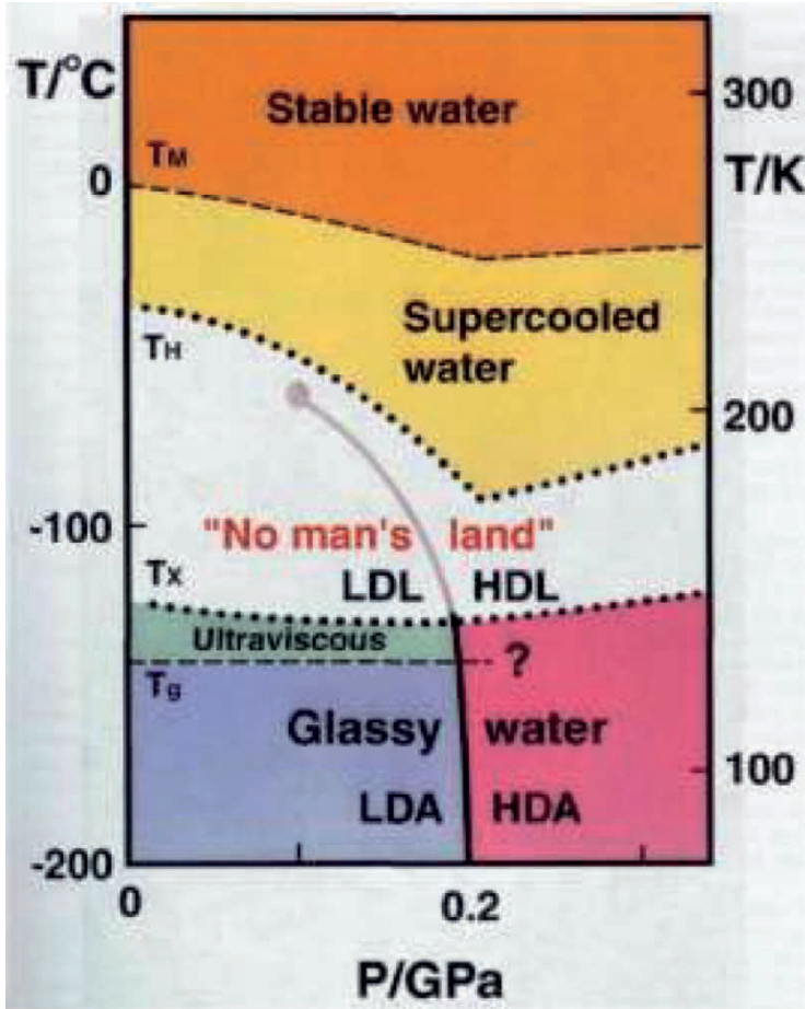
Figure 1. Phase diagram of liquid water. The liquid–liquid critical point lies in the experimentally inaccessible “no man’s land.” Courtesy of O. Mishima.
