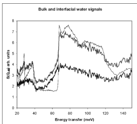
Figure 3. Examples of IINS spectra for bulk water (ice Ih – noise-free upper line), interfacial water (noisy lower line), and a sample displaying a mixture of bulk and interfacial water (noisy upper trace). Note that the very sharp edges in the bulk water spectrum at 67, 28, and 37 meV are absent from the interfacial water spectrum.
