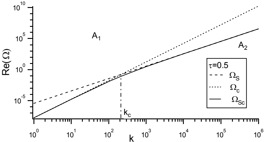
Figure 5. The inner region (leading-order) damping rate (continuous curve) for polymer–nematic mixture, defining two distinct regimes. The non-conserved order parameter dispersion relation (dashed curve) and conserved parameter dispersion relation (dotted curve). In the region A_1 relaxation of the concentration is the important process, while in the region A_2 relaxation of the orientational order parameter dominates.
