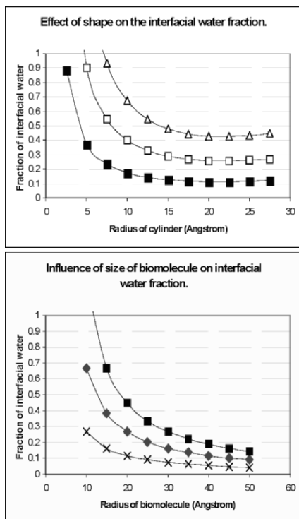
Figure 1. Theoretical calculation of the interfacial water component in a cell as a fraction of the total water at 300 mg/ml protein, and with spherical proteins of variable radius. The three curves show calculations for one, two, and three shells of interfacial water molecules (crosses, diamond and squares respectively).
