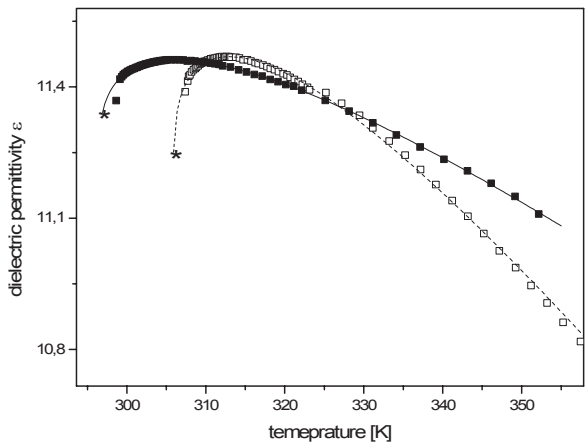
Figure 2. Temperature dependence of dielectric permittivity measured at 10 kHz for bulk 5CB (open) and mixture with Aerosil (solid). Curves are parameterized by relation (1).
