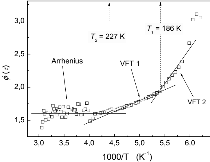
Figure 12. Stickel-plot of the temperature dependence of dielectric relaxation time. The sloped lines reveals regions described by two different VFT functions (Eq. (1)) while the non-sloped lines indicates the Arrhenius behavior (Eq. (2)).
