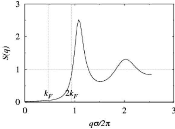
Figure 4. The pair structure factor of the ion subsystem. Two vertical lines denote the values of the wave vector equal to k_F and 2k_F correspondingly. These values correspond to \sigma = 4 \text{ a.u.} and \eta = 0.45 .
