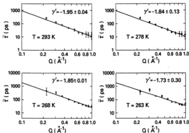
Figure 11. Average relaxation time \bar{\tau} [defined in Eq. 10] for the 100% hydrated sample plotted against Q in log-log scales. It can be seen that the slope is approximately -2 at room temperature.
