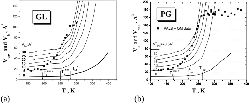
Figure 10. Mean cavity volumes, calculated from Eq. (4) for several cases of V_{\text{lim}} , together with the experimental mean hole volumes (points) from PALS for GL (a) and PG (b).
