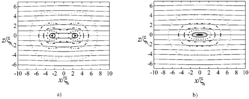
Figure 6. Smectic layer profile with contour plot of \eta(x,z) superimposed at different stages during the annihilation process. Contours correspond to \eta/\eta_b = 0.95, 0.8, 0.6, 0.4, 0.2, 0.05 . (a) d=5\xi , and (b) d=0 .
