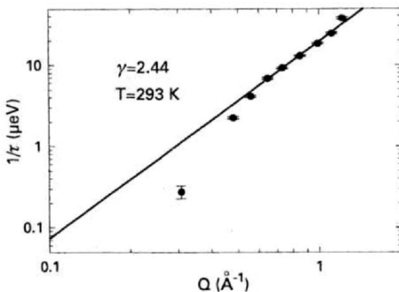
Figure 12. Log-log plot of 1/\tau vs Q , at T = 293 \text{ K} . Evidence of a power law dependence on the structural rate 1/\tau on Q .
