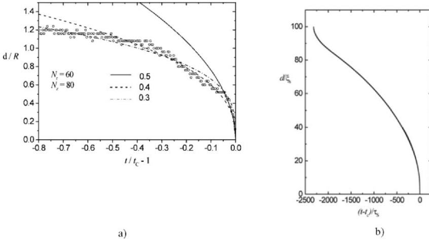
Figure 7. d = d(t) Dependence, (a) nematic point defects and (b) smectic edge dislocations.
