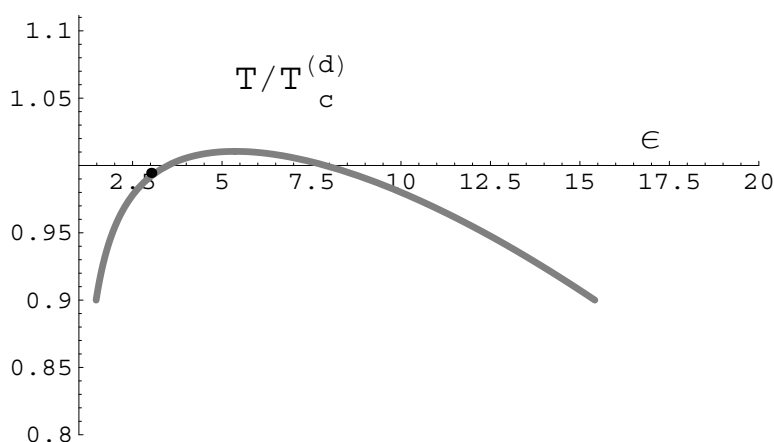
Figure 10. The dielectric permittivity according to Eq. (38) and the data.
