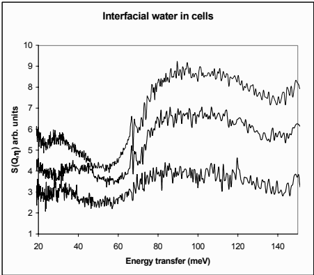
Figure 5. Interfacial water signals detected by IINS in cells and tissues after subtraction of the bulk water signal. Lower trace – Chlamydomonas cells (single-celled green algae). Center trace – beetroot (Beta vulgaris) tuber tissue. Upper trace – bovine cardiac muscle tissue.
