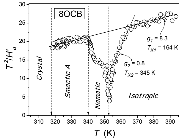
Figure 6. The linearized, derivative-based transformation of dielectric relaxation data from focused on the validity of the critical-like relation (3) in the description of dynamics in 8OCB (see relations (3) and (4)). All parameters given in the figure were determined from the linear regression analysis as discussed below relation (4) and derived in Ref. 15.
