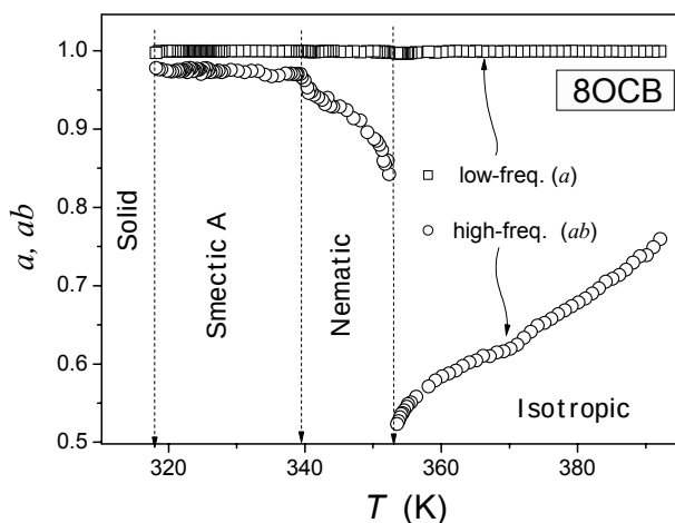
Figure 8. The evolution of Havriliak–Negami 1,2 form parameters describing the low- and the high-frequency wings of dielectric loss curves in 8OCB.
