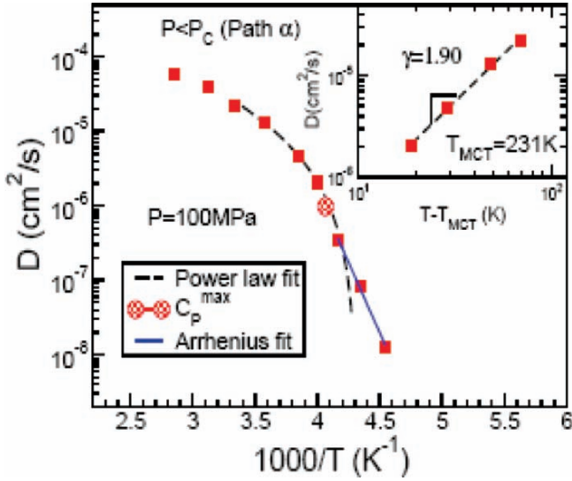
Figure 4. At high temperatures, D behaves like that of a non-Arrhenius liquid and can be fit by D \sim (T - T_{\text{MCT}})^{\gamma} (also shown in the inset) where T_{\text{MCT}} = 231 K and \gamma = 1.90 , while at low temperatures the dynamic behavior appears to change to that of a liquid where D is Arrhenius.
