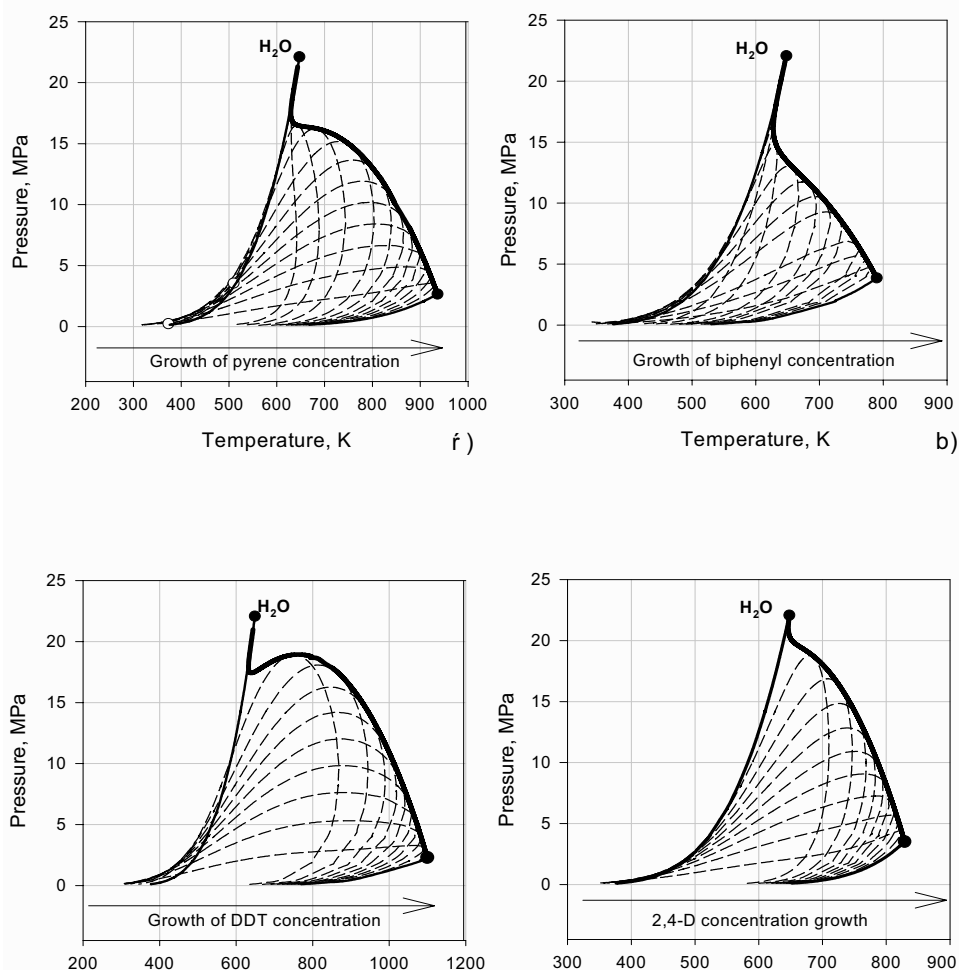
Figure 6. Phase envelopes for mixtures: a) pyrene-supercritical water; b) biphenyl-supercritical water; c) DDT-supercritical water; and d) 2,4-D-supercritical water.
