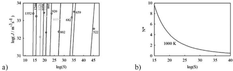
Figure 9. a) Nucleation rates for platinum obtained from the simulation. b) Critical cluster size obtained from the correlation shown in a).
