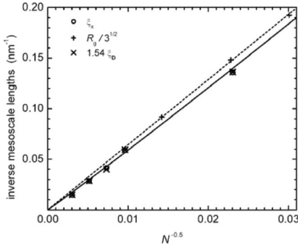
Figure 5. Inverse mesoscale lengths as a function of N^{-1/2} . 16 Circles are inverse correlation lengths \xi_x at the crossover temperature; \times are theoretically calculated inverse screening length \xi_D multiplied by 1.54; + are inverse normalized radii of gyration R_g/\sqrt{3} from Ref. 21. The solid curve represents a theory that includes logarithmic corrections.
