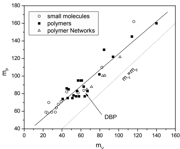
Figure 3. Isobaric fragility m_p (at atmospheric pressure) versus isochoric fragility m_v for 33 materials (in order of increasing m_v ). 20
