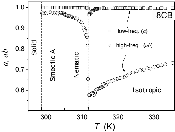
Figure 7. The evolution of Havriliak–Negami 1,2 form parameters describing the low- and the high- frequency wings of dielectric loss curves in 8CB.
