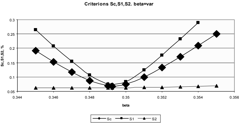
Figure 4. The influence of \beta = var on the criteria, S_1 , S_2 and S_c , of Models 1, 2 for the refractive indexes of R236ea.
