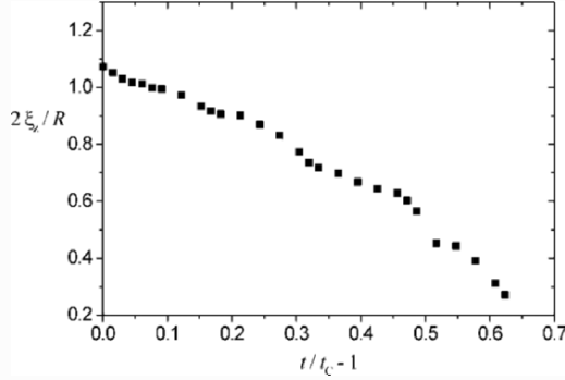
Figure 8. The time dependence of the chargeless ring size \xi_z in the post-collision regime. In the early regime the ring gradually shrinks and finally disappears.
