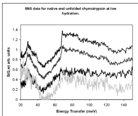
Figure 4. IINS spectra recorded for chymotrypsin, a small protein under different hydration levels and in the native and unfolded (denatured) states. From bottom to top: Unfolded chymotrypsin at 70 g water/100 g protein (gray trace). Unfolded chymotrypsin at 40 g water/100 g protein. Native chymotrypsin at 40 g water/100 g protein. Native chymotrypsin at 70 g water/100 g protein.
