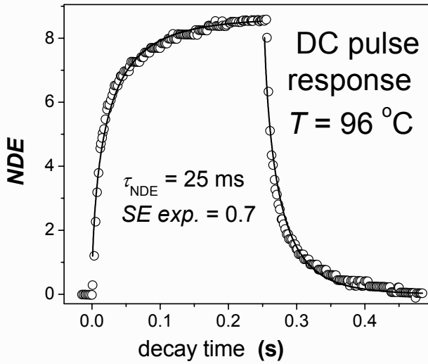
Figure 7. The NDE response induced by the DC pulse of a strong electric field in the vicinity of the SmA–SmC* transition. Solid curved are portrayed via the stretched exponential functions. NDE(t) = NDE_{\infty} (1 - \exp[-(t/\tau_{NL})^x]) or NDE(t) = NDE_{\infty} \exp[-(t/\tau_{NL})^x] , t denotes the elapse time and \tau_{NL} is the nonlinear dielectric relaxation time; NDE_{\infty} is for the saturated NDE value. Significant parameters are given in the figure.
