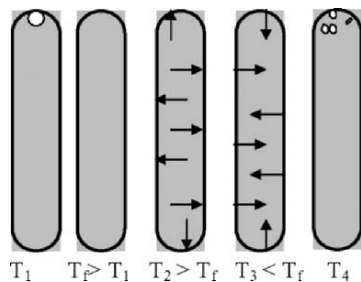
Figure 6. Straight-glass Berthelot method. For detailed explanation, see the text.
