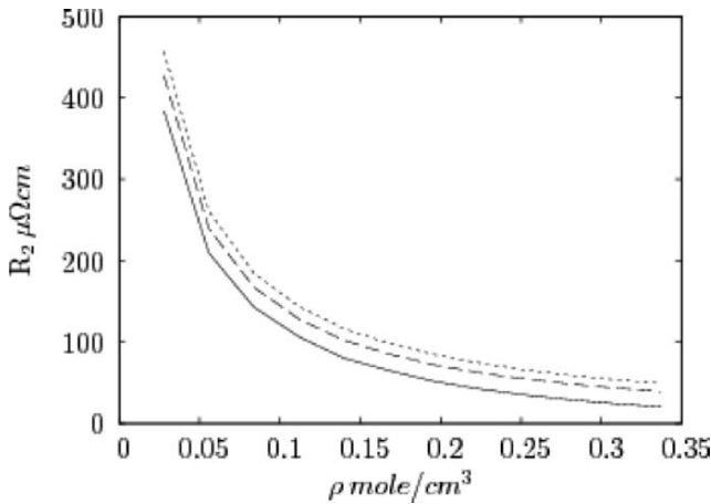
Figure 5. The resistivity of metallic hydrogen calculated using only the contribution of the second order in electron–proton interaction. --- T = 3000 \text{ K} , - - T = 6000 \text{ K} , ... T = 12000 \text{ K} .
