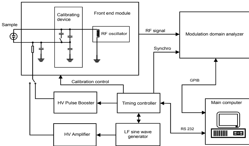
Figure 3. The scheme for the dual-field, single-generator and modulation domain nonlinear dielectric spectrometer.
