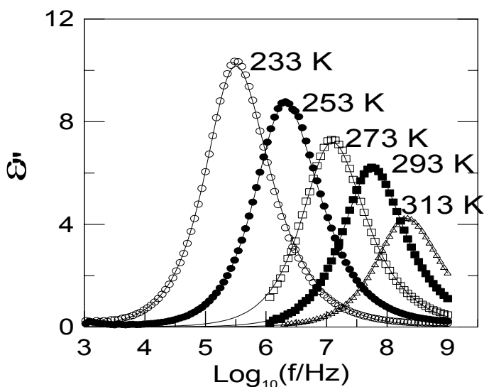
Figure 6. The frequency dependence of the dielectric loss \epsilon'' for NPA at different temperatures in the OD fcc phase (left panel) and relaxation time as a function of the reciprocal temperature (from López et al. 69 ).
