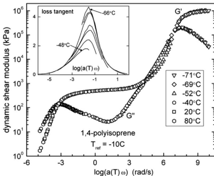
Figure 3. Master curve of the mechanical storage and loss moduli for 1,4-polyisoprene ( M_w=500 kg/mol). The inset shows the loss tangent in the transition zone, where thermorheological complexity is evident.
