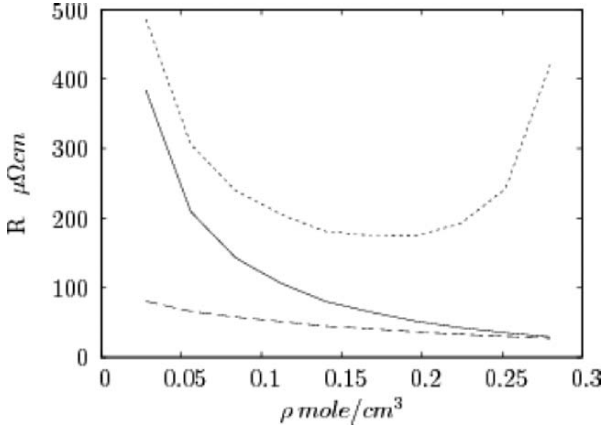
Figure 6. The resistivity of metallic hydrogen using the contributions of a higher order in electron–proton interaction at the temperature T=3000 K. --- R_2 , - - R_3 , ... R_2/(1-R_2/R_3) .
