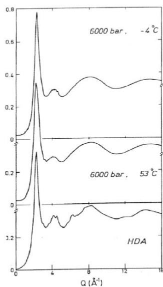
Figure 4. Structure factors S_M(Q) of liquid \text{D}_2\text{O} , under 6000 bar, as compared with that of high-density amorphous ice (HDA) at 77 K. 29
