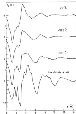
Figure 2. Pair correlation functions d_L(r) of supercooled \text{D}_2\text{O} , at normal pressure, as compared with that of low-density amorphous ice at 77 K. 29
