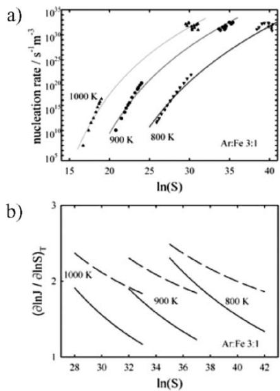
Figure 8. a) Nucleation rates for iron obtained from the simulation together with experimental data. 75 b) Critical cluster size obtained from the correlation shown in a); dashed lines: c=1 , solid lines: c=0 .
