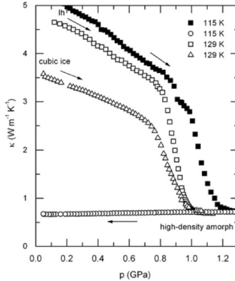
Figure 3. Thermal conductivity of hexagonal ice at 115 and 129 K and of cubic ice at 129 K is plotted against the pressure showing their respective amorphization ranges, and the thermal conductivity of the pressure-amorphized solid on lowering the pressure to ambient. The jog from the smooth sigmoid shape in the plot for 115 K near 0.9 GPa is caused by the inadvertent waiting at this pressure for an unknown period. The plots show that the onset pressure for amorphization decreases with increase in the temperature and is about 0.1 GPa lower for cubic ice at 129 K than for hexagonal ice. Data taken from Ref. 38.
