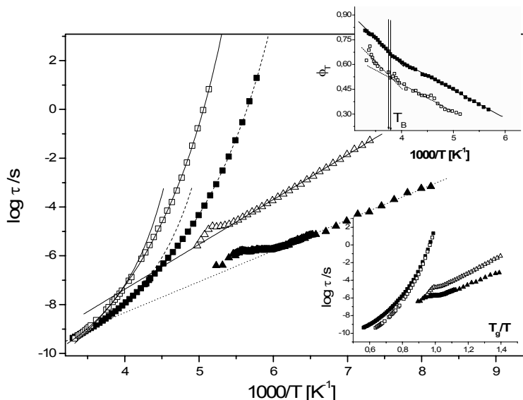
Figure 3. Arrhenius plot of the \alpha - and \beta -relaxation times for DIOM (solid points) and DIOP (empty points) (solid and dashed lines and curves represent fit by the VFT and activation law). Lower inset present the same data rescaled to glass temperature T_g . Upper inset show Stickel plot of the data.
