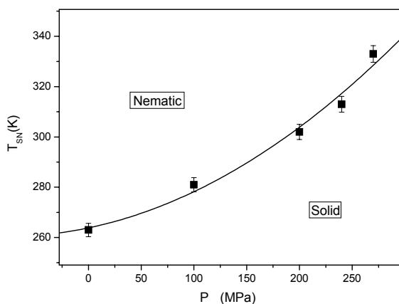
Figure 7. Pressured dependence of the solidification from the nematic phase of the 5CB–Aerosil mixture. Solid curve is a guide for the eyes.
