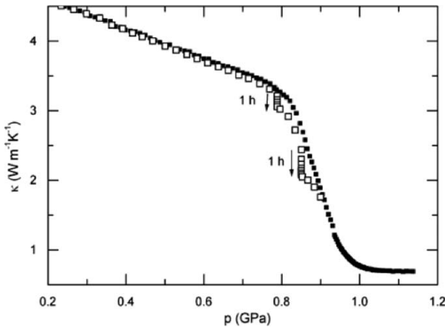
Figure 4. Thermal conductivity of hexagonal ice at \sim 130 K is plotted against the pressure. The vertical arrows during the course of crystallization are for fixed pressure conditions of 0.8 and 0.85 GPa at which the sample was kept for 1 h after the pressure-amorphization had begun. Data taken from Ref. 22.
