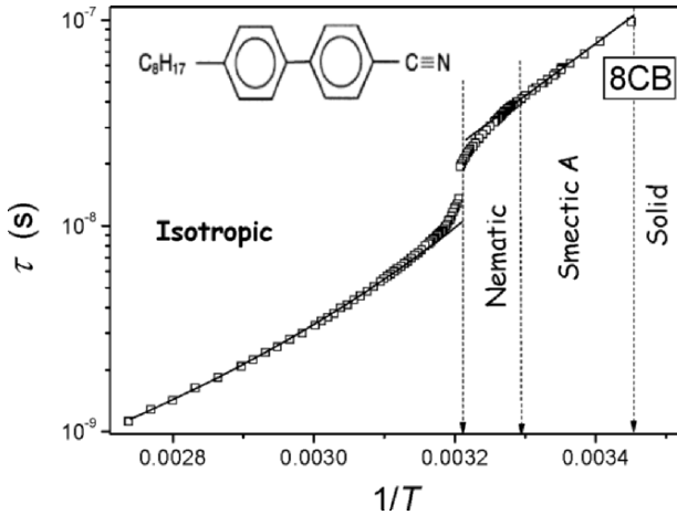
Figure 1. The Arrhenius plot of the evolution of dielectric relaxation times in isotropic and liquid crystalline 8CB. The solid curve is plotted via the VFT relation (1) with parameters taken from the linearized, derivative-based analysis given in Fig. 2: D_T = 2.6 and T_0 = 218 K. The fit yielded \tau_0^{VFT} = 24.7 ps for the prefactor. The glass temperature from the condition \tau(T_g) = 100 s yields T_g = 238 K.
