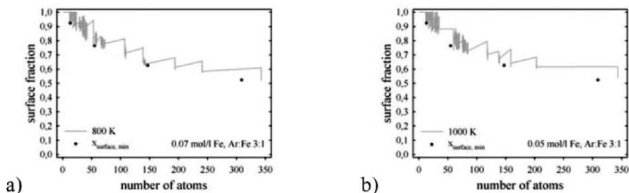
Figure 13. Surface fraction of the largest cluster in the system vs. its size for a) 800 K and 0.07 mol/l Fe and b) 1000 K and 0.05 mol/l Fe.
