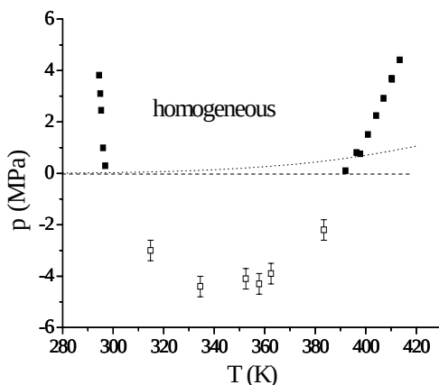
Figure 2. Liquid-liquid locus of polystyrene/methyl acetate mixture (2 w%, M_w=2,000,000 ). Black marks: direct data by optical measurement, 12 hollow marks: extrapolated data from isotherm conductivity measurements, dotted line: vapor pressure curve of the methyl acetate.
