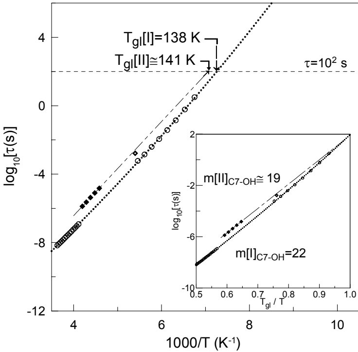
Figure 4. \alpha -Relaxation time for phases I (empty circles) and II (full diamonds) of cycloheptanol in an Arrhenius plot. The lines correspond to the VFT-fitting of the \alpha -relaxation data in phase I and to the Arrhenius fitting for phase II. The inset shows the typical Angell's plot for the \alpha -relaxation in phases I and II with the fragility index (from Puertas et al. 48 ).
