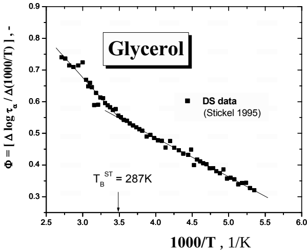
Figure 5. Stickel's plot for the primary \alpha relaxation time, \tau_\alpha for GL demonstrating the change in the dynamical regime at the characteristic DS (Stickel) temperature, T_B^{\text{ST}} correlating with the characteristic PALS temperature T_{b2}^L .
