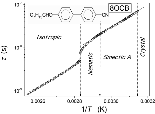
Figure 4. The Arrhenius plot of the evolution of dielectric relaxation times in isotropic and liquid crystalline 8OCB. The solid curves indicate the Arrhenius temperature behavior.
