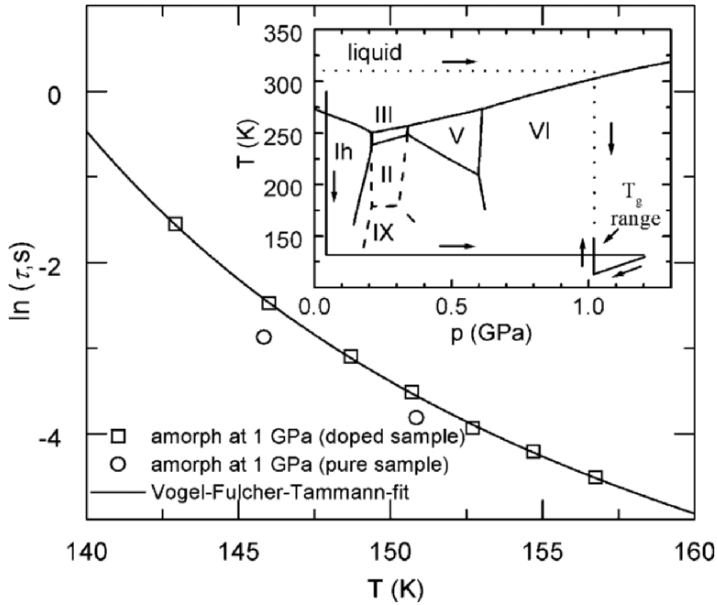
Figure 8. The relaxation time of pure and KOH-doped amorph at 1 GPa plotted against the temperature. The line is the best fit of the Vogel–Fulcher–Tammann equation, \ln \tau = -9.81 + [204.0/(T - 118.2 \text{ K})] . Data taken from Ref. 79. Inset is the phase diagram of the ices. The temperature–pressure region in which amorphization studies of hexagonal ice have been performed are indicated. The path that leads to an ultraviscous liquid state is shown by arrows. The path from the liquid water to ultraviscous state shown by the dashed line requires supercooling at 1 GPa. This path has not been experimentally achieved.
