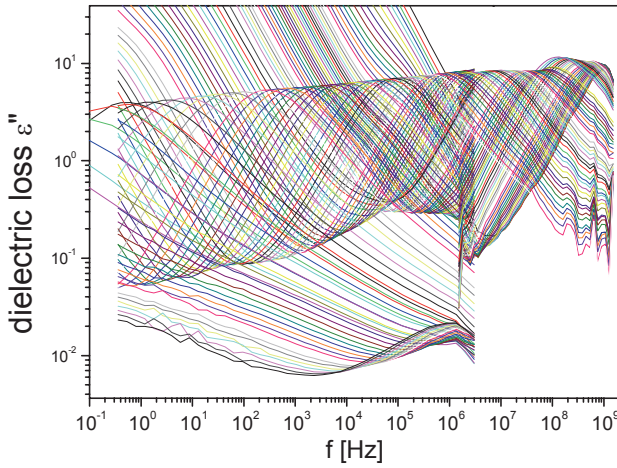
Figure 10. The frequency dependence of the dielectric loss \varepsilon'' for NPA_{0.70}NPG_{0.30} mixed crystal at different temperatures from 363 K (liquid state) down to 130 K. Measurements were performed every 2 K on slow cooling.
