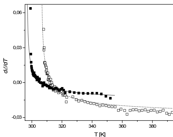
Figure 3. Derivative analysis of \varepsilon'(T) data from Fig 2. The solid and the dashed curves are portrayed by eq. (2) with the same exponent \alpha = 1/2 .
