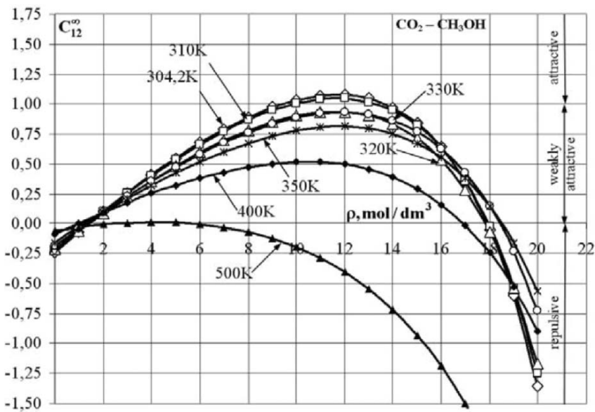
Figure 3. Direct correlation function integral for mixture CO 2 -CH 3 OH at infinite dilution.
