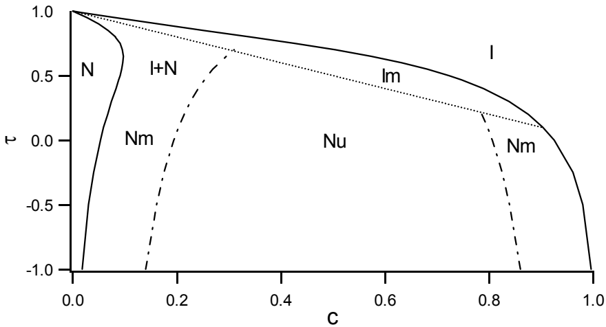
Figure 1. Phase diagram for nematic-non-nematic binary mixture. The solid curve refers to the binodal, the dotted line shows the hidden nematic-isotropic phase transition, and the dashed-dotted line is the spinodal. \Gamma = \lambda = \chi = 1 .
