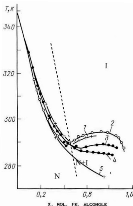
Figure 1. Phase diagrams of BMOAB-alcohol solutions. 3 I indicates the isotropic region, N the nematic region, N+I the two-phase region. Clearing temperatures (the last droplet of the nematic phase disappears): 1 propanol, 2 isopentanol, 3 n -butanol, 4 n -pentanol, 5 n -decanol. Dashed line: the last droplet of the isotropic phase disappears (shown for BMOAB- n -decanol solutions). In solutions of BMOAB in propanol, isopentanol, and n -butanol two isotropic phases coexist. Note, the clearing-temperature curve for BMOAB- n -pentanol solution is very flat, implying a close critical phase separation.
