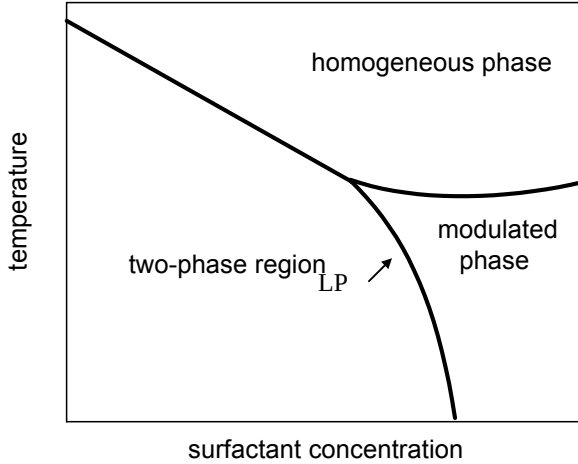
Figure 3. Schematic phase diagram of surfactant solution forming a modulated phase. The Lifshitz point (LP) separates the critical line of liquid–liquid phase separation (on the left) and the first order phase separation (lower curve on the right). The transition between the homogeneous disordered phase and the modulated phase is second order.
