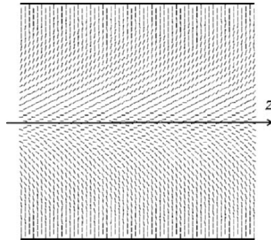
Figure 3. The escaped radial nematic structure.
