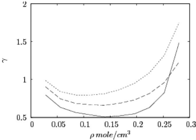
Figure 8. The temperature and density dependence of the nearly free electrons model applicability criterion. --- T = 3000 K, - - T = 6000 K, and ... T = 12000 K.
