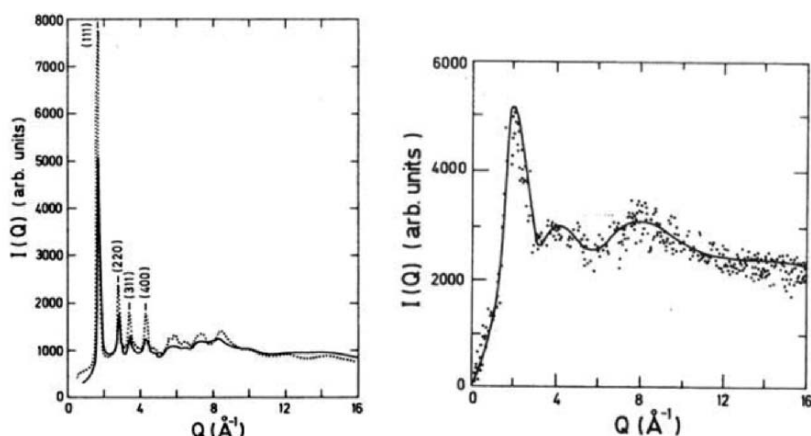
Figure 9. (a) (left side) Spectrum of cubic ice ( -198^{\circ}\text{C} ) (dotted line) compared with that of confined \text{D}_2\text{O} at -100^{\circ}\text{C} from fully hydrated Vycor (full line).
