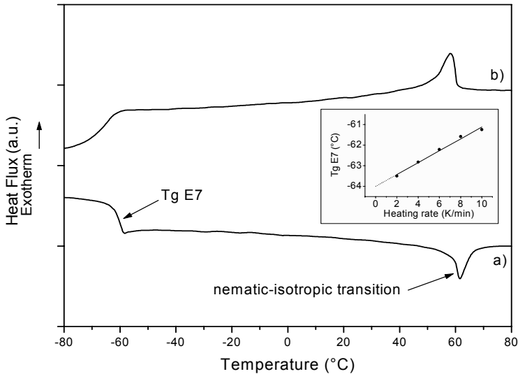
Figure 2. DSC thermogram of the eutectic mixture of the liquid crystals E7 for the second heating (a) and second cooling (b) ramp. The applied rate was 10 K/min. The inset exhibits the dependence of the glass transition as a function of the heating rate.
