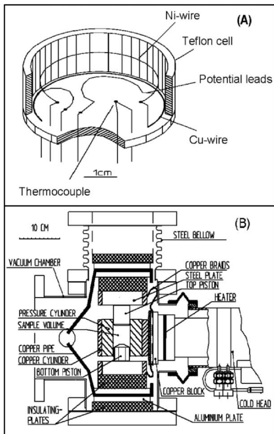
Figure 1. (A) The high pressure cell assembly for measuring the thermal conductivity and heat capacity. (B) The arrangement of the high pressure vessel showing the application of the uniaxial stress and arrangement that allows the use of helium cryostat in a massive assembly.
