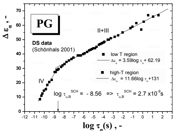
Figure 6. Schönhals' plot for the primary \alpha relaxation time, \tau_\alpha , for PG showing the change in the \alpha relaxation strength at the characteristic DS (Schönhals) temperature, T_B^{\text{SCH}} correlating with the characteristic PALS temperature T_{b2}^L .
