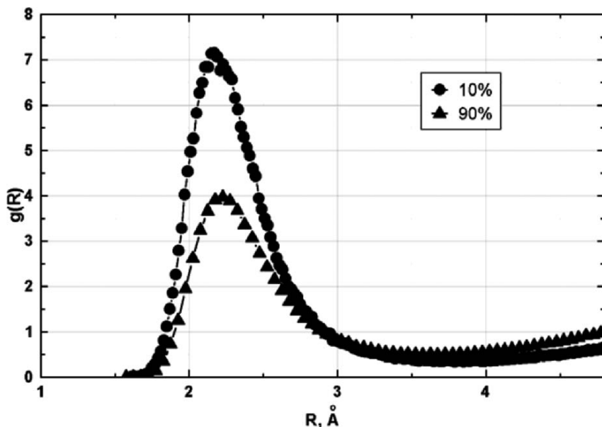
Figure 4. LiCl radial distribution function at two concentrations of LiCl: 10% (circles) and 90% (triangles).
