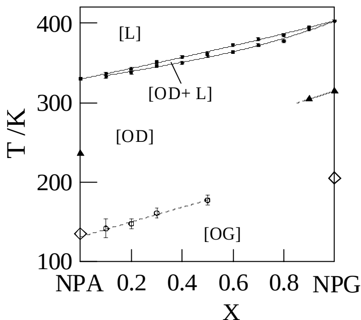
Figure 8. Equilibrium phase diagram for the NPA+NPG two-component system together with the glass-transition temperatures as determined from specific-heat measurements, except for pure compounds for which they were obtained from dielectric measurements by superimposing \tau(T_g)=100 s. Full symbols were obtained by scanning calorimetry. 78,79
