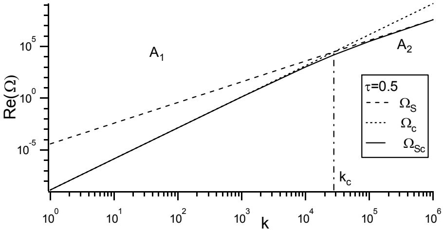
Figure 4. The inner region (leading-order) damping rate (continuous curve) for nematic–non-nematic mixture, defining two distinct regimes. The non-conserved order parameter dispersion relation (dashed curve) and conserved parameter dispersion relation (dotted curve). In the region A_1 relaxation of the concentration is the important process, while in the region A_2 relaxation of the orientational order parameter dominates.
