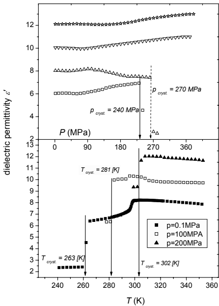
Figure 6. Temperature and pressure dependences of dielectric permittivity measured at 10 kHz for mixture of 5CB with aerosil. Arrows indicate temperatures of crystallization.
