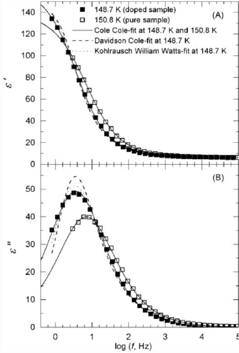
Figure 7. The dielectric permittivity and loss spectra for pure amorph and KOH-doped amorph at 1 GPa at 150.8 and 148.7 K, and its analysis in terms of the Cole–Cole symmetrical distribution of relaxation times. For the KOH-doped sample, the measured values were converted to \epsilon' and \epsilon'' by using the cell constant, C_g = C_\infty (KOH-doped water)/ \epsilon_\infty (pure water) at 130 K. The best fit parameters of the Cole–Cole function are: \alpha = 0.29 and \epsilon_0 = 164 , \epsilon_\infty = 6.4 , and \tau_{CC} = 0.044 s. The corresponding data for pure water at 150.8 K are: \alpha = 0.30 and \epsilon_0 = 132 , \epsilon_\infty = 6.4 , and \tau_{CC} = 0.022 s. Data taken from Ref. 79.
