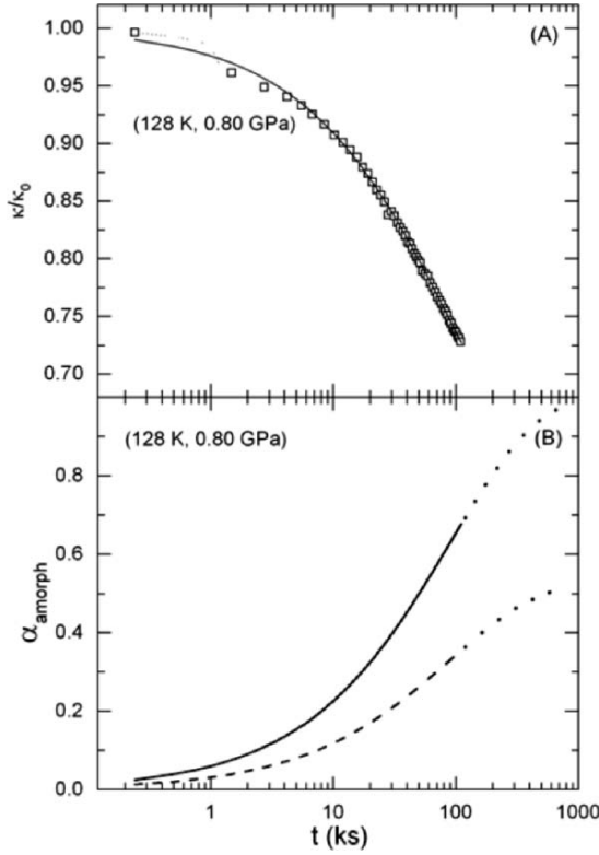
Figure 6. (A) The normalized value of thermal conductivity measured during the amorphization of hexagonal ice at 0.8 GPa and 128 K is plotted against logarithmic time. \kappa_0 is the value at the beginning of the measurements. (B) The degree of amorphization of the ice at 0.8 GPa and 128 K, calculated from Eq. (3) is plotted against the time on a logarithmic scale: For the solid line \kappa_\infty is assumed to be 1.8 \text{ W m}^{-1} \text{ K}^{-1} , and for dashed line \kappa_\infty is assumed to be 0.7 \text{ W m}^{-1} \text{ K}^{-1} . The dotted lines correspond to extrapolations by using Eq. (2). The plot was calculated by assuming that the sample is a mixture of crystalline and amorphous ice and the amorphous \kappa(\infty) of \sim 0.7 \text{ W m}^{-1} \text{ K}^{-1} does not reach a long time limiting value because the sample remains a mixture of ice and amorph at that time. Data taken from Ref. 38.
