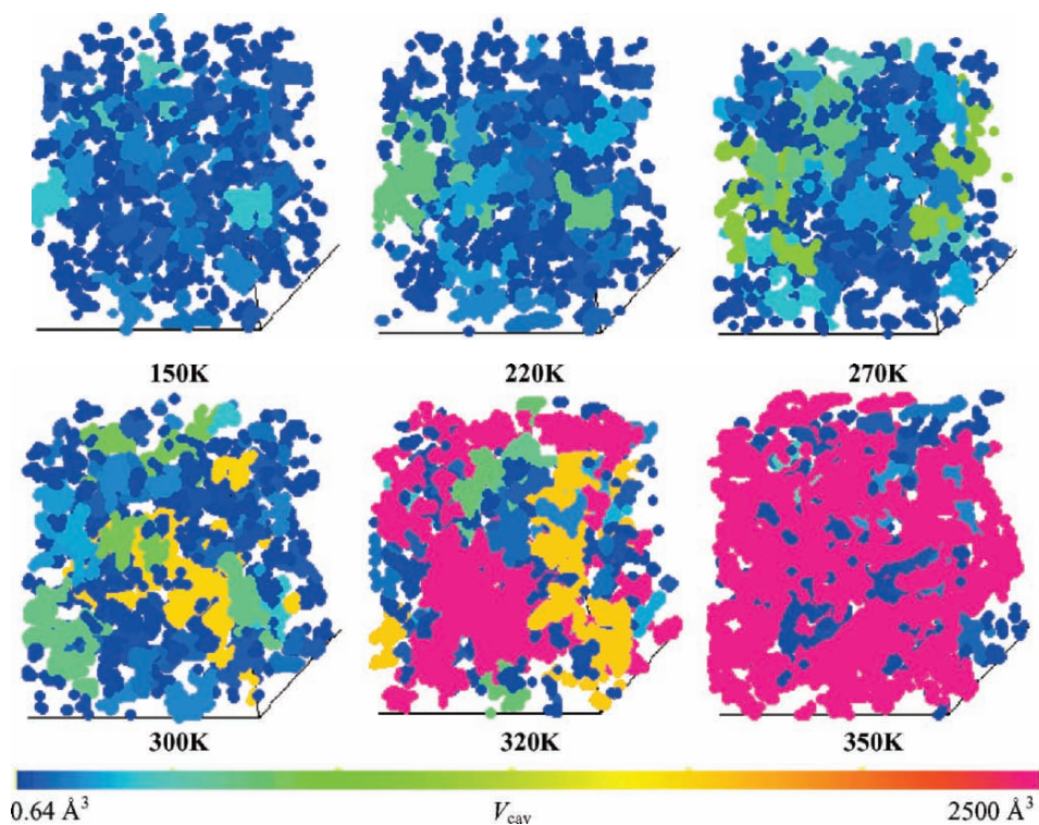
Figure 12. Temperature evolution of the cavity microstructure in 3D space for GL. Yellow color indicates the presence of the percolated cavity volume over the whole simulation box.
