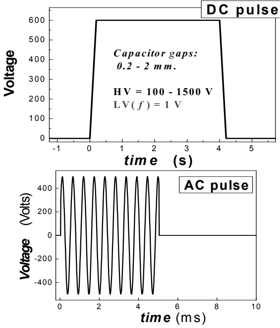
Figure 5. Forms of high voltage pulses applied in NDE studies in this paper.
