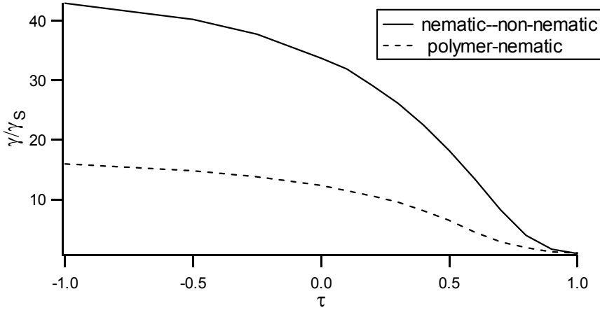
Figure 3. Interfacial tension between the isotropic and nematic phases plotted against the reduced temperature. The solid curve refers to the nematic-non-nematic mixture and the dashed line corresponds to the polymer-nematic mixture.
