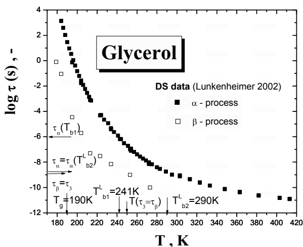
Figure 4. Relationship between the o-Ps lifetime, \tau_3 , and the secondary \beta_{JG} relaxation time, for \tau_\beta for GL.
