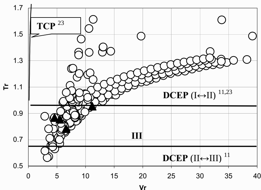
Figure 3. Distribution of hydrocarbon–water mixtures in reduced variables.
