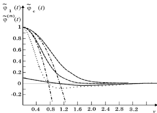
Figure 1. Time dependences of the autocorrelation functions. The solid curve corresponds to the normalized autocorrelation function of a Lagrange particle, 11 the dash-dotted curves to the dependences \varphi_l(t) that decay by a polynomial law, the dashed curves to exponential dependences, and the dotted curve to a dependence obtained on the basis of the molecular dynamics data. 14
