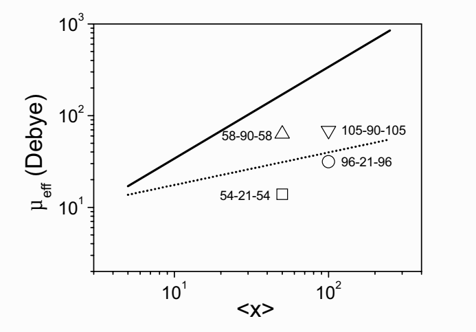
Figure 4. Calculated effective dipole moment of PBLG plotted as a function of the degree of polymerization in the triblock copolymers PBLG- b -PEO- b -PBLG. The solid line gives the expected effective dipole moment for a perfect \alpha -helical structure. The symbols correspond to the different copolymers; up triangle: PBLG 58 - b -PEG 90 - b -PBLG 58 , down triangle: PBLG 105 - b -PEG 90 - b -PBLG 105 , square: PBLG 54 - b -PEG 21 - b -PBLG 54 , circle: PBLG 96 - b -PEG 21 - b -PBLG 96 .
