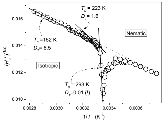
Figure 5. The derivative transformation plot of the data presented in Fig. 4. The linear regression analysis applied for the following domains yields VFT parameters given in the figure.
