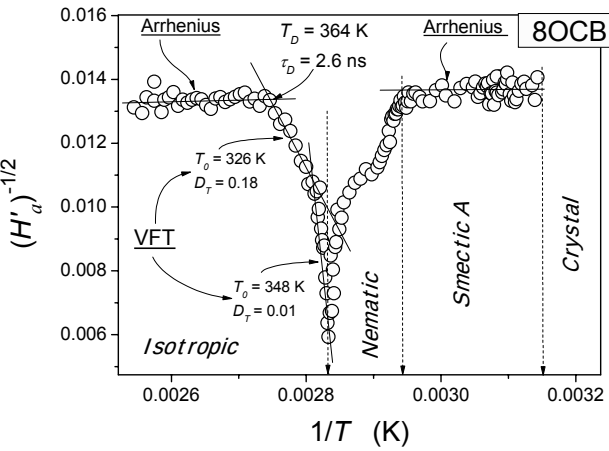
Figure 5. The linearized, derivative-based transformation of dielectric relaxation data from focused on the validity of the VFT relation in the description of dynamics in 8OCB (see relations (1) and (2)). All parameters given in the figure were determined from the linear regression analysis as discussed below relation (2) and derived in Ref. 15. The horizontal line points out Arrhenius domains.
