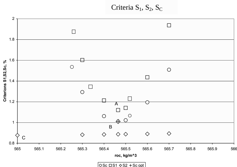
Figure 3. The influence of \rho_c = var on the criteria, S_1 , S_2 , and S_c , of Models 1, 2 for the densities of R236ea. S_1^{min} , S_2^{min} , and S_c^{min} are shown as A, B, and C.
