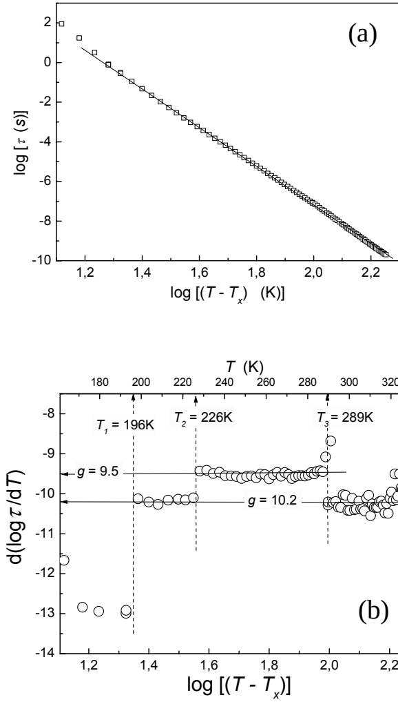
Figure 15. (a) The log-log plot showing the possible validity of the MCT “critical” like behavior \tau \propto (T - T_X)^{-\gamma} , with \gamma = 9.8 and T_X = 148 K. (b) The derivative of the log-log MCT plot given in (a). It confirms the validity of the MCT “critical-like relation” but reveals existence of three different regimes, with different values of the power exponent \gamma . The crossover temperatures agree well with temperatures indicated in Figs. 12 and 13.
