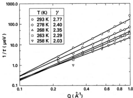
Figure 10. Evidence of a power law dependence of the structural relaxation rate on Q (Eq. 9), measured with 10 \mu\text{eV} resolution, in the 100% hydrated sample. This graph shows a log-log plot of 1/\tau vs Q . Within a Q range of 0.1–1 \text{\AA}^{-1} the exponent \gamma , which is the slope of the solid lines joining the data points, seems to be a constant. The corresponding data from MD simulation 54 show that the exponent \gamma is Q -dependent, approaching 2 as Q goes below 0.1 \text{\AA}^{-1} .
