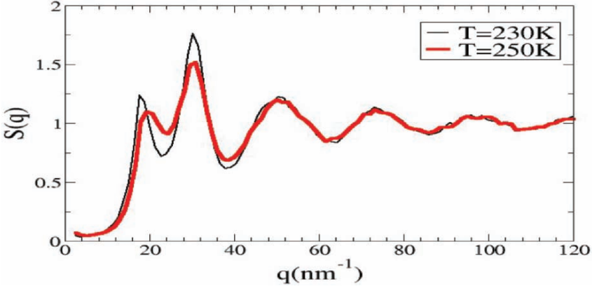
Figure 6. Structural changes on crossing the Widom line at P = 100 MPa. (a) Oxygen–oxygen structure factor S(q) above the Widom line (see Fig. 5). (b) Structure factor S(q) below the Widom line. Tetrahedrality of the water molecules increases dramatically upon crossing the Widom line indicated by a sharp increase in the first and second peaks of the structure factor.
