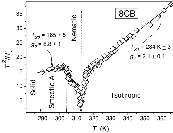
Figure 3. The linearized, derivative-based transformation of dielectric relaxation data from focused on the validity of the critical-like relation (3) in the description of dynamics in 8CB (see relations (3) and (4)). All parameters given in the figure were determined from the linear regression analysis as discussed below relation (4) and derived in Ref. 15. Note that \tau_{VFT}(T_{X1}) \approx 1.3 \times 10^{-7} , in fair agreement with the “magic” universal time-scale (see Refs. 20 and 21).
