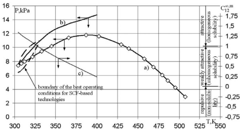
Figure 4. LPD of binary mixture SCF(CO 2 )–cosolvent (C 6 H 14 ): a) critical curve P^c(T) ; 14 b) maxima-of-pressure curve P^m(T) , corresponding to the best miscibility of components; c) decreasing of hexane solubility in carbon dioxide with temperature increasing.
