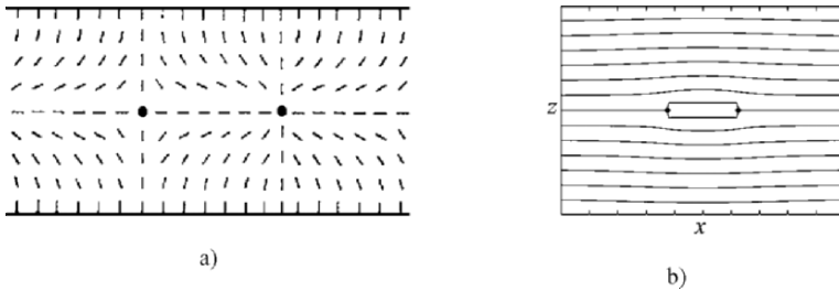
Figure 1. Schematic presentations of pairs of defects. (a) A nematic anti-hedgehog (left) and hedgehog (right) point defect within a cylindrical confinement and (b) a pair of SmA edge dislocations. The smectic layers are stacked along the z -direction of the Cartesian coordinate system (x, y, z) .
