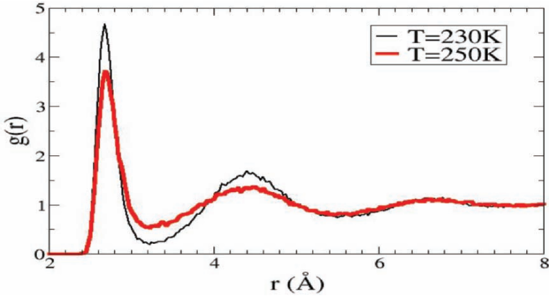
Figure 5. Oxygen–oxygen pair correlation function above and below the Widom line at P = 100 MPa. Above the Widom line, water is less ordered while upon crossing the Widom line, water becomes more ordered.
