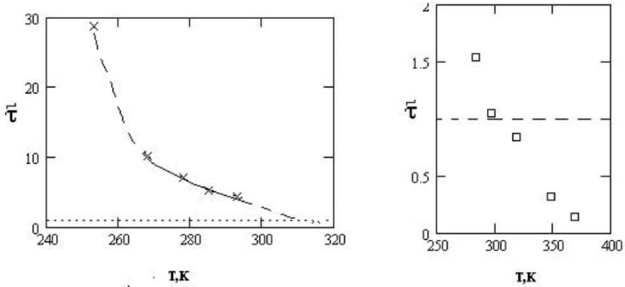
Figure 3. The temperature dependence of the ratio \tilde{\tau} = \tau_0 / \tau_1 (see the text for explanation).
