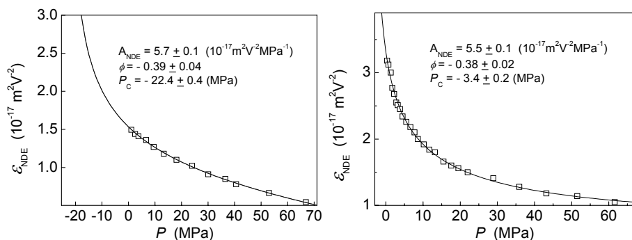
Figure 3. Anomaly of the nonlinear dielectric effect (NDE) measured on two isotherms. The form of the anomaly is \varepsilon_{\text{NDE}} = [A_{\text{NDE}}(P - P_c)^\phi]_{\text{critical}} + [C + BP]_{\text{background}} . The obtained critical pressures can be seen in the inserts. a (left): T_c = 26.7^\circ\text{C} , b (right): T_c = 19.5^\circ\text{C} .
