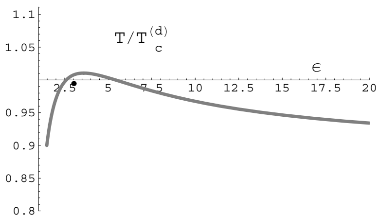
Figure 8. Theoretical curve according to Eq. (34) and experimental points for \epsilon(T) along the binodal.
