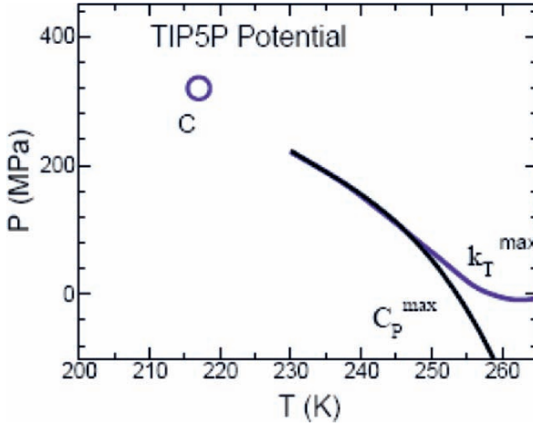
Figure 3. Relevant part of the phase diagram for the TIP5P potential, showing the liquid-liquid critical point C at P_c = 320 MPa and T_c = 217 K, the line of maximum of isobaric specific heat C_p^{\text{max}} and the line of maximum of isothermal compressibility k_T^{\text{max}} .
