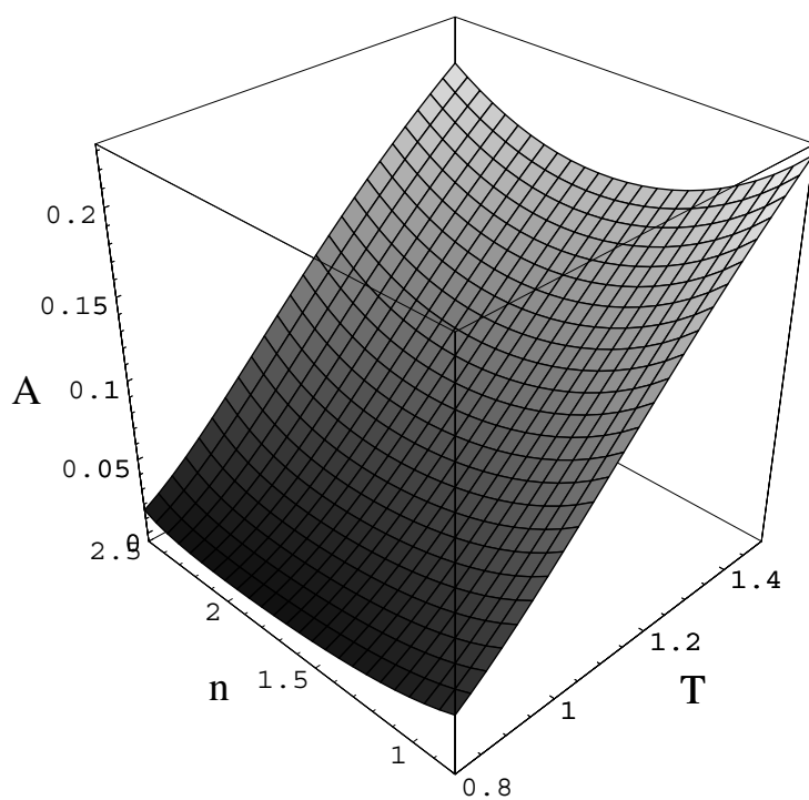
Figure 4. The degree of dissociation A as a function of (dimensionless) density and temperature at E_H = 3.87 T_c^{(d)} , \tilde{\lambda} = 0.6 , and \tilde{\sigma} = 0.88 .
