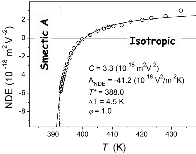
Figure 9. The stationary NDE response in the isotropic phase of DOBAMBC, on approaching the isotropic–smectic a transition. The response is associated with DC pulse excitation.
