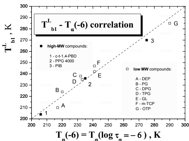
Figure 3. The empirical correlation between the first characteristic PALS temperature, T_{b1}^L , and the temperature, T_\alpha(-6) , at which the primary \alpha relaxation time, \tau_\alpha , reaches just 10^{-6} s for a series of small molecular and polymer glass-formers.
