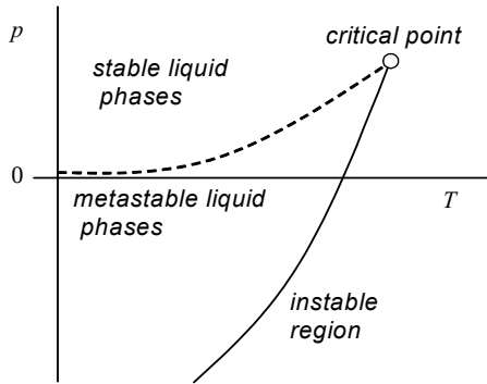
Figure 2. Schematic phase diagram and liquid–vapor spinodal for a van der Waals fluid. Dashed line represents the vapor pressure curve, solid line represents the L–V spinodal.
