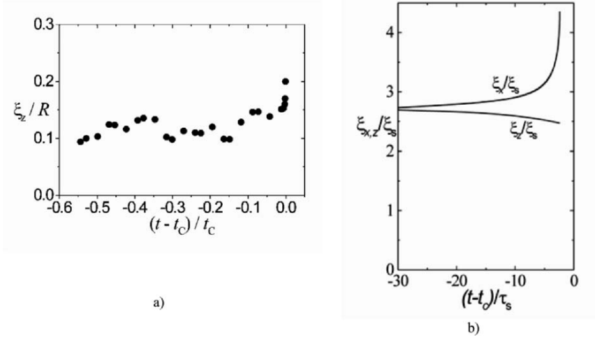
Figure 4. (a) The average ring radius as a function of time. At a given time the radii of hedgehog and anti-hedgehog are comparable and (b) the characteristic radii \xi_x and \xi_z of the edge dislocation core structure along the x and z axis. Prior the collision the value of \xi_x strongly increases. \tau_s \approx \gamma|\alpha|^{-1} .
