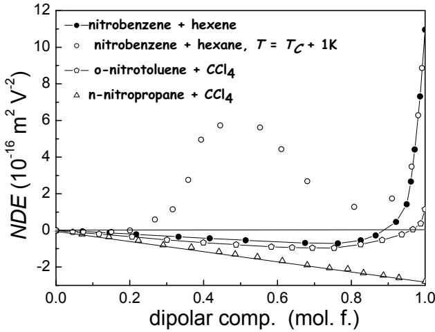
Figure 2. Isothermal behavior of NDE in selected solutions composed of a dipolar component and a nondipolar solvent (hexene, hexane, carbon tetrachloride). For the mixture nitrobenzene – hexane studies were carried out just above the critical consolute temperature ( T_C = 19.5^\circ\text{C} ). Curves in the figure are guides for eyes.
