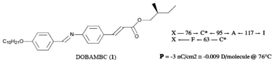
Figure 4. The ferroelectric liquid crystalline (FLC) molecule of p -( n -decyloxy) benzylidene- p -amino-(2-butyl)cinnamate (abb. DOBAMBC), its polymorphism, and polarity. The letter I is for the isotropic liquid, X is for the solid phase. The other letters are for Smectic mesophase. The polymorphism appearing on cooling and heating is given. 18
