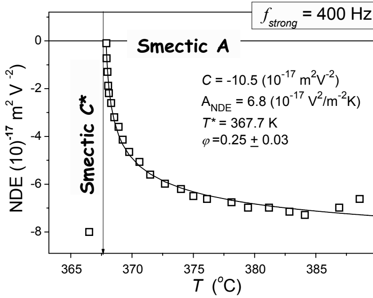
Figure 8. Results of the frequency selective NDE studies in SmA mesophase of DOBAMBC in the stationary nonlinear domain.
