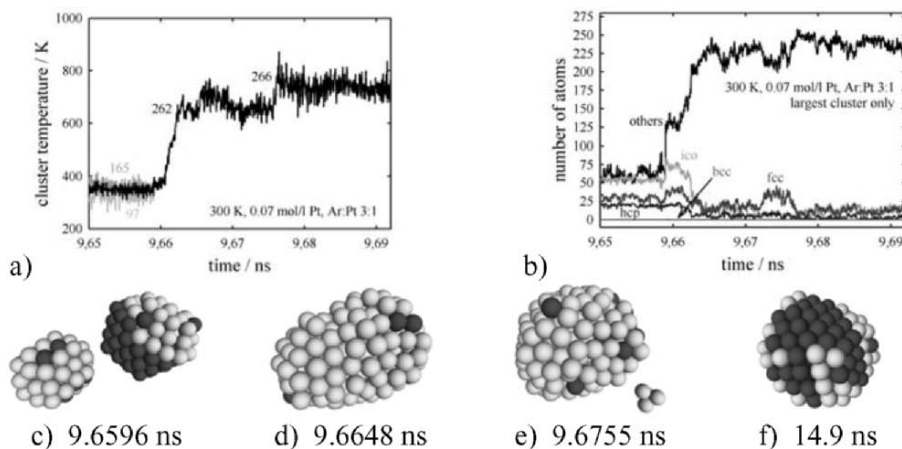
Figure 17. a) High temporal resolution of the heating up of the largest cluster after the collision of the two clusters of 165 and 97 atoms. The newly formed cluster of 262 atoms is hit by a tetramer about 150 ps later. b) Development of the structural composition for the same time range as in a). c)–f) Snapshots of the clusters taking part in the coalescence process c) before the collision, d) shortly after, e) snapshot prior to the collision with the tetramer, f) restructured cluster several ns later.
