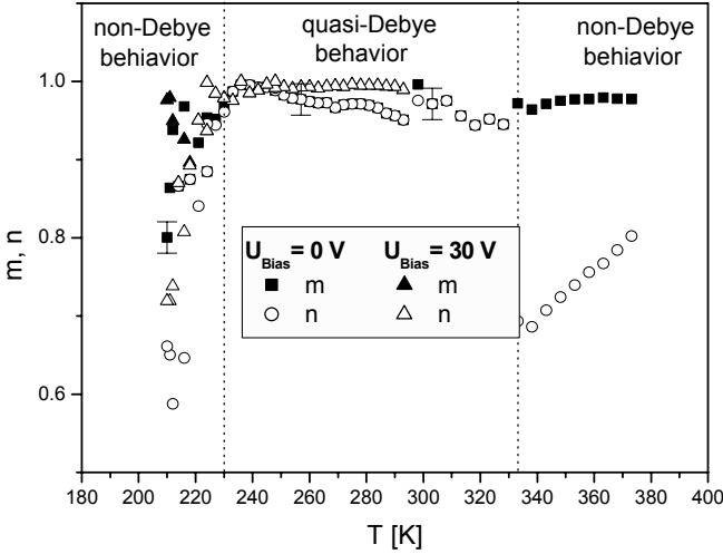
Figure 9. The shape parameters of dominated relaxation process obtained from fitting process of the HN relaxation function to the data in Fig. 1.
