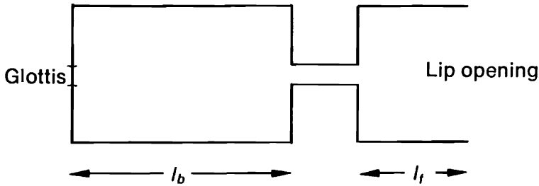
Figure 8.12. An idealized model of the supralaryngeal vocal tract for the production of fricative consonants. The position of the constriction can be shifted by changing the values of the length of the back and front cavities, l_b and l_f .
