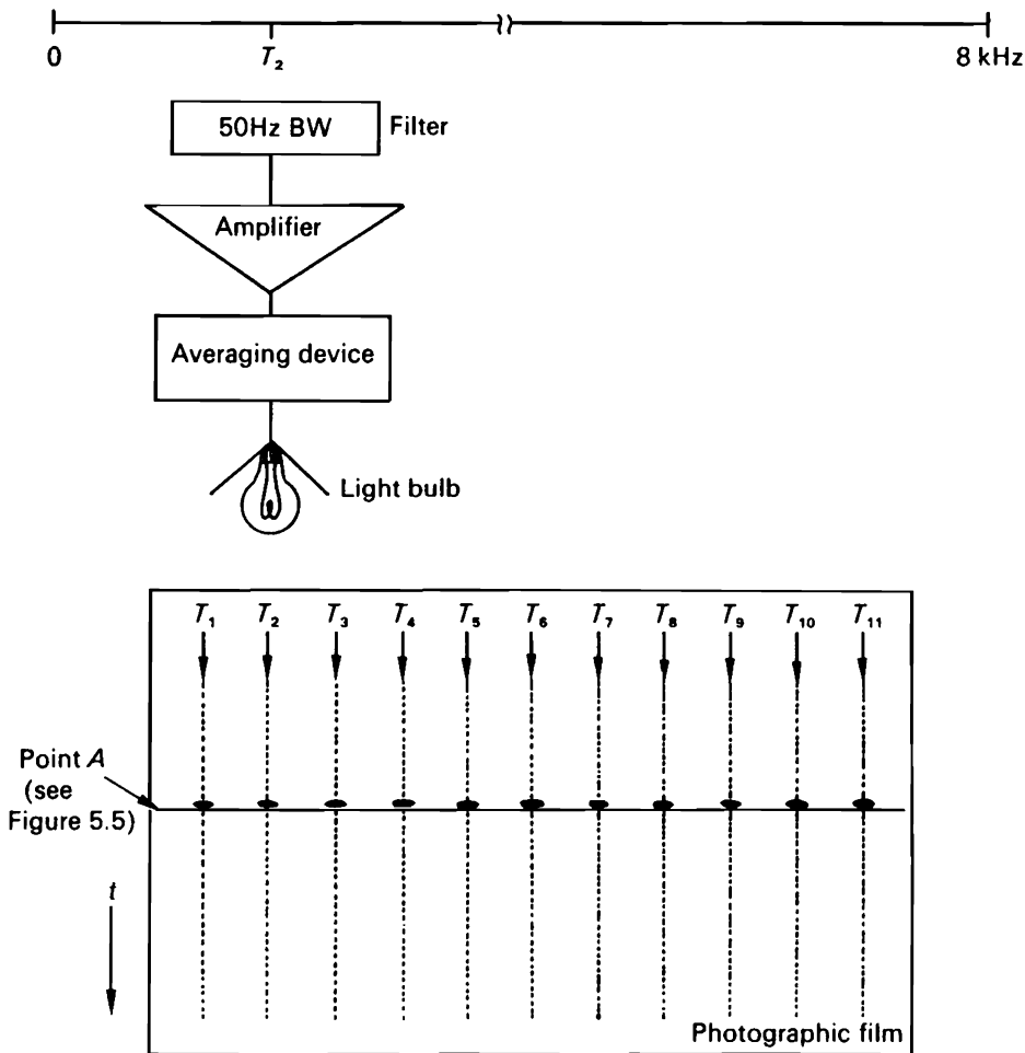
Figure 5.4. Sketch of a hypothetical "photo-output" narrow-band sound spectrograph machine.
