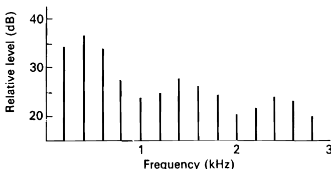
Figure 4.6. Spectrum of the sound [ə] produced with a different fundamental frequency of phonation. The speech signal still has the phonetic quality of the vowel [ə] although it has a different fundamental frequency than the [ə] whose spectrum is plotted in Figure 4.4.
