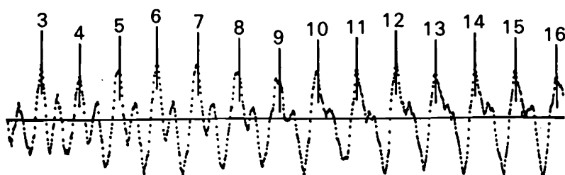
Figure 5.18. A waveform with successive pitch periods marked by the computer.
