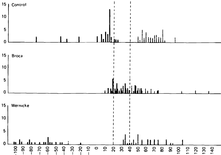
Figure 9.6. The distribution of VOT productions for the alveolar stop consonants for a normal control, a Broca's aphasic, and a Wernicke's aphasic. From S.E. Blumstein, Neurolinguistics: Language-brain relationships . In S.B. Filskov and T.J. Boll (eds.), Handbook of Clinical Neuropsychology . Reprinted by permission of John Wiley & Sons, Inc. Copyright © 1981.
