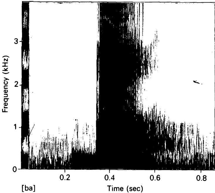
Figure 5.2. Wide-band spectrogram of the sound [ba].
