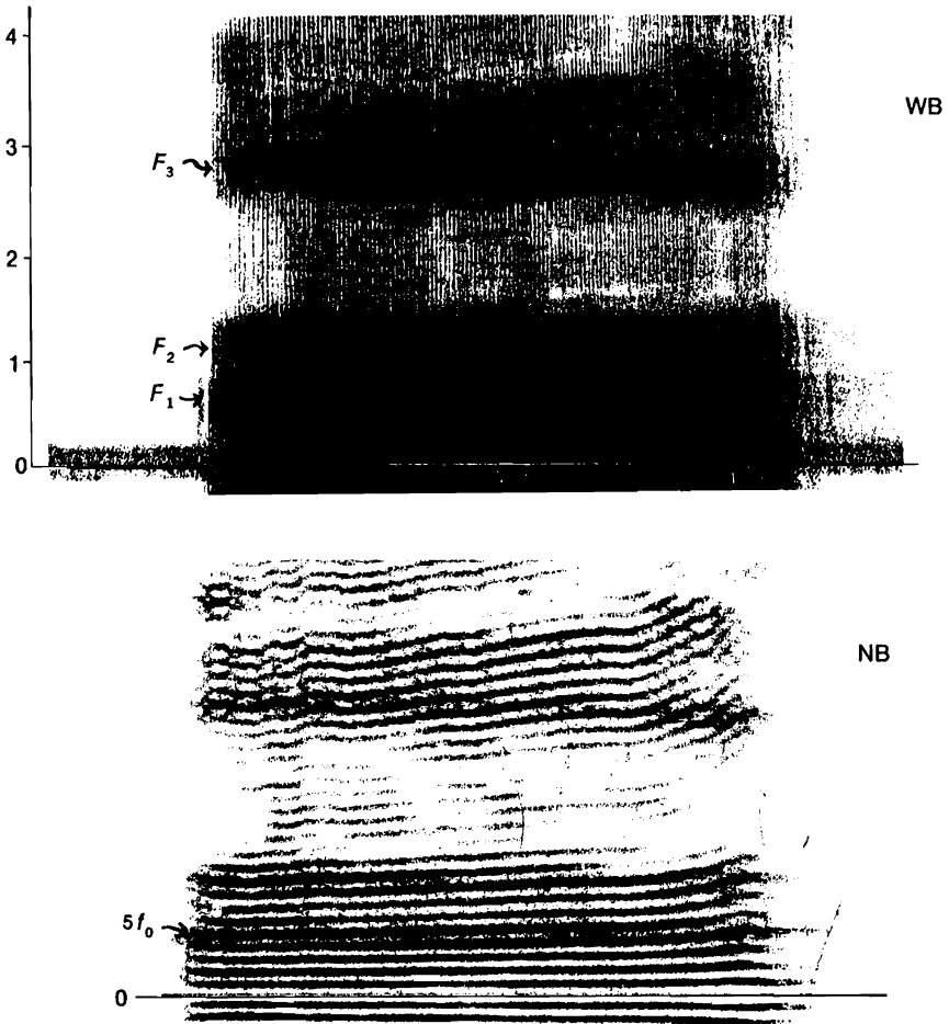
Figure 5.13. Using the mirror image technique for “zero” frequency calibration. The formant frequencies are noted on the upper wide-band spectrogram. The fifth harmonic of the fundamental frequency is marked on the lower narrow-band spectrogram.
