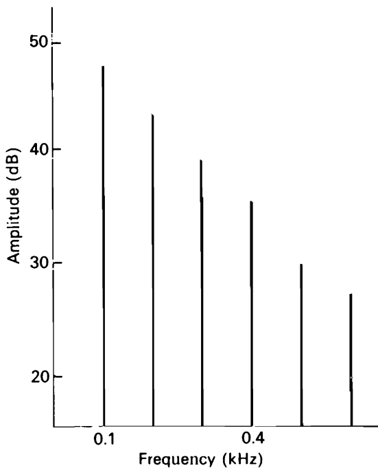
Figure 4.2. Spectrum of typical glottal air flow.
