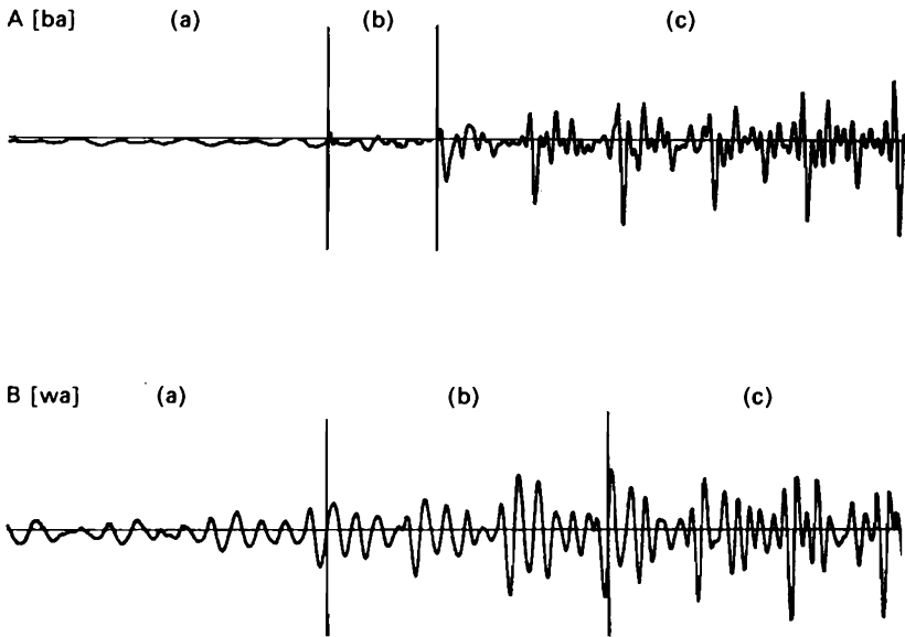
Figure 5.16. Waveforms for the sounds [ba] and [wa]. Letters indicate different acoustic segments demarcated by cursors: (a) prevoicing, (b) consonantal release, and (c) steady-steady portion of the vowel. (After Mack and Blumstein, 1983.)
