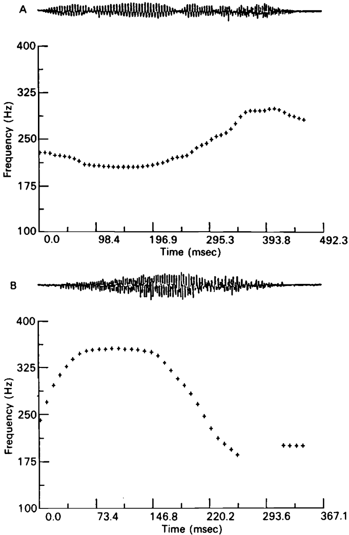
Figure 5.17. Waveforms and fundamental frequency of phonation for the vowel [i] in two words of Chinese spoken in isolation.
