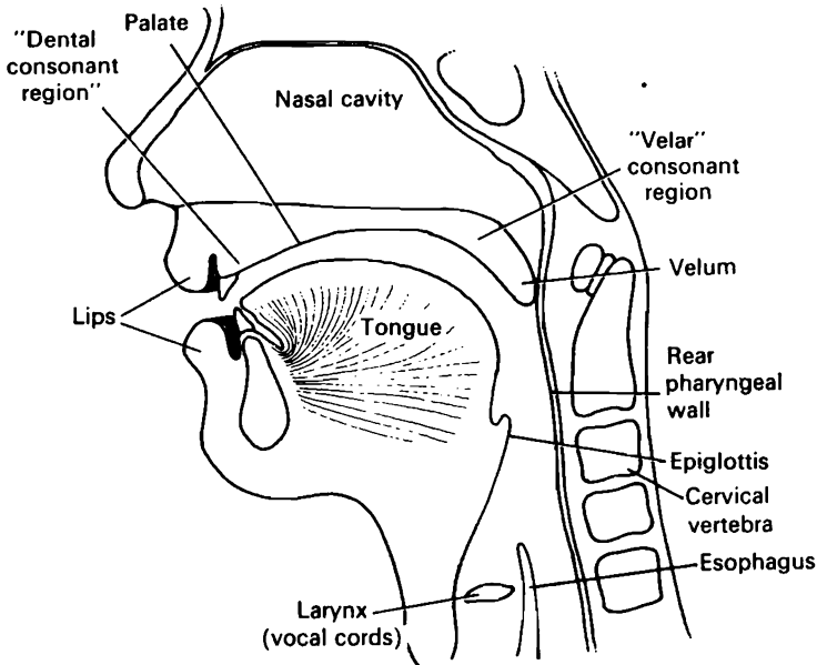
Figure 4.8. The adult human vocal tract.
