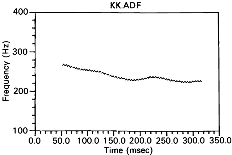
Figure 5.19. A plot of the fundamental frequency of the word dog spoken by a three-month-old child. This includes the periods marked in Figure 5.18.
