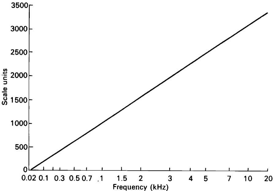
Figure 7.5. The Mel scale which relates perceived pitch to frequency. (Adapted from Fant, 1973.)
