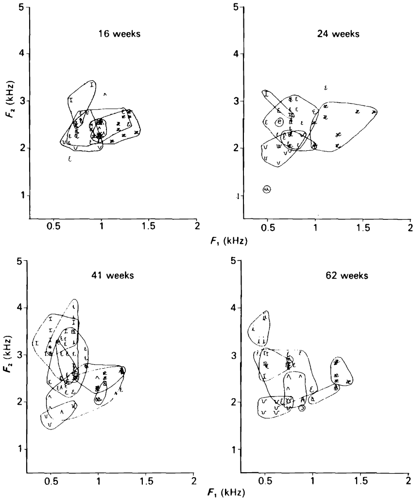
Figure 9.3. Gradual development of the formant frequency pattern for the vowels of American English in an infant from age 16 to 62 weeks.
