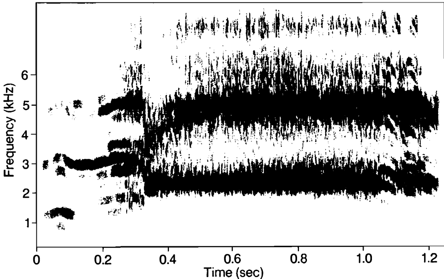
Figure 5.11. Spectrogram of breathy utterance of a newborn infant. The "noise" excitation makes it possible to resolve the formant frequencies although the fundamental frequency is very high.
