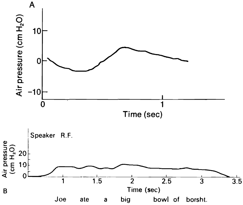
Figure 6.1. (A) Pulmonary air pressure during quiet respiration. (B) Pulmonary air pressure during speech. The speaker was instructed to emphasize the underlined word in the sentence. Note the air pressure peak.
