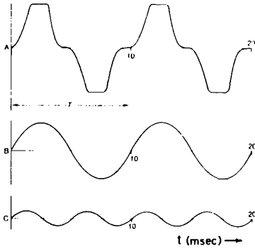
Figure 3.6. (A) A complex waveform. (B) and (C) Its first two sinusoidal Fourier components.
