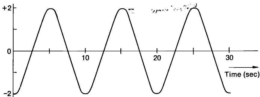
Figure 3.4. Wave of Figure 3.2 shifted in phase.
