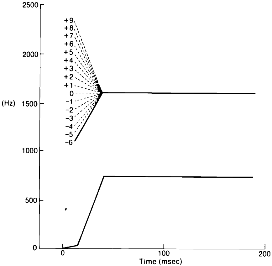
Figure 7.7. Schematic representation of two formant frequency patterns that will produce the sounds [bæ], [dæ], and [gæ]. The numbers - 6 through + 9 reference the different signals. (Adapted from Liberman, 1970b).
