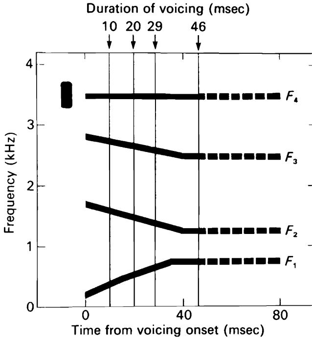
Figure 8.15. Schematized spectrographic representation of a stimulus with formant trajectories appropriate for the syllable [da]. From Blumstein and Stevens, 1980.
