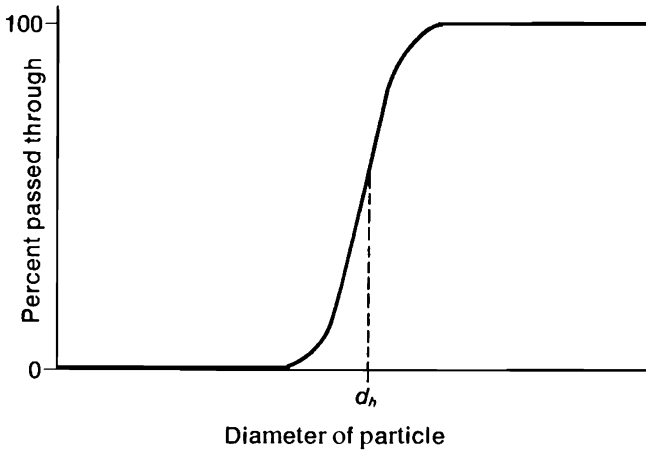
Figure 3.10. Transfer function of sieve as “large-diameter pass through” filter.
