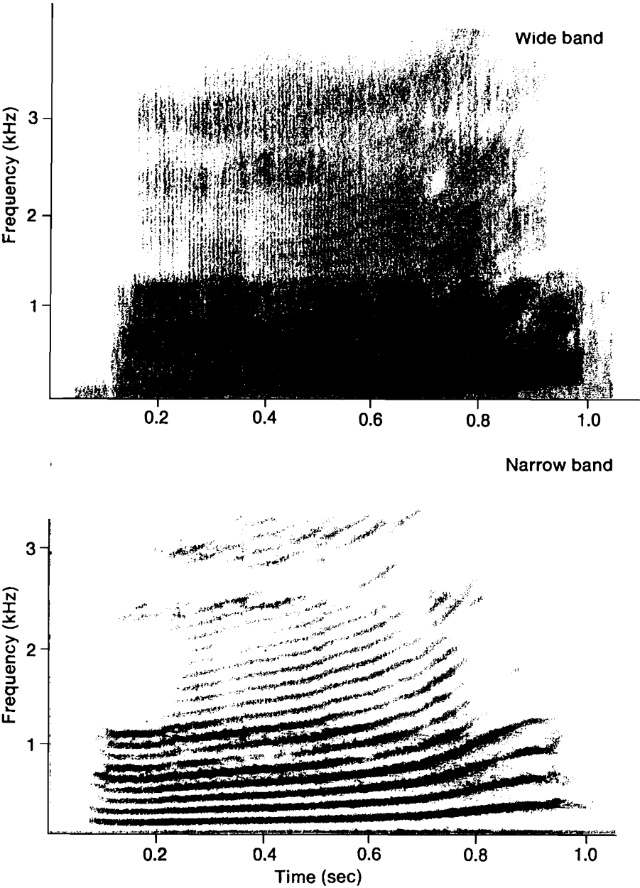
Figure 5.10. Note the “staircase” effect on the wide-band spectrogram. The fundamental frequency is at the point of being too high for the spectrograph to resolve the formant frequencies.
