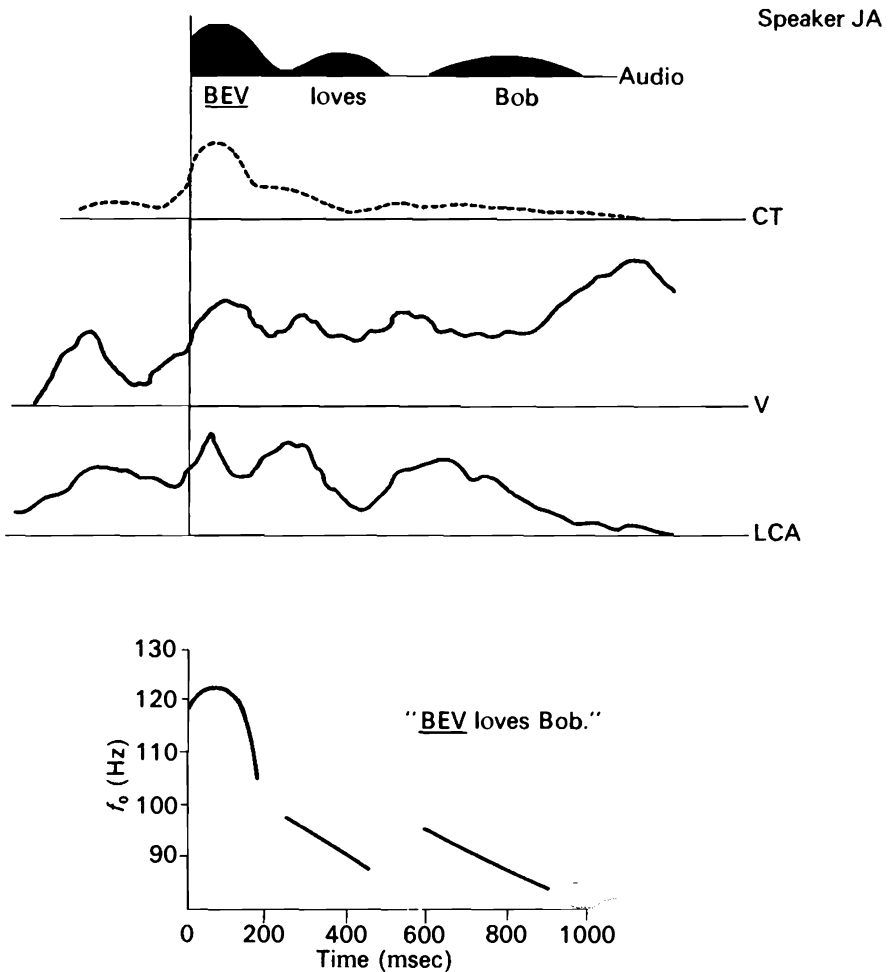
Figure 6.8. Computer-averaged and computer-integrated electromyographic signals and fundamental frequency of phonation as functions of time for 38 tokens of the sentence Bev loves Bob spoken by one speaker. The speaker stressed the word Bev . The activity of the cricothyroid muscles (CT), internal thyroarytenoid muscles (V), and lateral cricoarytenoid muscles (LCA) electrical activity are plotted. (After Atkinson, 1973.)
