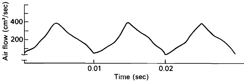
Figure 4.1. Three cycles of a waveform typical of the air flow through the glottis during phonation.
