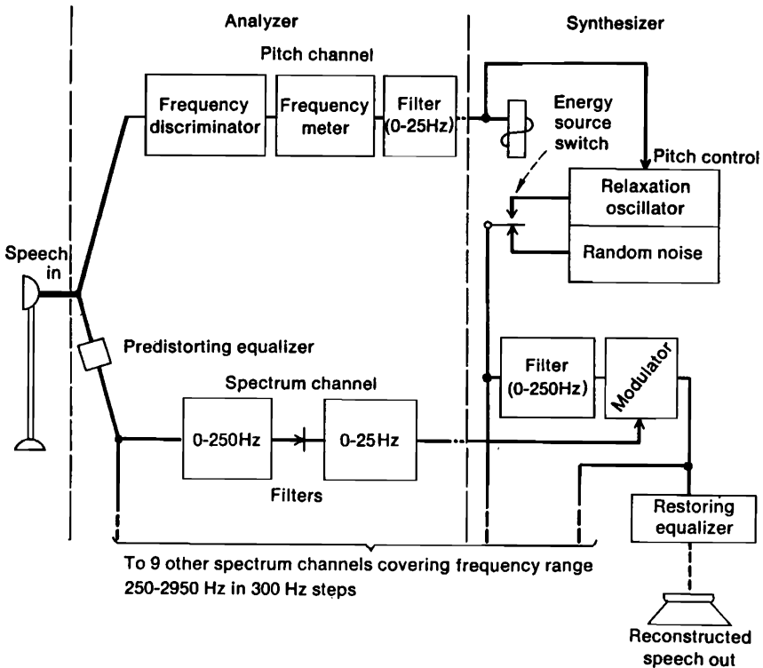
Figure 7.1. Vocoder block diagram. (After Dudley, 1936.)
