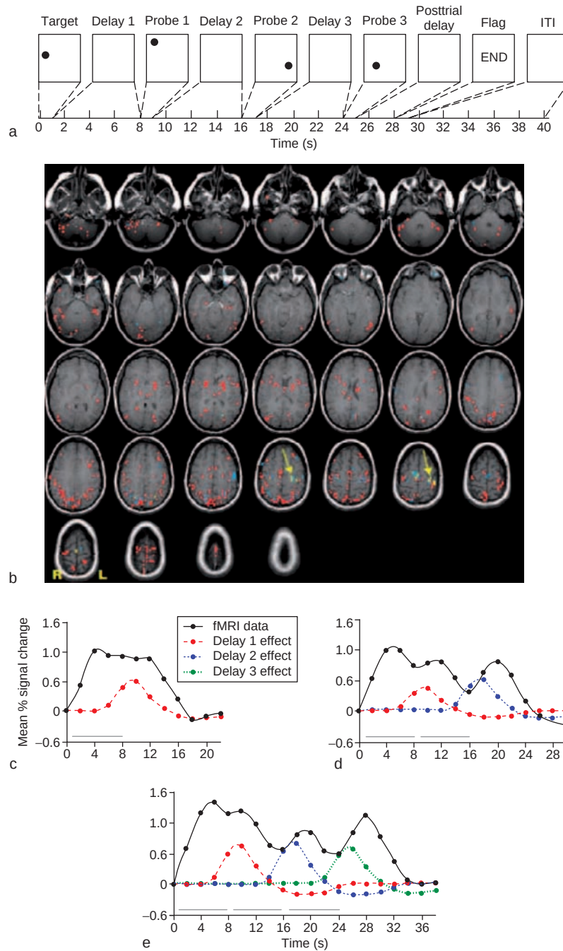
Plate 34 A functional magnetic resonance imaging experiment demonstrating sustained memory-related activity for location across multiple delay periods. (a) Behavioral task. Individuals view and encode the target location, then, after a 7 s delay, indicate with a button press whether the probe does or does not appear in the same location. One-third of the trials end after probe 1. On two- and three-delay trials, the offset of probe 1 is followed by another delay period, after which individuals evaluate the location of probe 2 with respect to the target. On one- and two-delay trials, the 'END' message appears at times 12 and 20 s, respectively. (b) Results from a single representative individual. Voxels in red showed sustained delay-period activity for delay 1 only. Voxels in blue are the subset of voxels with delay-period activity sustained across delay 1 and delay 2. Voxels in yellow are the still smaller subset with delay-period activity sustained across all three delays. Note that although many regions, including the prefrontal cortex, show delay-period activity during delay 1, only dorsal-stream parietal and frontal oculomotor regions sustain this delay-period activity across all three delays. Arrows highlight the voxels from left frontal eye field (the activity of which is shown in panels c, d, and e). (c) Activity from three-delay voxels in the left frontal eye field, averaged across one-delay trials. 'Delay 1 effect' reflects the estimated magnitude of delay 1 activity. Gray bar along the horizontal axis indicates the duration of the delay period. (d) Activity from these same frontal eye field voxels averaged across two-delay trials. Graphical conventions are the same as in panel b. (e) Activity from these same frontal eye field voxels averaged across three-delay trials. Graphical conventions are the same as in panel c. Adapted from Postle BR (2006) Distraction-spanning sustained activity during delayed recognition of locations. NeuroImage 30: 950-962. (see page 344).
