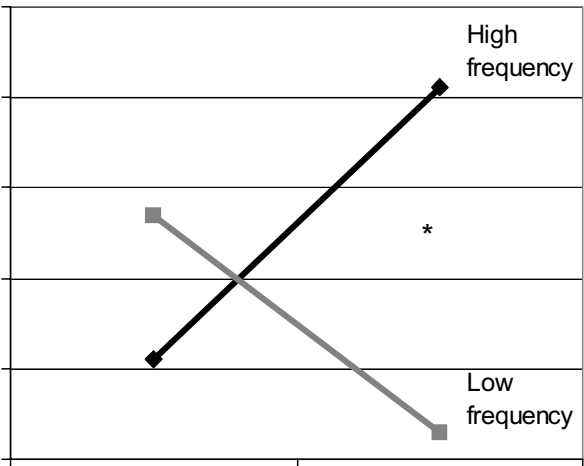
Figure 2b. High gamma band response relative to baseline for high and low-frequency words in the first-time window (0-256 ms), * = p < .01 .
