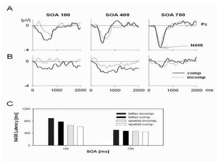
Figure 4. Difference Waves between Event-related Potentials Elicited by Non-synonymous and Synonymous Target Words (N400 component). This figure shows the difference waves in two dual task experiments as a function of stimulus onset asynchrony (SOA) with a letter (L or R) that had to be responded to with compatible or incompatible (comp vs. incomp) left and right pedal presses. Panels A and B show the N400 component when words had to be judged for meaning (synonymity) and for acoustic properties (voice pitch), respectively. When nouns were judged for meaning, task load delayed the N400 component (see panel A, SOA 100 incompatible). N400 was abolished when nouns had to be processed for acoustic properties under task load (see panel B, SOA 100 incompatible). The abscissae show the first 2 seconds after the onset of the spoken target word. The ordinates show the voltage of the brain's response to those words (in microvolt). Panel C. Latency of N400 Maximum as a Function of SOA: depending on whether the additional task stimulus was a letter (language-related) or a spatial location of a small square (spatial), as well as of the compatibility of response assignment to this stimulus (comp. vs. incomp.). Due to task overlap the peak latency of the N400 is more strongly delayed when letters had to be processed in an additional task than when squares had to be processed.
