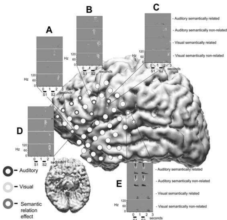
Figure 2. Left and bottom view of a subject brain image (co-registration of pre-operative 3D-MRI and post-implantation CT scan). Electrodes are shown as white disks. Red circles denote sites with differential high gamma activity (HGA, >70 Hz) between semantically related pairs and non-related pairs. Blue and yellow circles denote HGA to auditory or visual stimuli respectively. Representative time-frequency plots A-E are presented. Sites A-D show an effect of semantic relatedness. Non-related word pairs are associated with greater HGA compared with semantically related stimuli, most apparent at late latencies. The latencies of HGA responses to visual stimuli are typically longer than those to auditory stimuli. Site E shows HGA responses and event-related desynchronization at lower (alpha/beta) frequencies almost exclusively during presentation of auditory (spoken) stimuli, with no difference based upon semantic relatedness. Note that the only site with responses confined to visual stimuli was located over occipital-temporal cortex.
